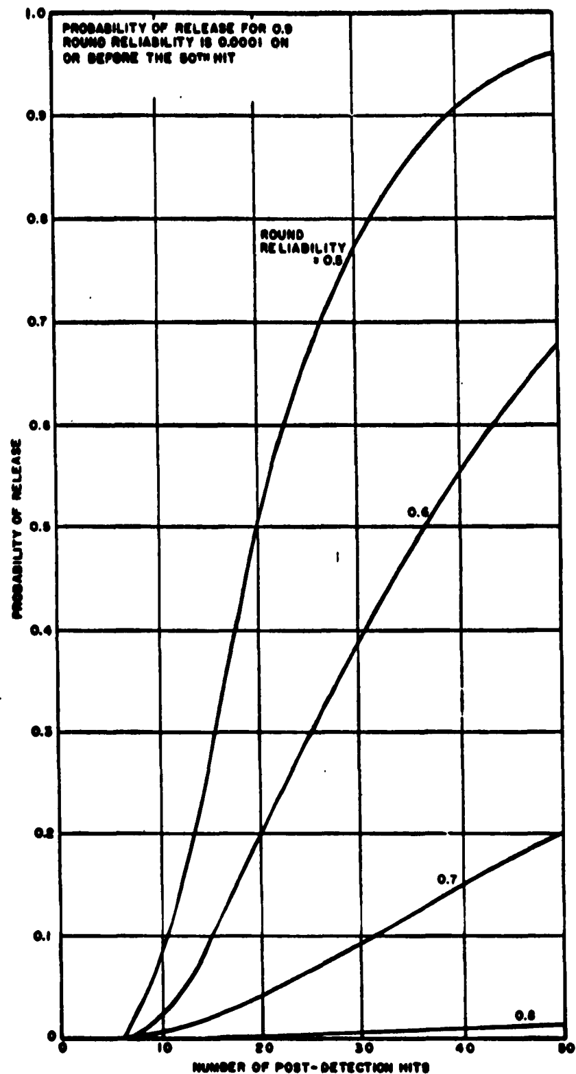
FIGURE 2. PROBABILITY OF RELEASE OF A MILITARY AIRCRAFT AS A FUNCTION OF THE NUMBER OF POST-DETECTION HITS AND ROUND RELIABILITY
