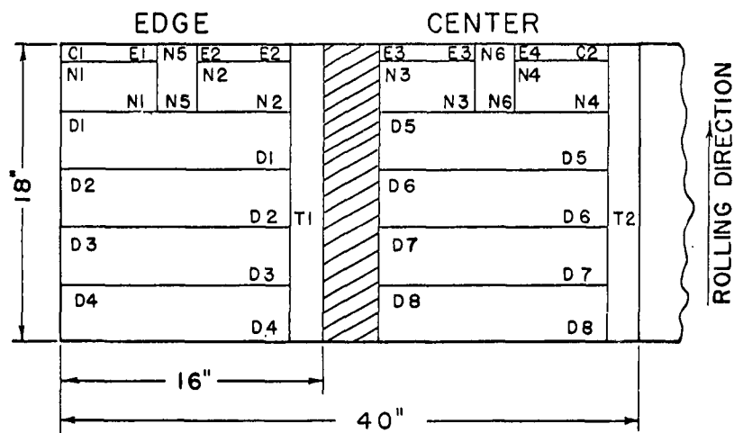
FIG. 1. COMPLETE SPECIMEN BLANK LAYOUT.
