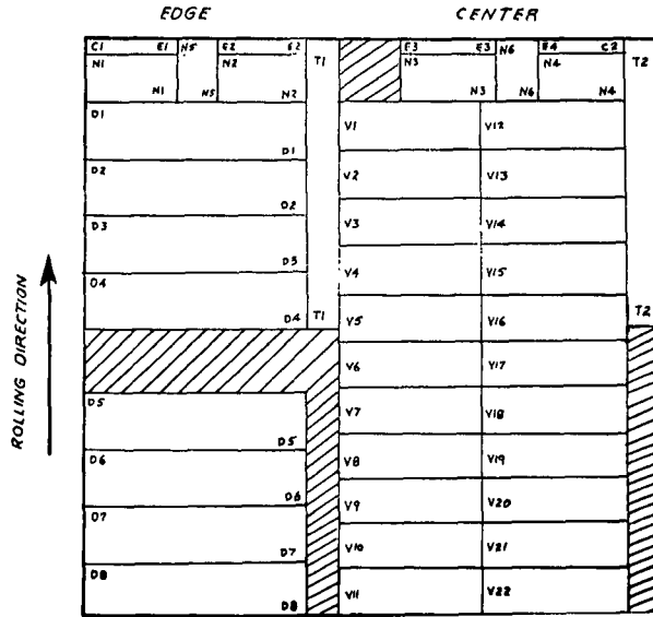
SPECIMEN BLANK LAYOUT FOR PROJECT SR-139
