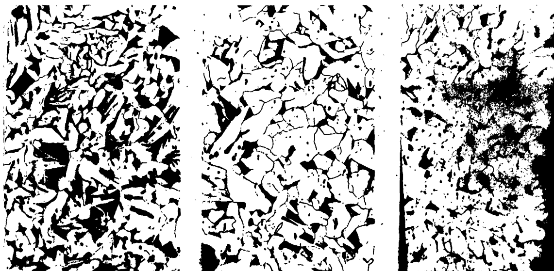
a) Area near plate surface. X 250
