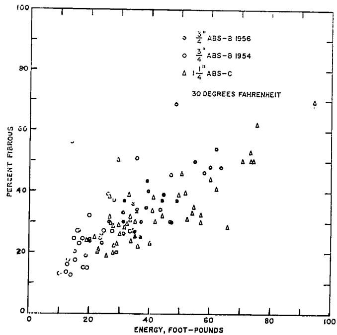
FIG. 18. CORRELATION OF CHARPY V-ENERGY ABSORPTION AND CHARPY V-FRACTURE APPEARANCE AT 30 F.
