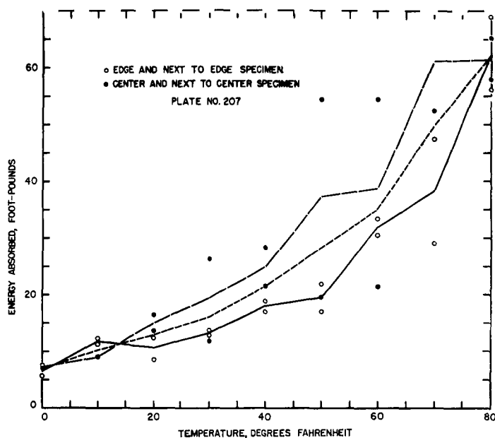
FIG. 19. INFLUENCE OF SPECIMEN LOCATION IN PLATE NO. 207 ON CHARPY V-ENERGY ABSORPTION.
