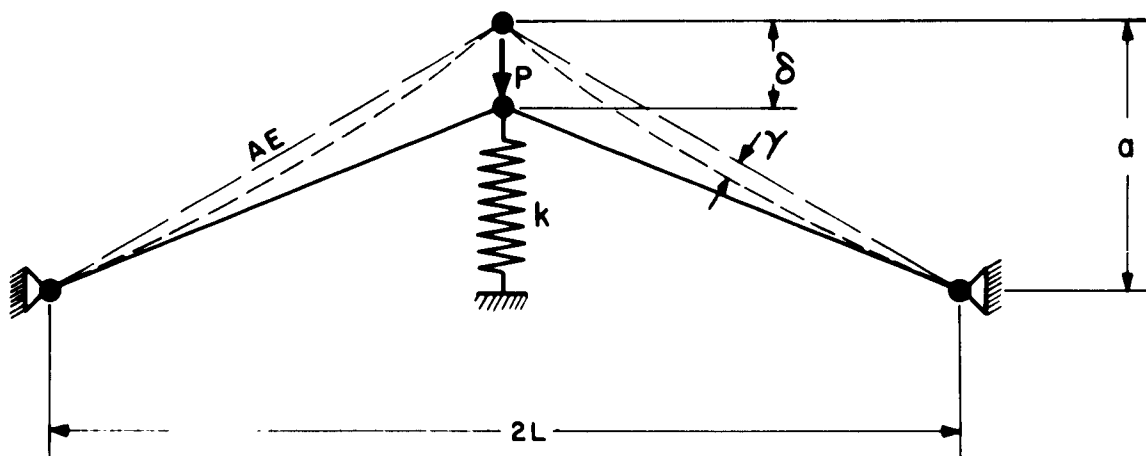
FIG. 2 MODEL TO EXHIBIT SNAP BUCKLING.
