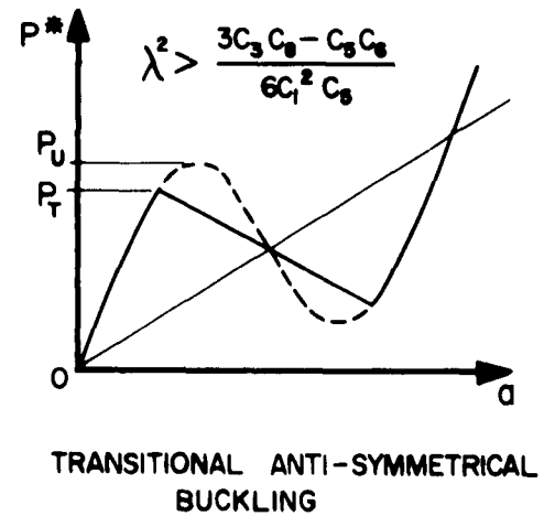
FIG. 12 VARIATION OF BUCKLING MODES WITH \lambda ( \lambda = \frac{\beta^2 R}{\uparrow} )
