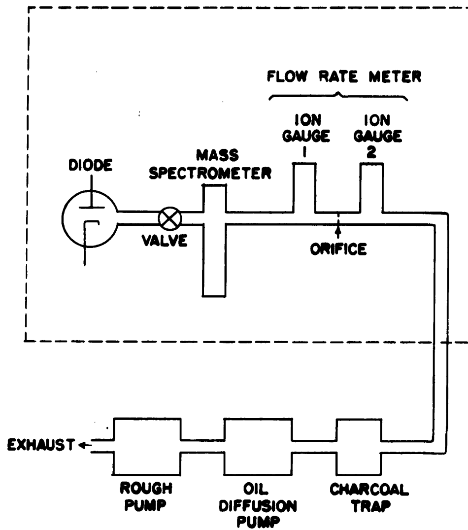
Figure 1. Vacuum System.
