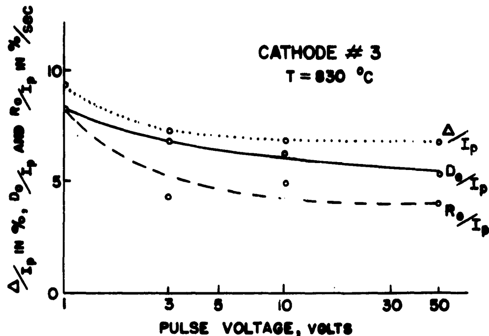
Figure 16. Dependence of Effect of Ion Bombardment by Oxygen on Pulse Voltage.
