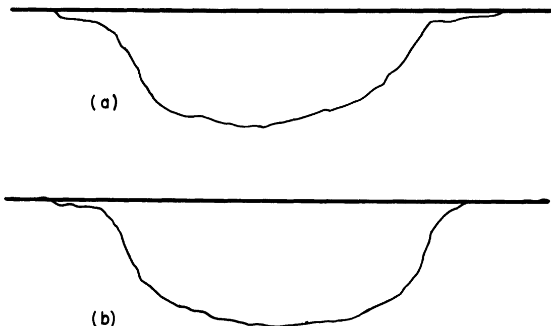
Figure 2-8. Electron Beam Profiles: (a) Cathode Poisoned by Oil from Diffusion Pump. (Ball valve accidentally left open over night.) (b) Cathode without Poisoning.
