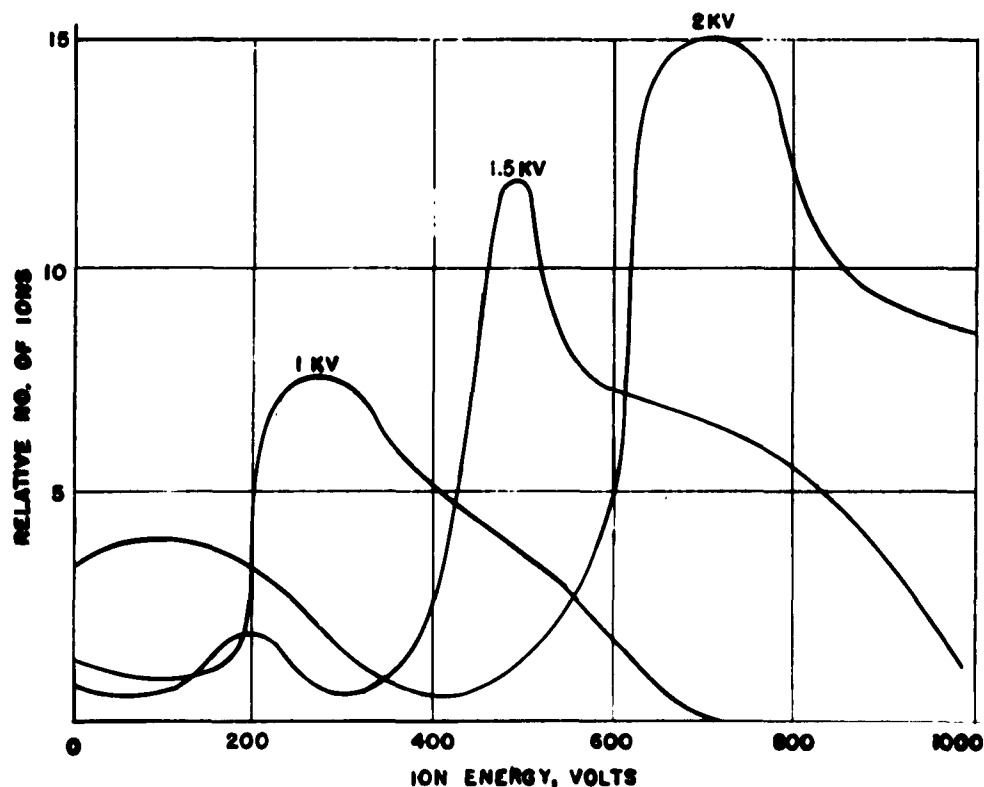
Figure A-5. Energy Distribution of Ions Extracted from Cold Discharge.
