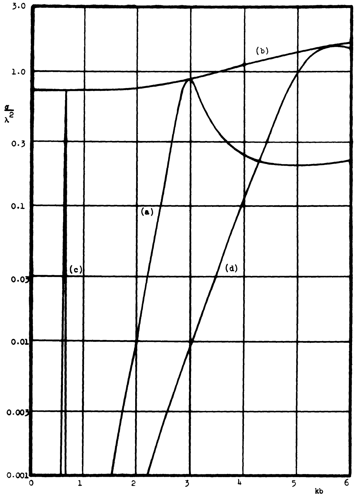
Figure 4. Echo area of (a) unloaded dipole, (b) resonant dipole, (c) dipole resonated by fixed L, and (d) open-circuited dipole. b/a = 150 .
