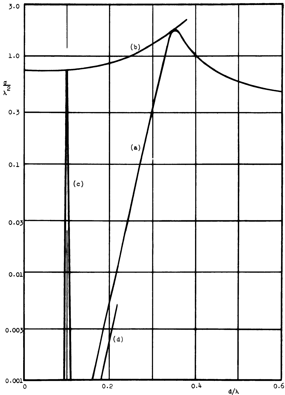
Figure 6. Echo areas of (a) unloaded loop, (b) resonant loop, (c) loop resonated by fixed C, and (d) open-circuited loop. d/a = 200 .
