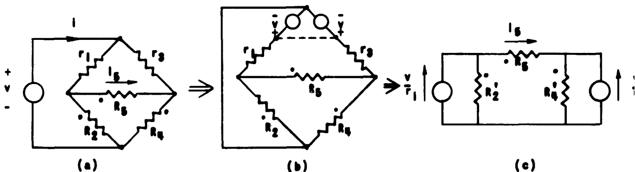
FIG. 39. A BRIDGE WITH THREE FWL RESISTORS.
