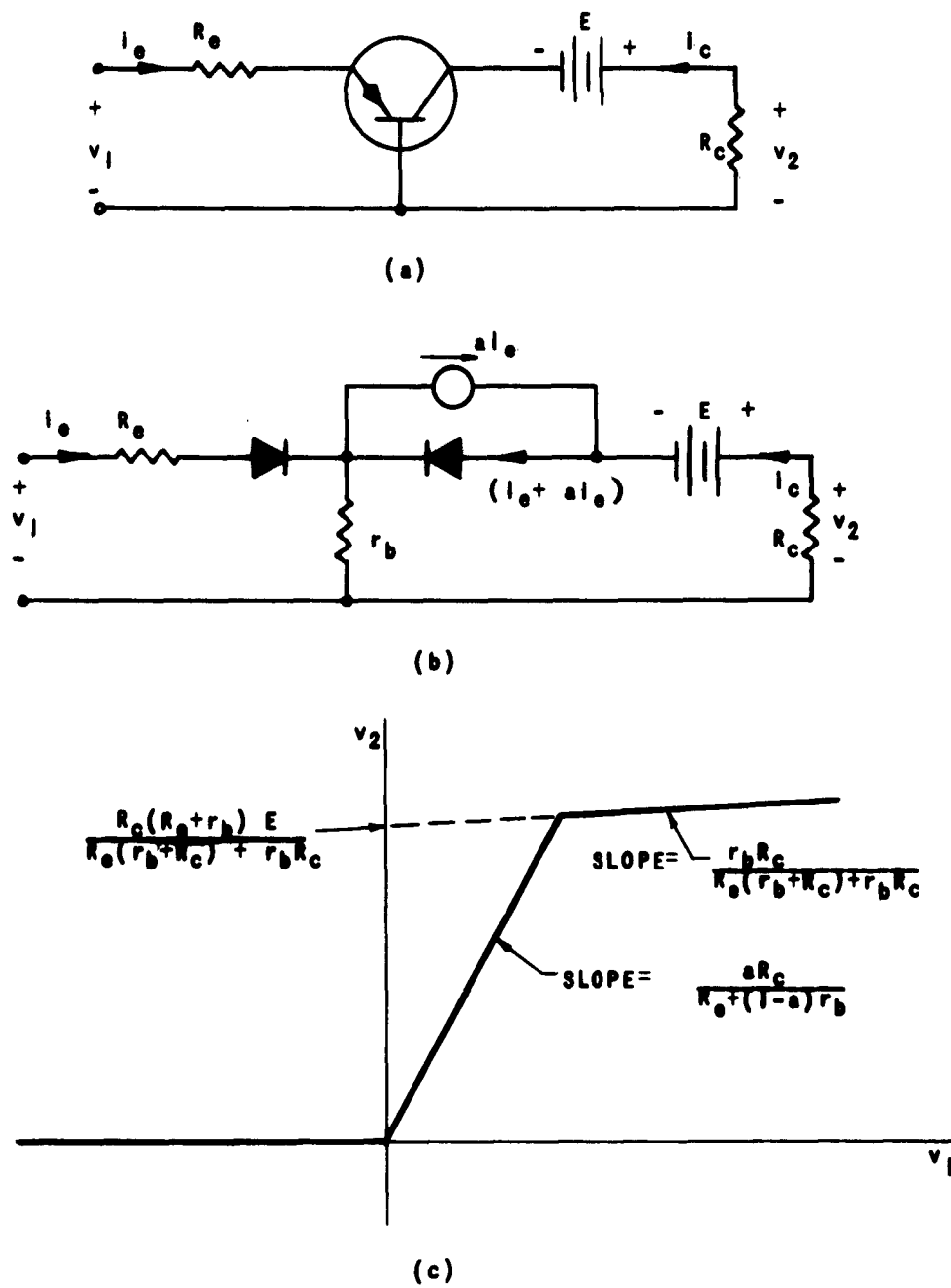
FIG. 54. GROUNDED-BASE TRANSISTOR AMPLIFIER AND TRANSFER CURVE.
