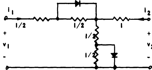
FIG. 47. PWL T-NETWORK WITH TWO PWL RESISTORS.
