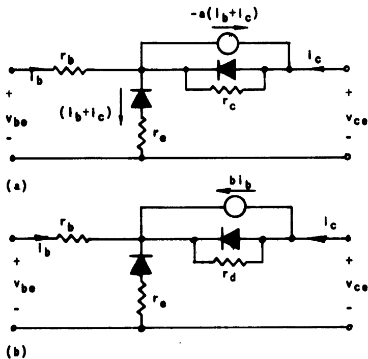
FIG. 52. PWL MODELS FOR GROUNDED-EMITTER TRANSISTOR.
