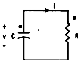
FIG. 56. PARALLEL R-C PWL NETWORK.
