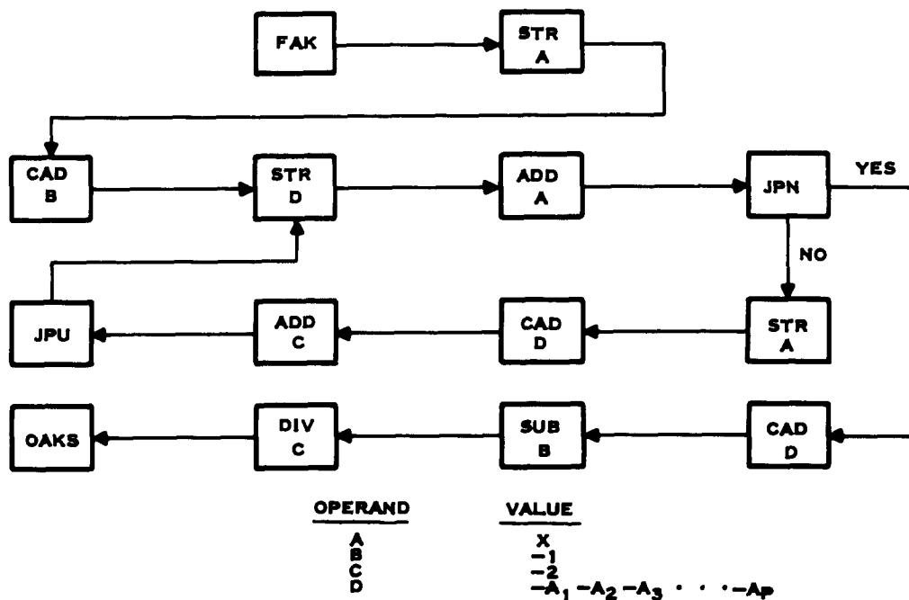
Square-Root Flow Diagram Figure 47
