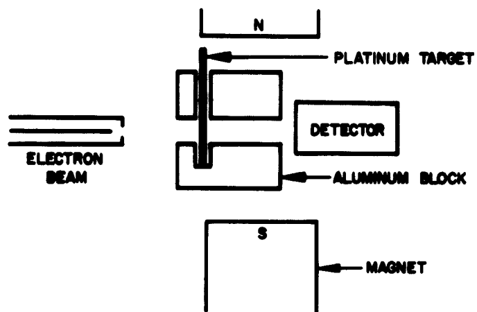
Fig. 19. Geometry used for the radiation of p-n junction detectors in an electron accelerator beam.
