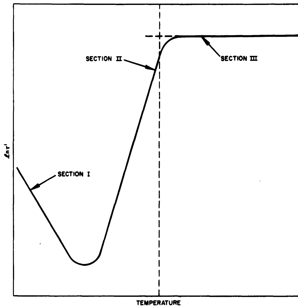
Fig. 65. Theoretical temperature dependence of the relaxation time constant.
