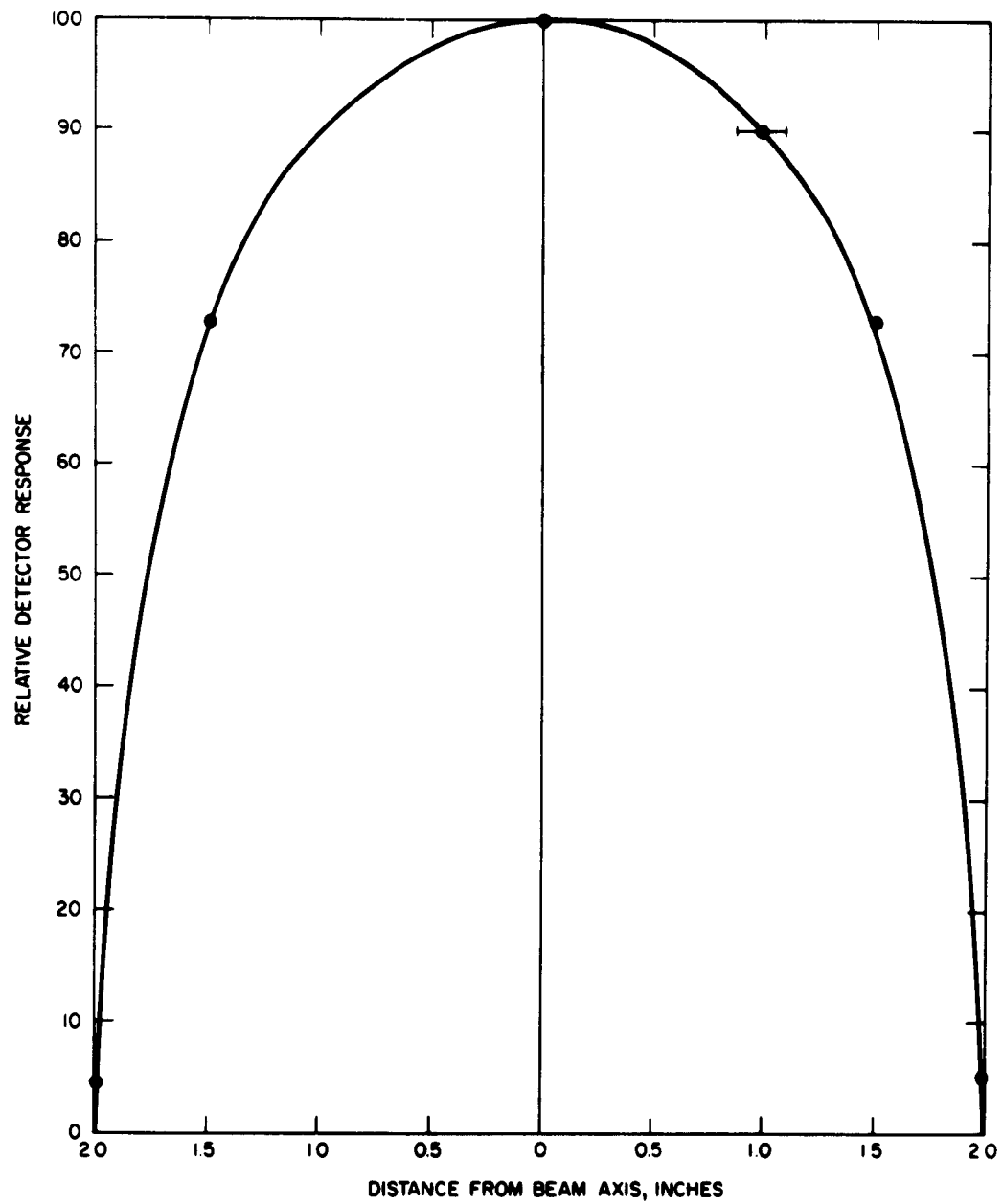
Fig. 7. The feasibility of using p-n junction radiation detectors for plotting beam profiles is illustrated by these data showing relative detector response as a function of distance from the axes of an x-ray beam.
