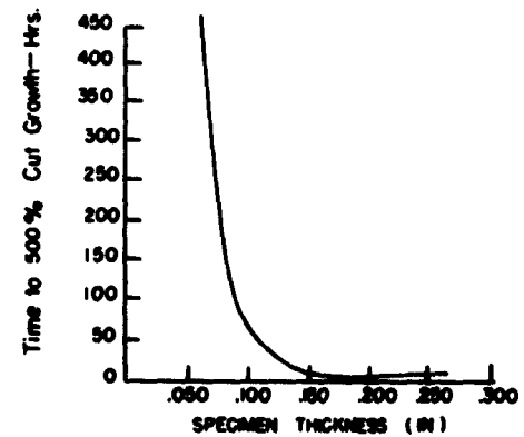
Flexing Resilience of Shore A 90
