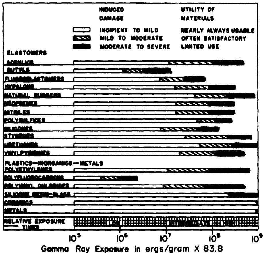
Relative radiation resistance of elastomers and other materials
