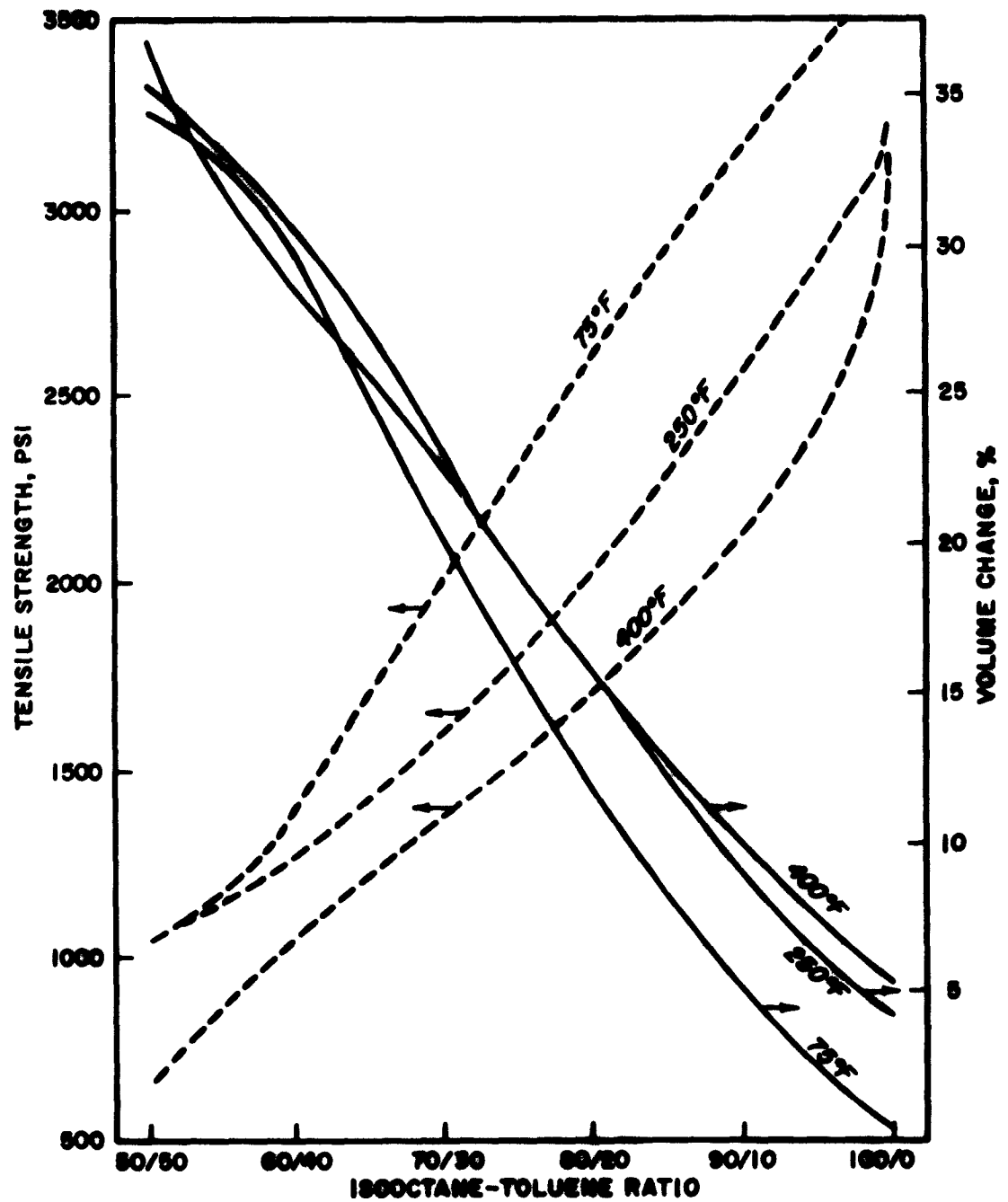
FIGURE 3-2 (3.2.2). EFFECT OF FUEL AROMATICITY ON BUNA N AT 75°F, 250°F, AND 400°F (REF. 11)
