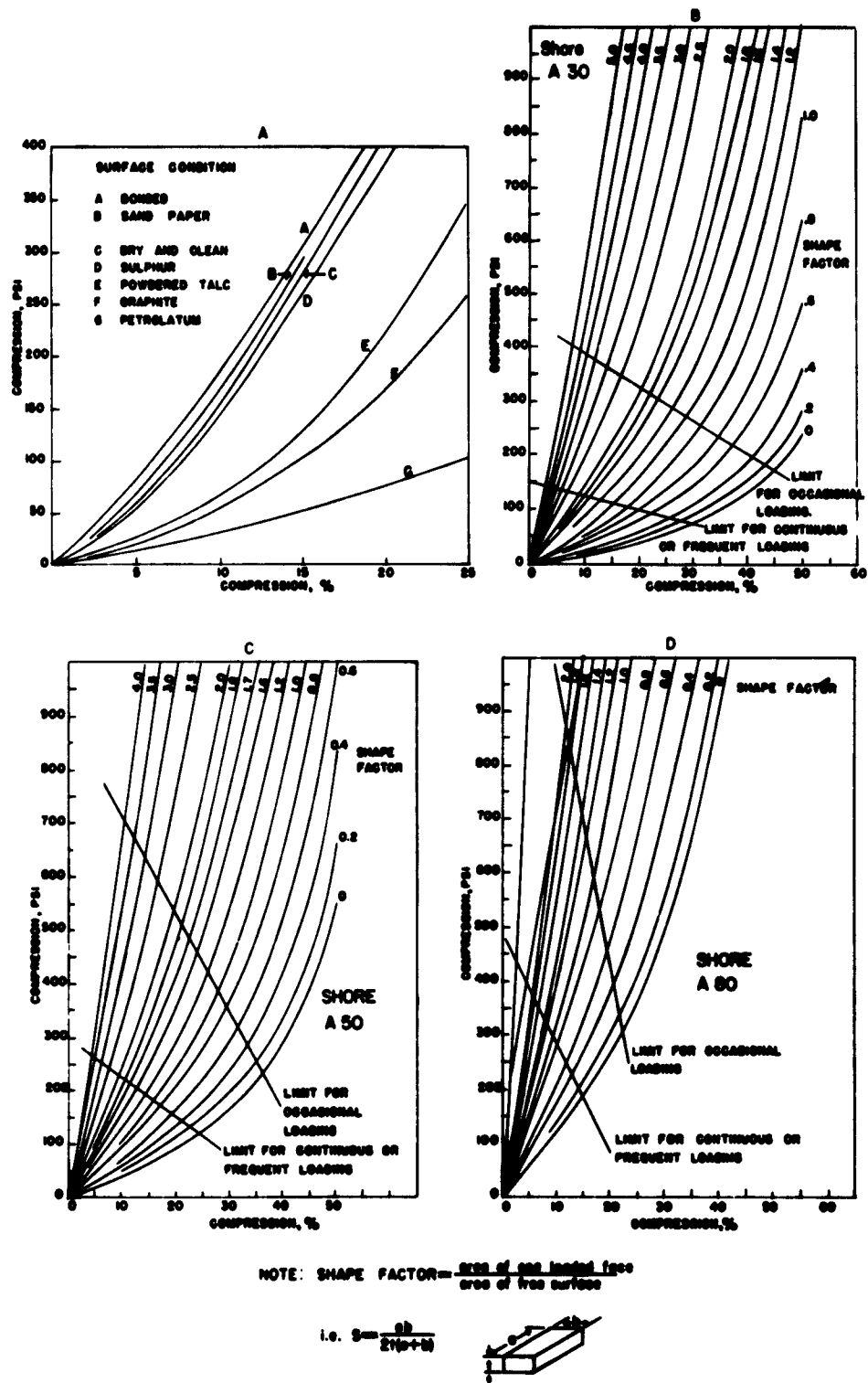
FIGURE 2-14 (2.2.1). EFFECT OF SURFACE CONDITIONS ON THE DEFLECTION OF RUBBER IN COMPRESSION AND COMPRESSION STRESS-STRAIN CURVES FOR 30, 50 AND 80 DUROMETER SPECIMENS (REF. 152)
