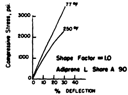
Compression-Deflection Curves
