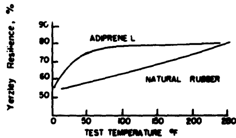
Resilience Temperature Curve for Shore A 60 Materials.
