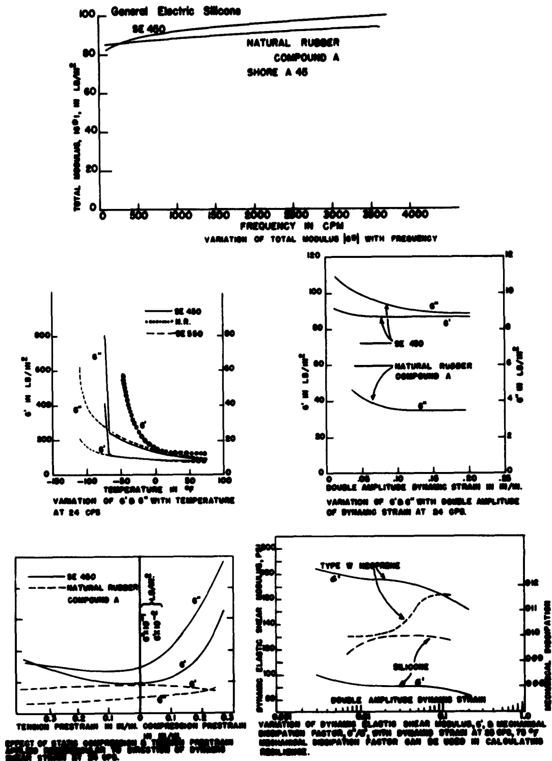
FIGURE 2-27 (2.2.2). G' AND G'' VALUES (REF. 175)
