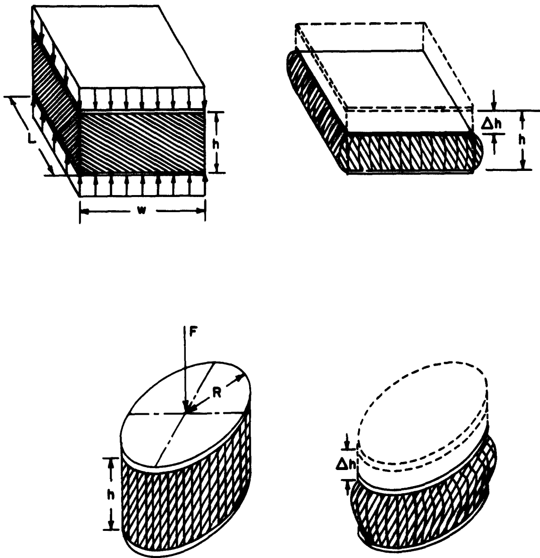
FIGURE 2-13 (2.2.1). BONDED SANDWICH UNITS LOADED IN COMPRESSION (SwRI)
