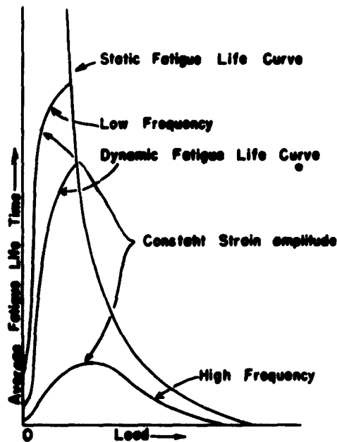
Superposition of Static Fatigue Life Curve
