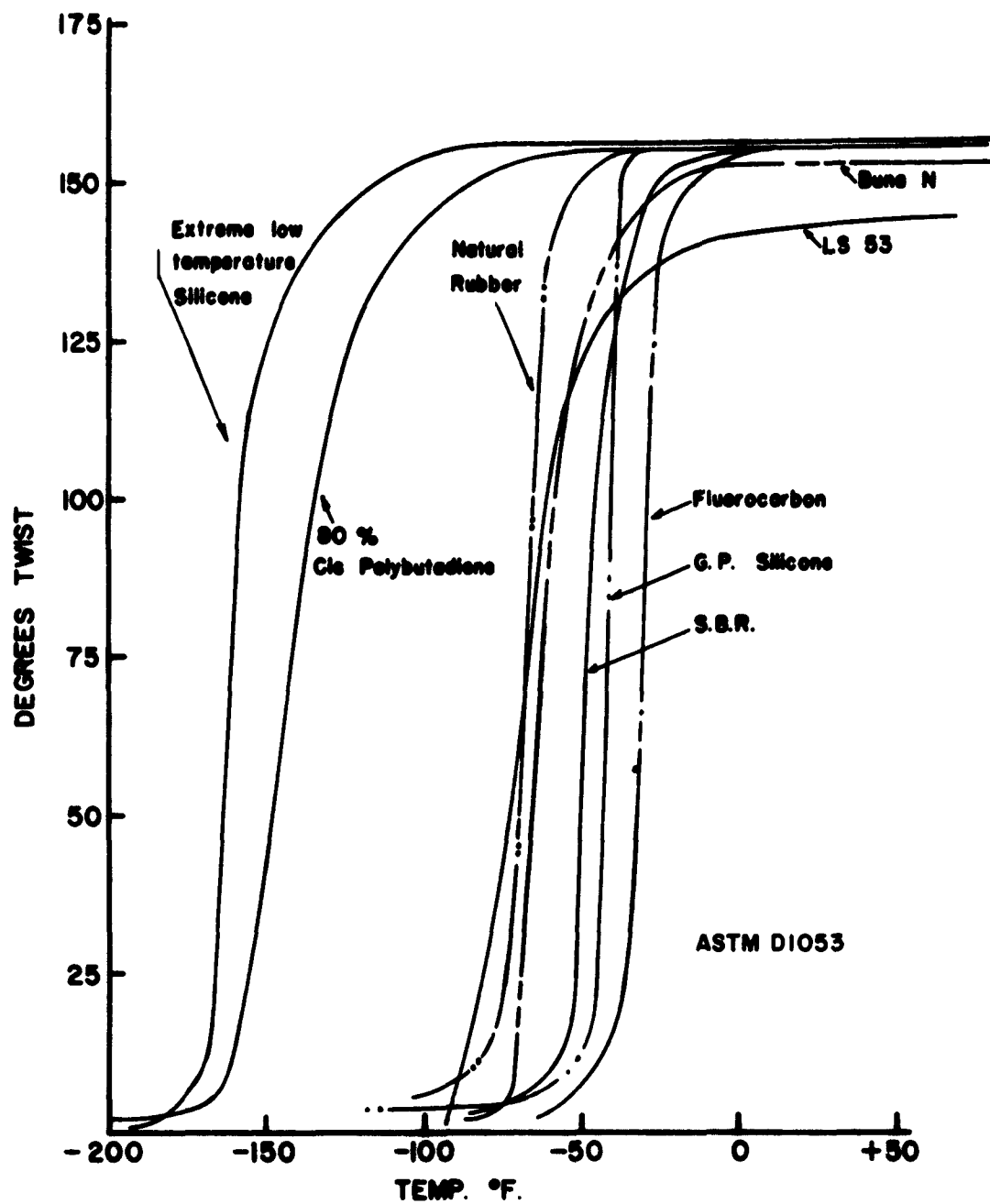
FIGURE 2-31 (2.3.2.1). STIFFENING OF ELASTOMERS AT LOW TEMPERATURES (SwRI)
