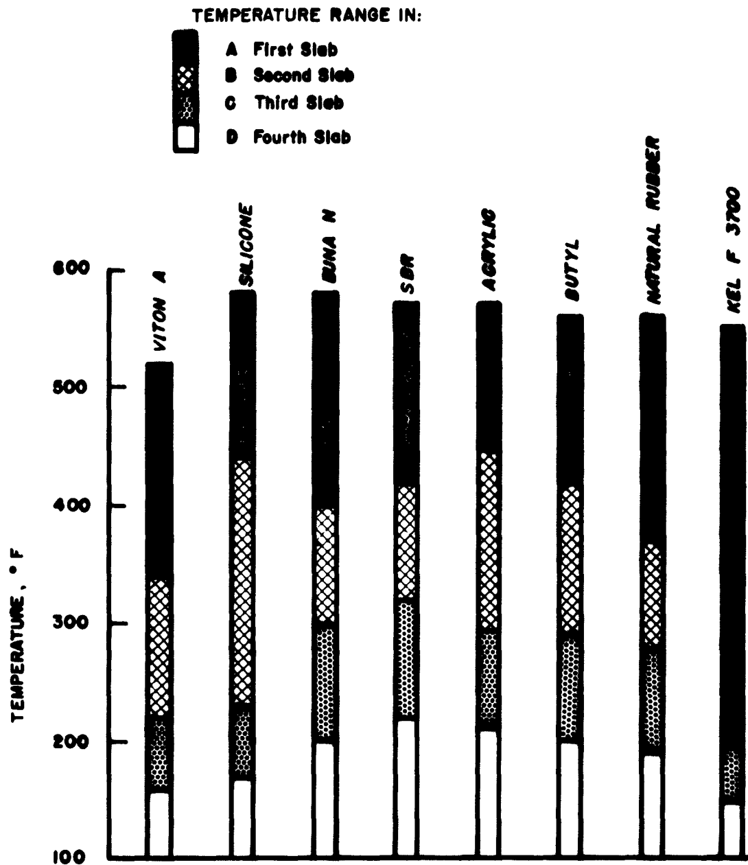
FIGURE 4-2 (4.3.1). TEMPERATURE DISTRIBUTION IN PAD OF 0.075-IN. RUBBER SLABS AFTER 3-MINUTE CONTACT WITH 800°F METAL SURFACE (REF. 134)
