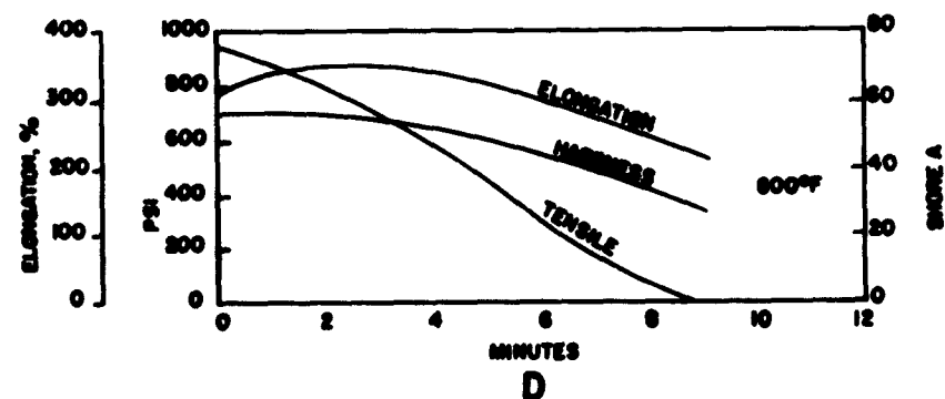
FIGURE 2-45 (2.3.2.2). TEMPERATURE EFFECTS ON SILICONES (REF. 46)
