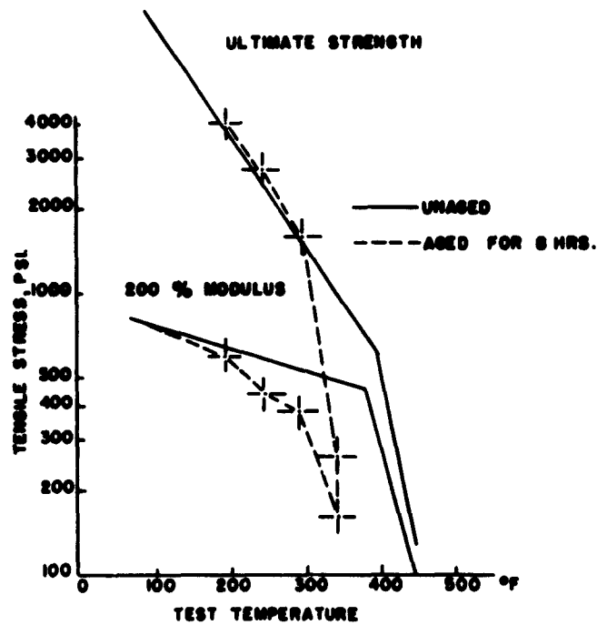
FIGURE 2-34 (2.3.2.2). EXAMPLES OF THE EFFECTS OF EXPOSURE TO ELEVATED TEMPERATURE OF A PLASTIC AND AN ELASTOMER (SwRI)
