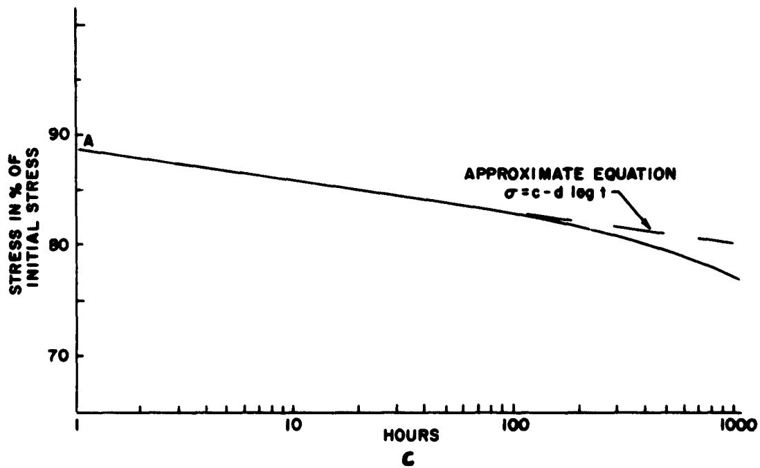
FIGURE 2-19 (2.2.1). TYPICAL STRESS RELAXATION AND RECOVERY CURVES (SwRI)
