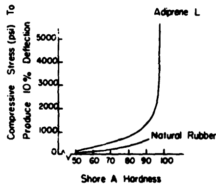
R.T. Deflection-Hardness Curves
