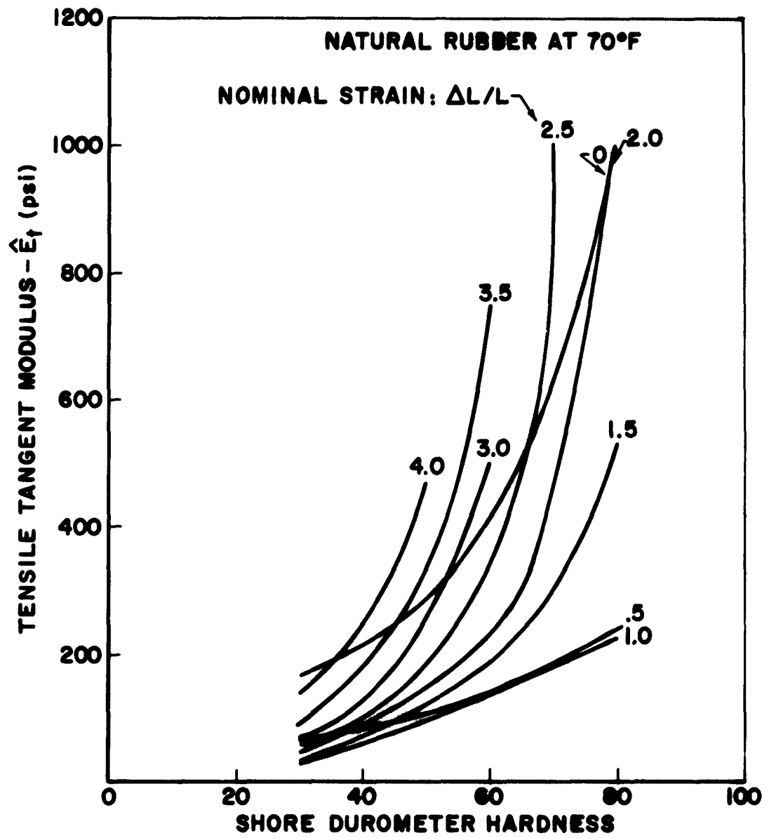
FIGURE 2-7 (2.2.1). TANGENT MODULI VALUES DERIVED FROM FIGURE 2-3 (SwRI)
