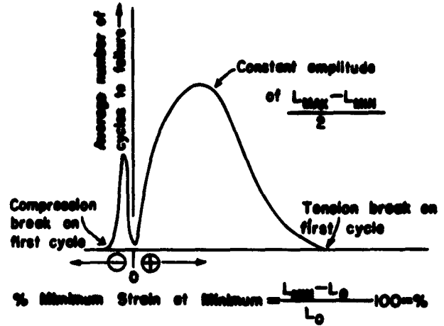
Typical Dynamic Fatigue Life Curve at Constant Temperature
