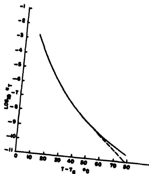
TEMPERATURE REDUCTION FACTORS FOR HYPALON-20 REDUCED TO -24.3^\circ\text{C}
