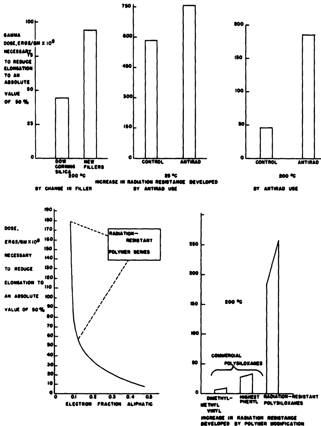
FIGURE 3-6 (3.4). VARIATION OF RADIATION RESISTANCE OF SILICONES (SHOWING THE EFFECTS OF COMPOUNDING VARIABLES AND HIGH POLYMER MODIFICATION) (REF. 91)
