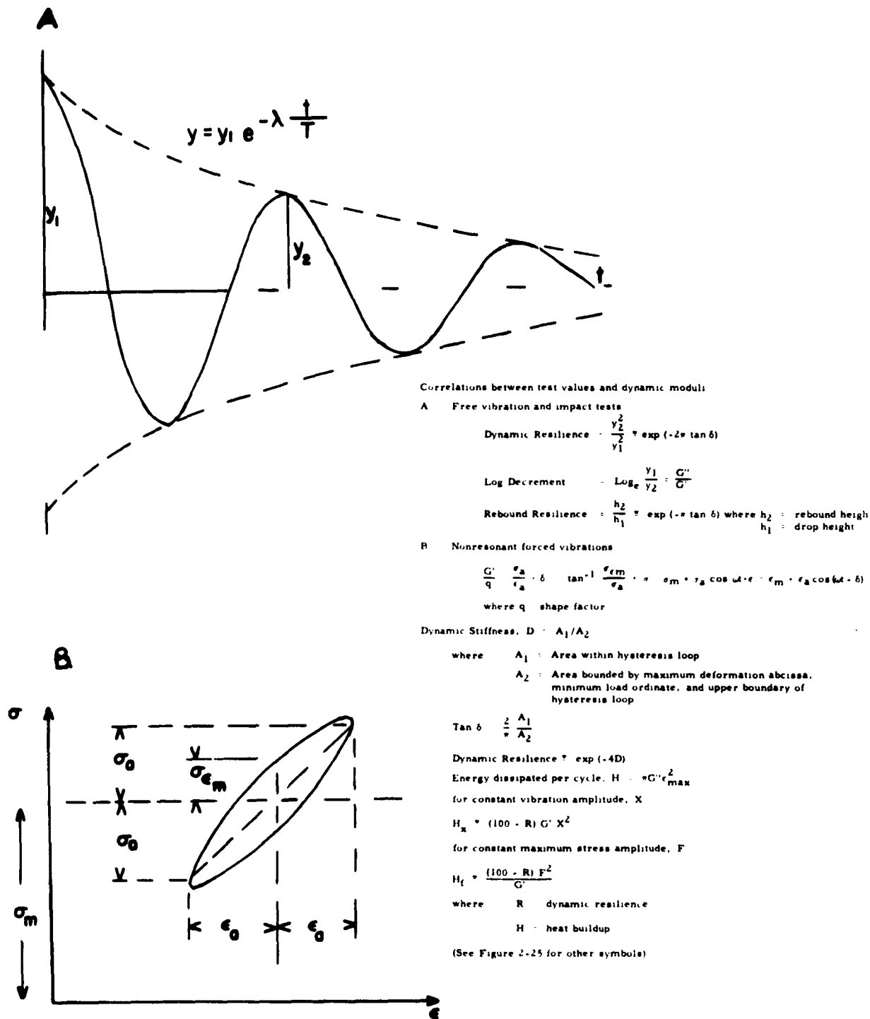
FIGURE 2-26 (2.2.2). CORRELATIONS BETWEEN TEST VALUES AND DYNAMIC MODULI (SwRI AND REFS. 100, 178)
