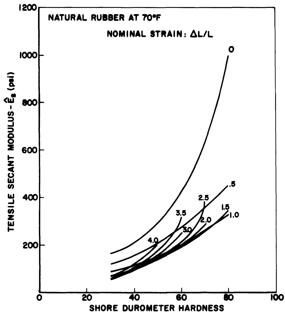
FIGURE 2-5 (2.2.1). SECANT MODULI VALUES DERIVED FROM FIGURE 2-3 (SwRI)
