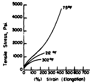
Elevated Temperature Stress-Strain Curves for Shore A 90
