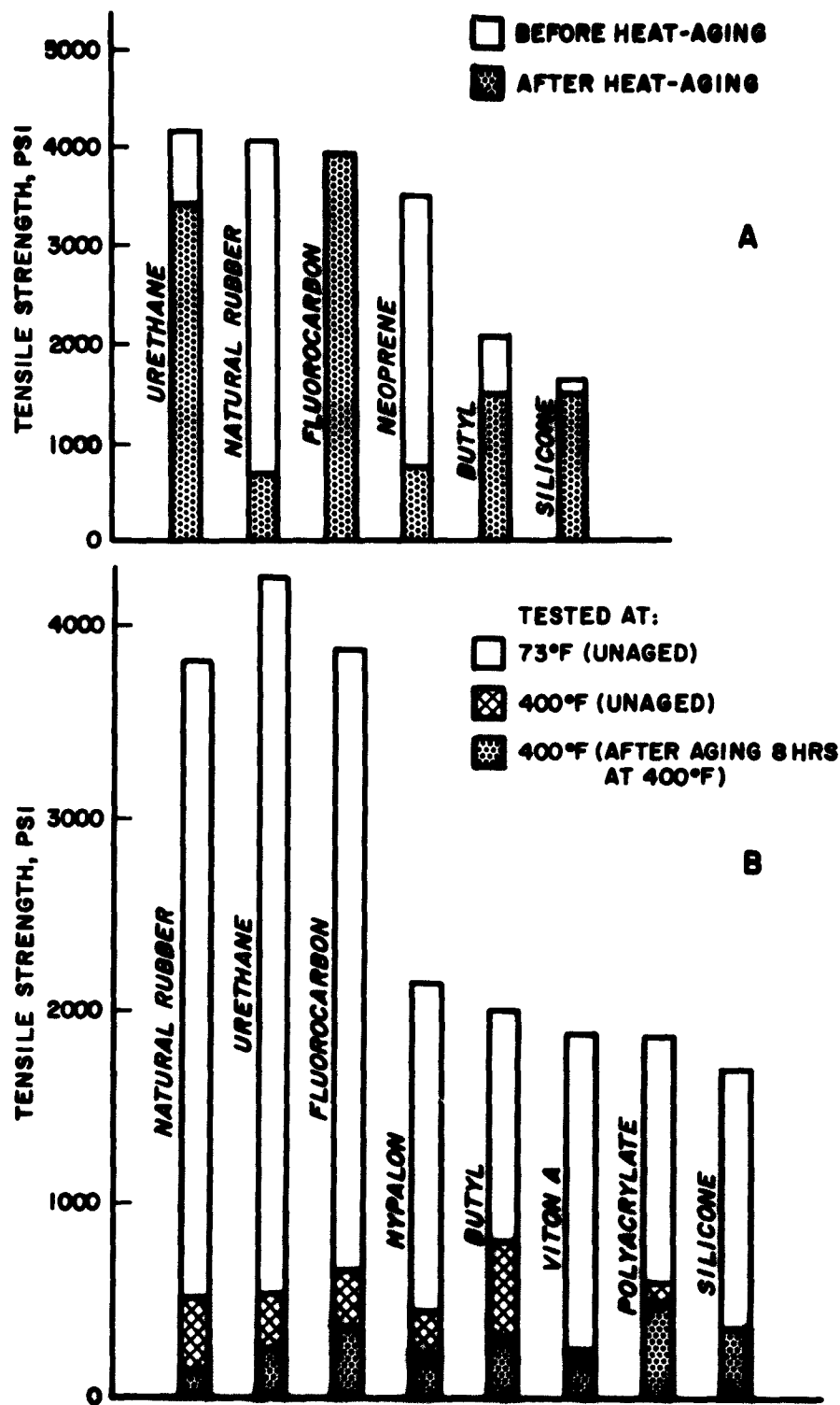
FIGURE 2-47 (2. 3. 2. 2)
