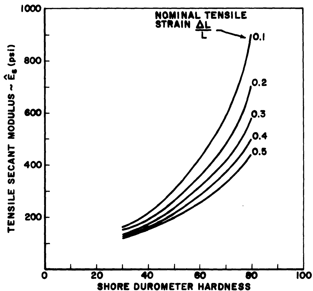
FIGURE 2-6 (2.2.1). SECANT MODULI VALUES DERIVED FROM FIGURE 2-4 (SwRI)
