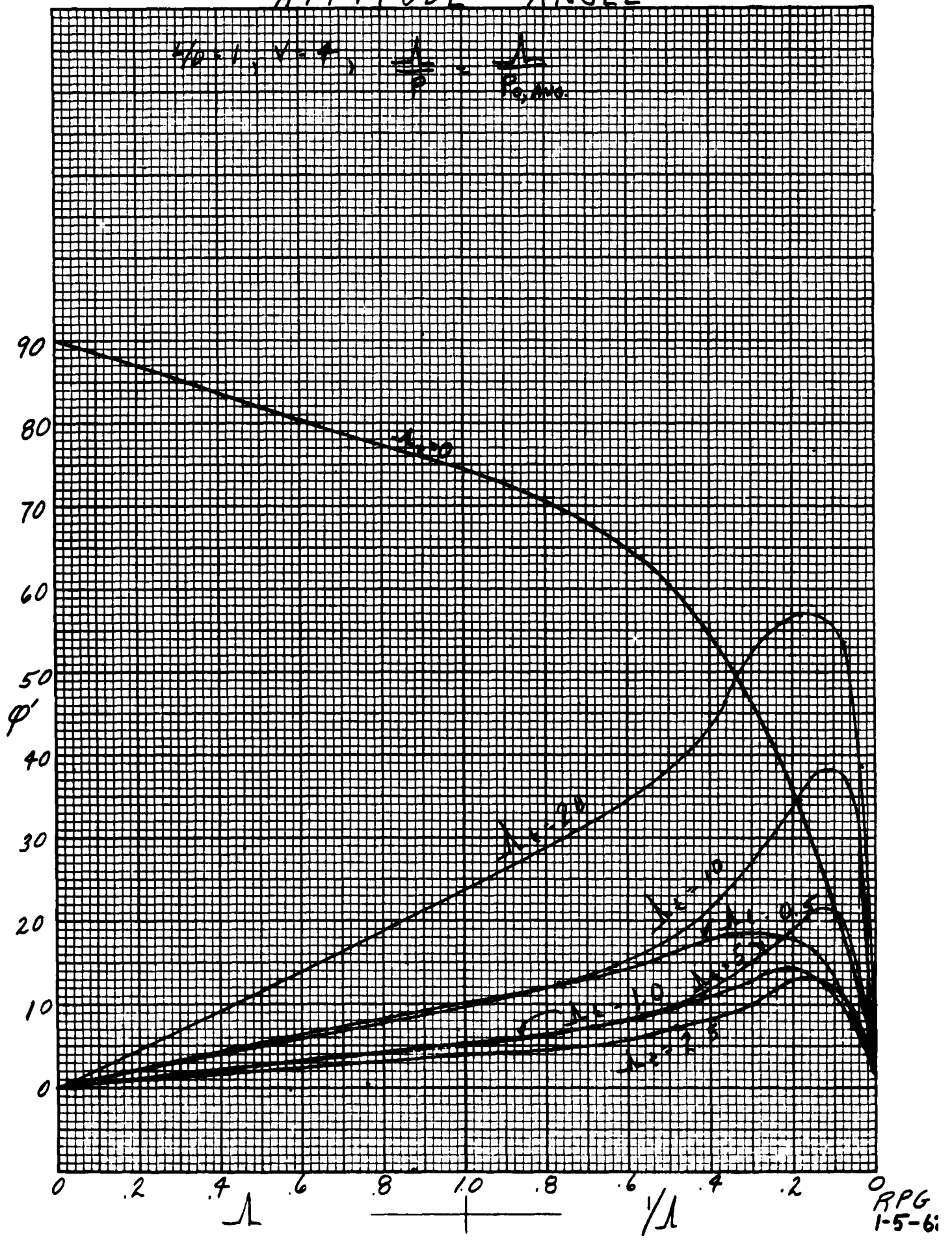
FIG. 8 ATTITUDE ANGLE
