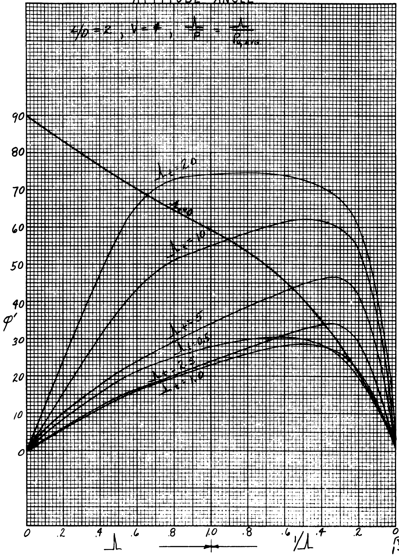
FIG. 11 ATTITUDE ANGLE
