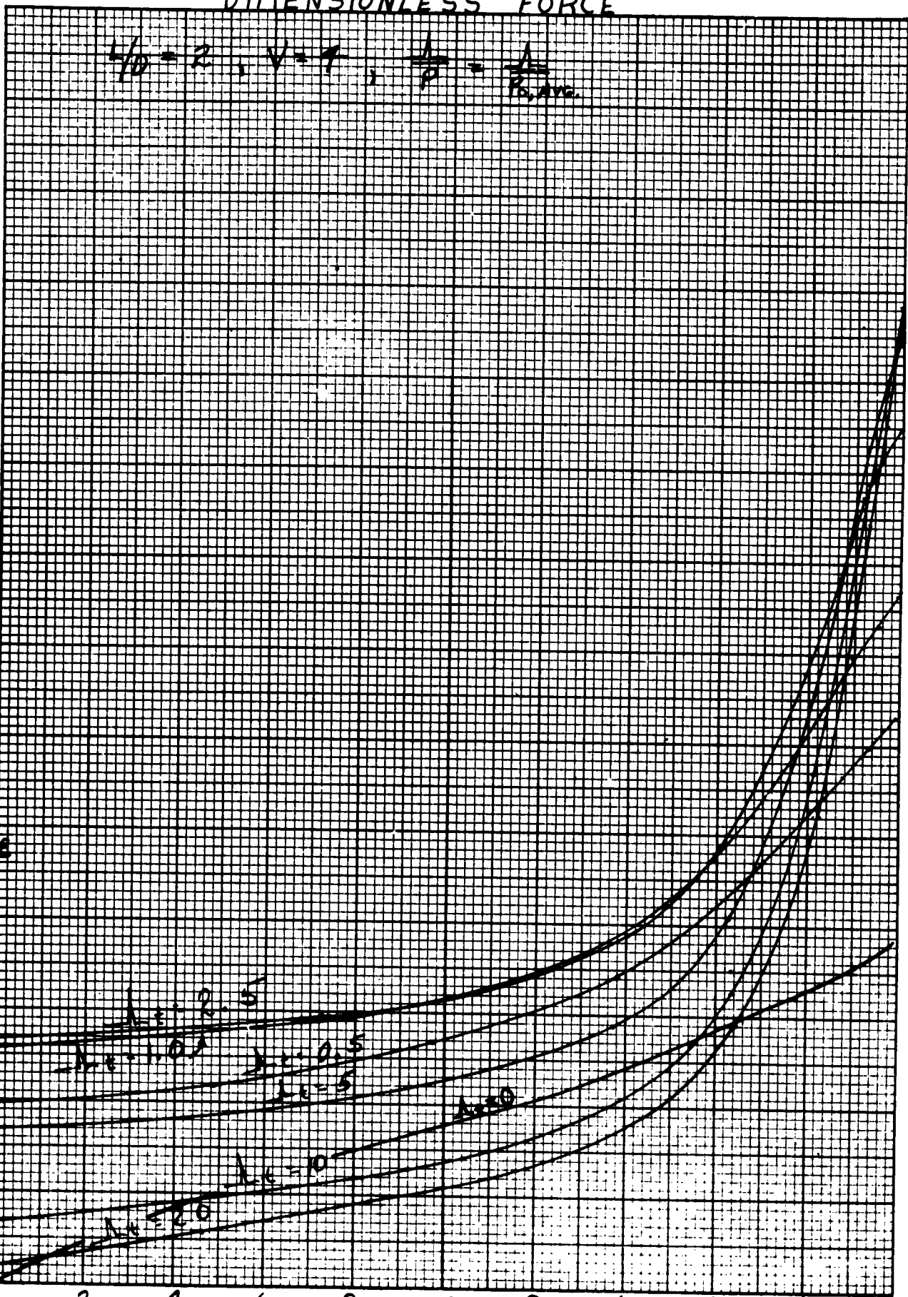
FIG. 5 DIMENSIONLESS FORCE
