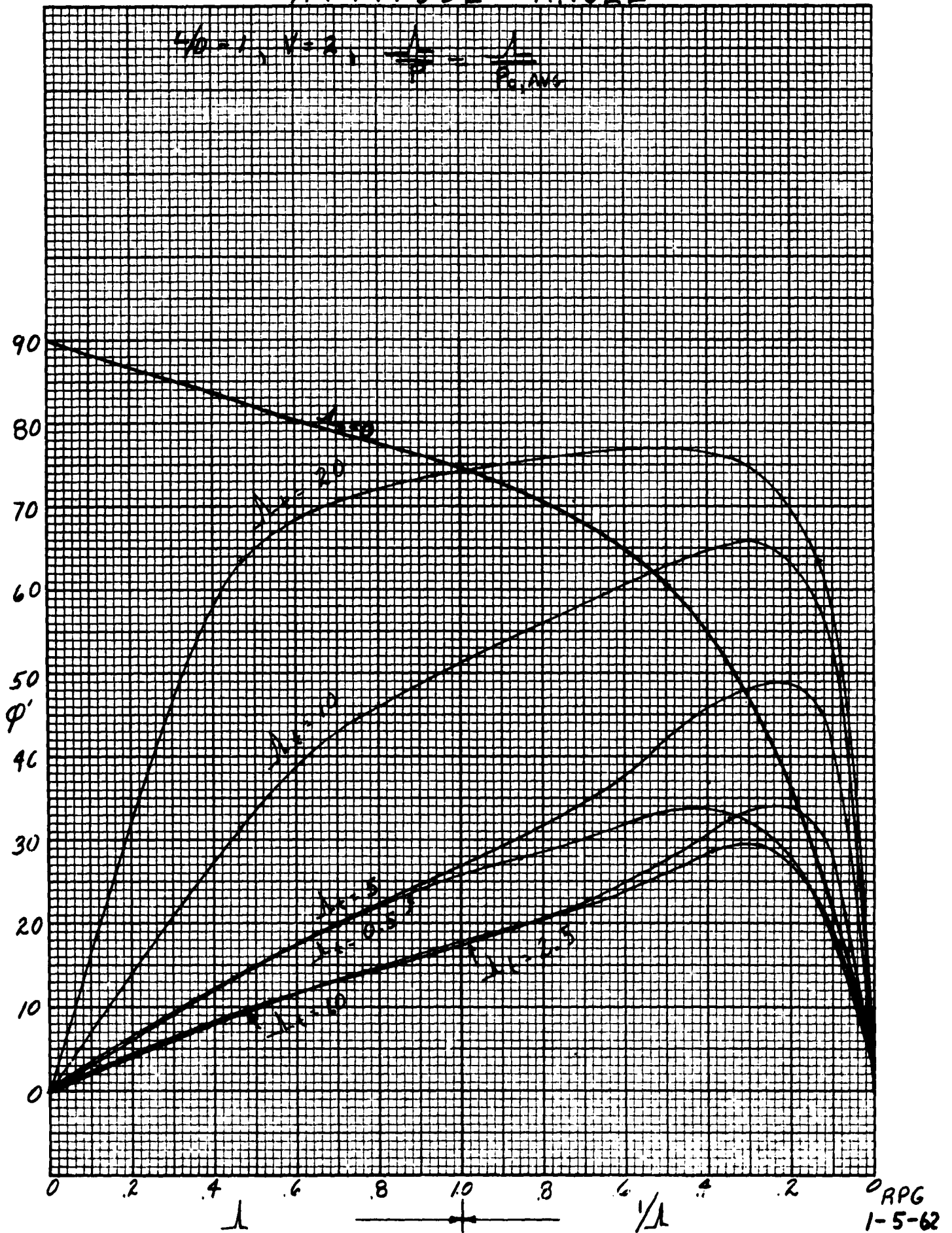
FIG. 7 ATTITUDE ANGLE
