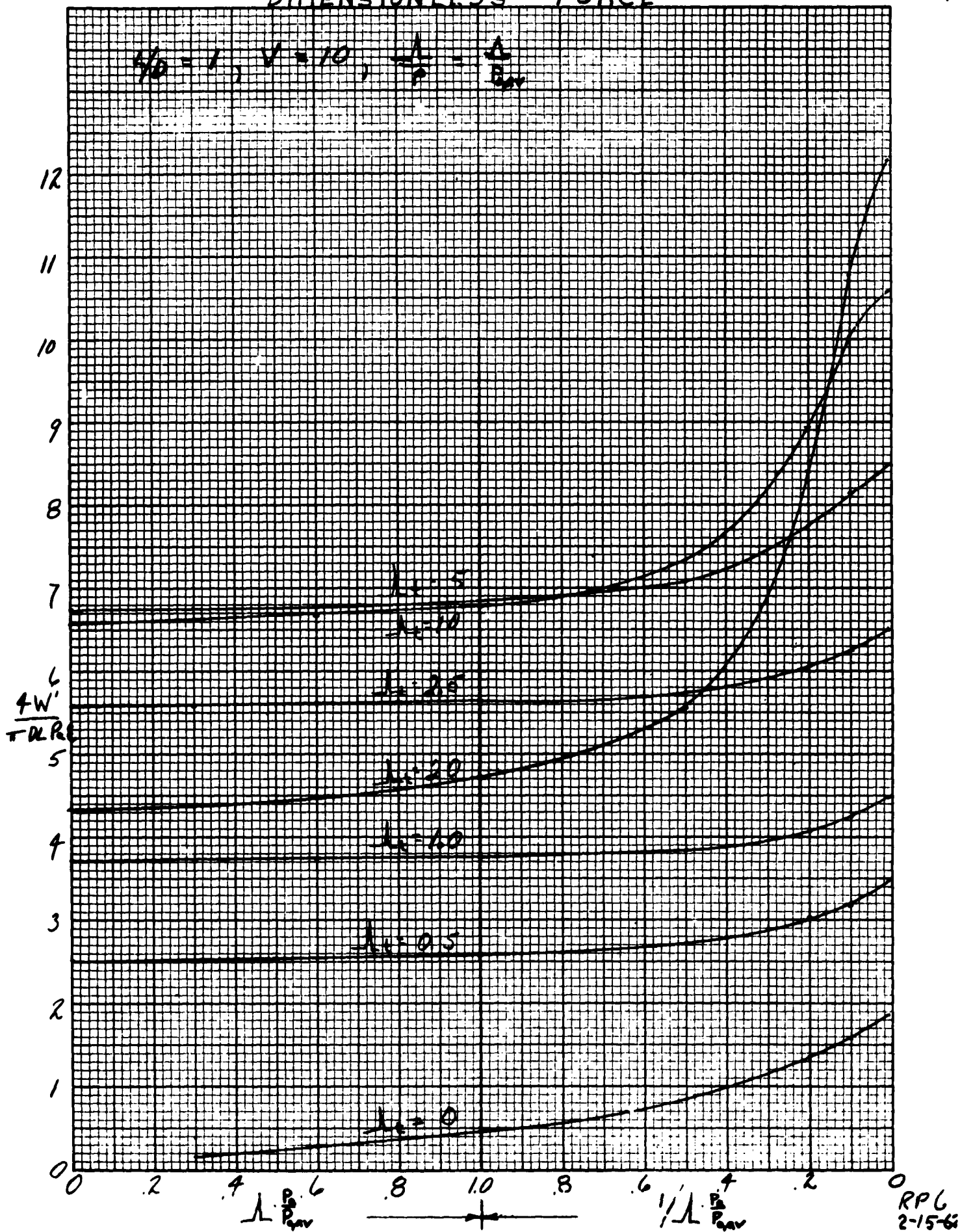
FIG.30 DIMENSIONLESS FORCE
