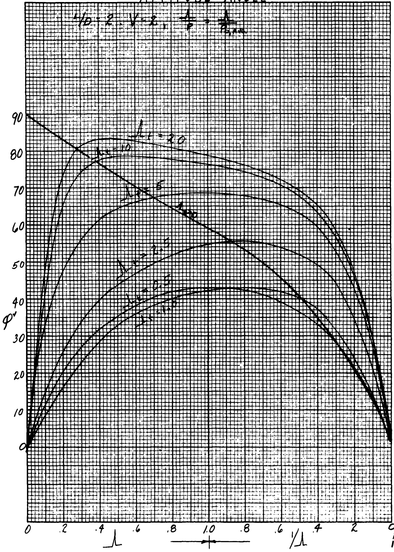
FIG. 10 ATTITUDE ANGLE
