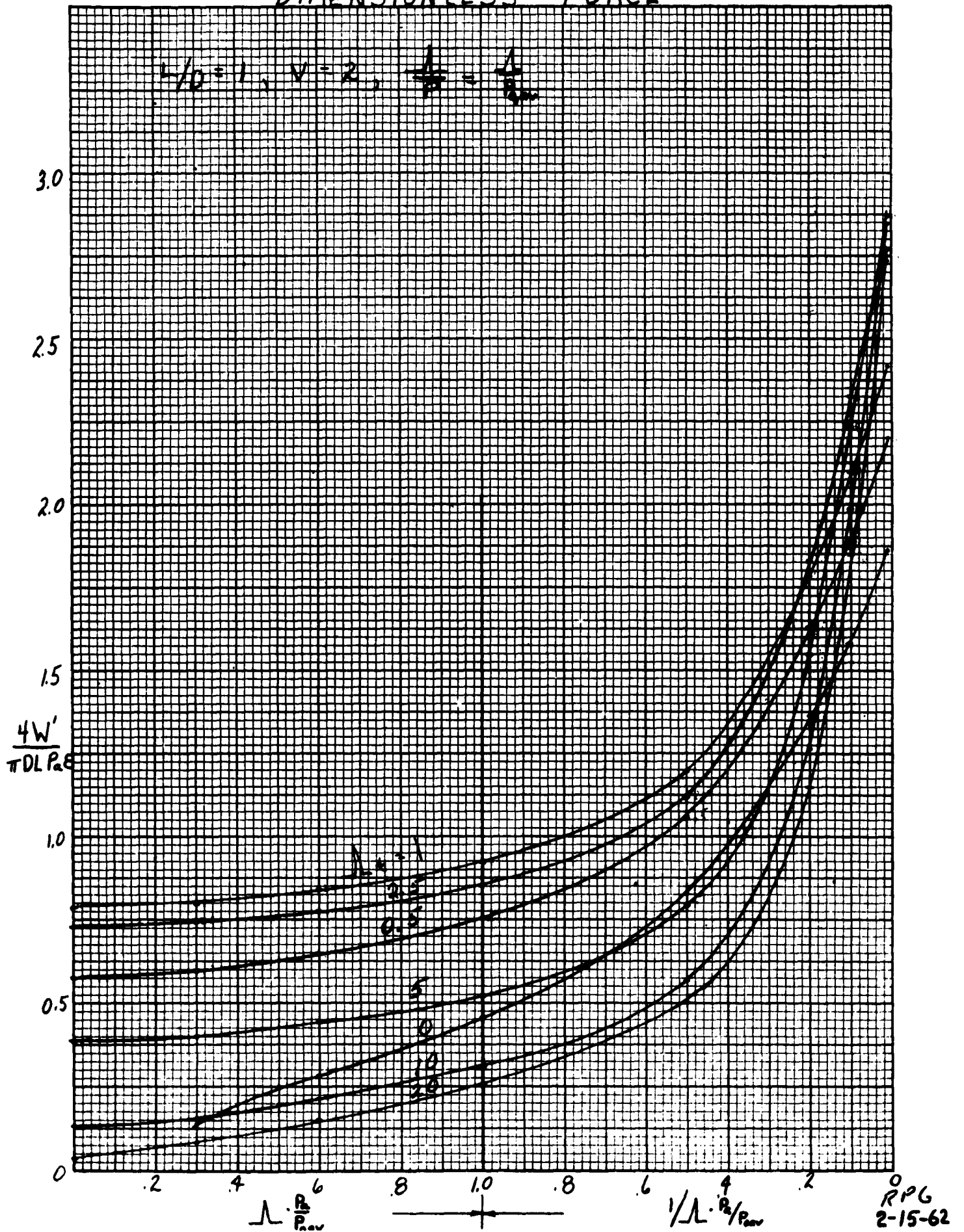
FIG. 29 DIMENSIONLESS FORCE
