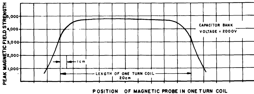
FIGURE 6. PLOT OF MAGNETIC FIELD VS DISTANCE ALONG ONE TURN COIL
