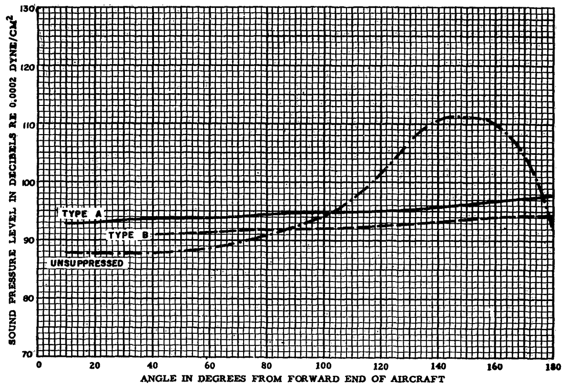
Figure 13. SPL at 250 Feet; 20-75 CPS
