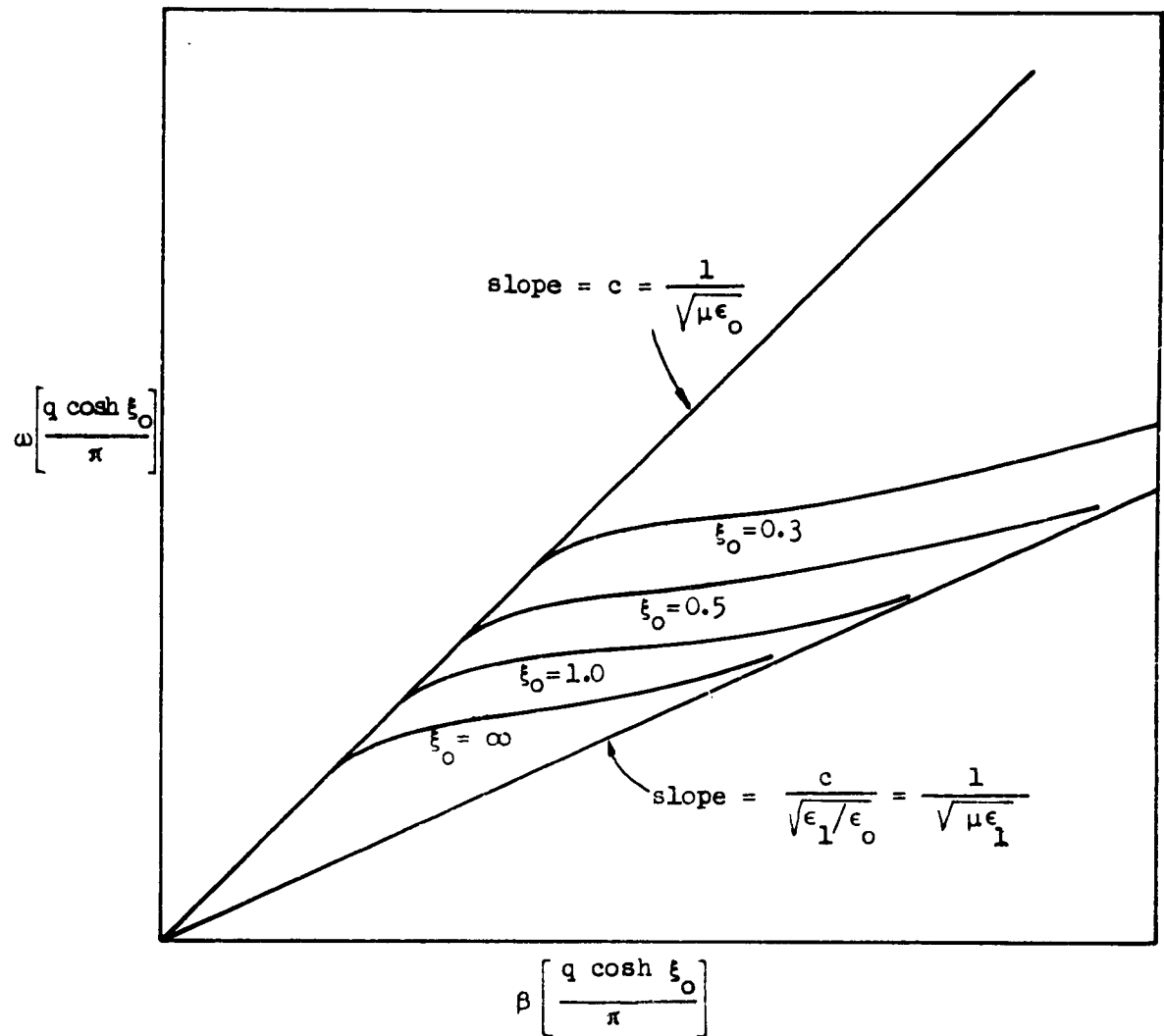
Fig. V-4. A sketch of the \omega - \beta diagram for the dominant dielectric rod mode.
