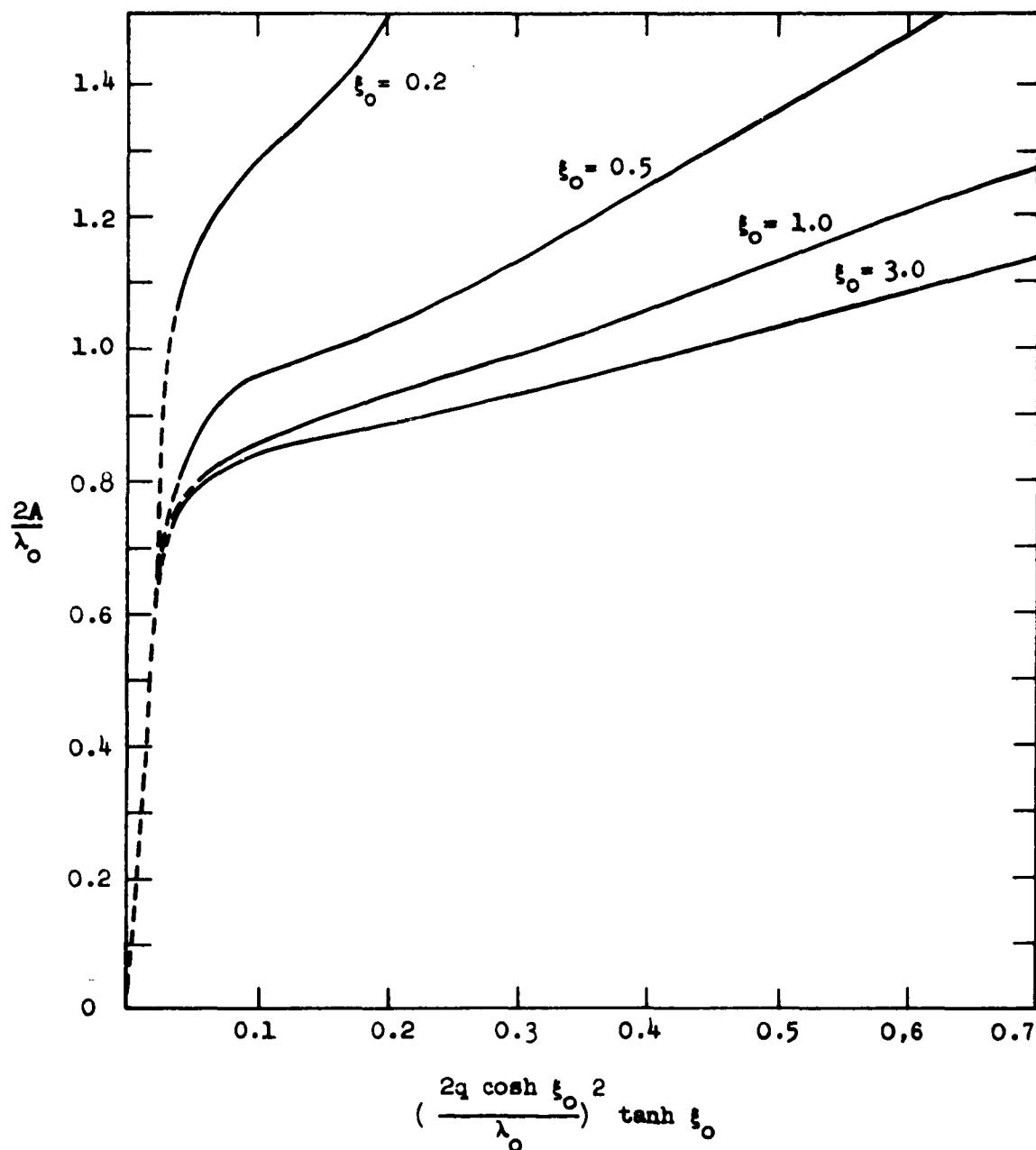
Fig. III-26. Normalized axial electric field extent 2A/\lambda_0 as a function of the normalized cross-sectional area for the {}_{0}\text{HE}_{11}^{(1)} mode. A is the distance measured from the origin to the point of observation where (E_z/E_{z_0})^2 = 0.1
