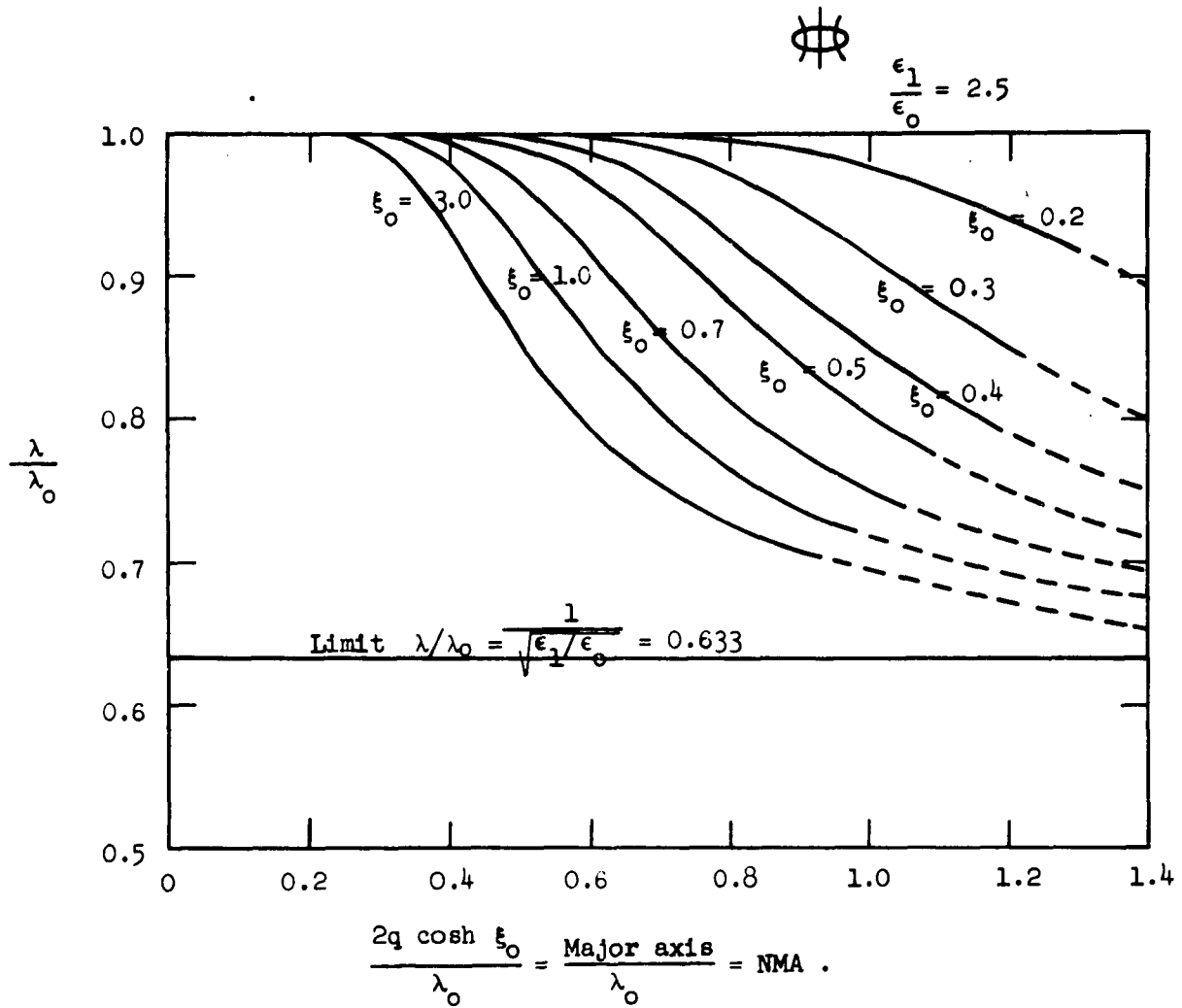
Fig. III-2. Normalized guide wavelength \lambda/\lambda_0 of the {}_{e\text{HE}}^{(1)}_{11} mode as a function of normalized major axis.
