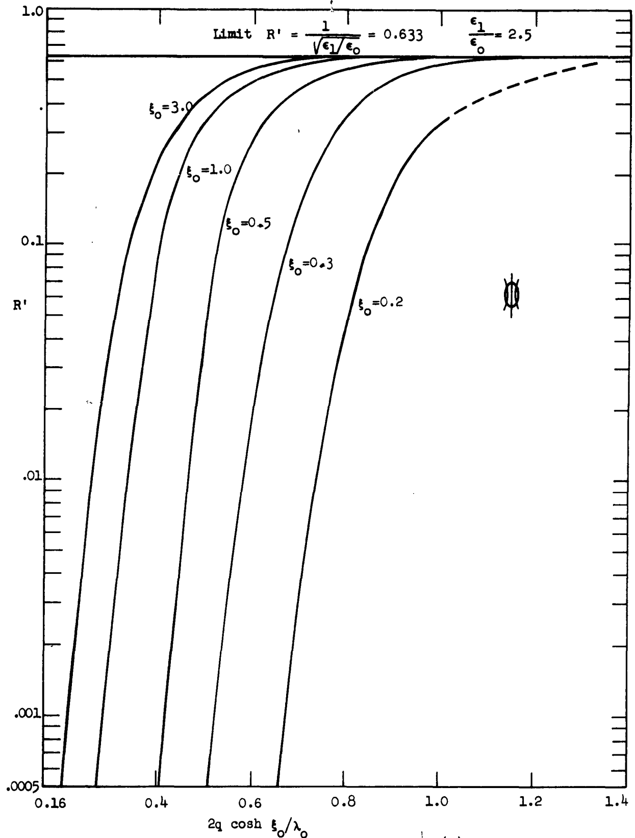
Fig. IV-4. The attenuation factor R' for the HE_{11}^{(1)} mode as a function of the normalized major axis.
