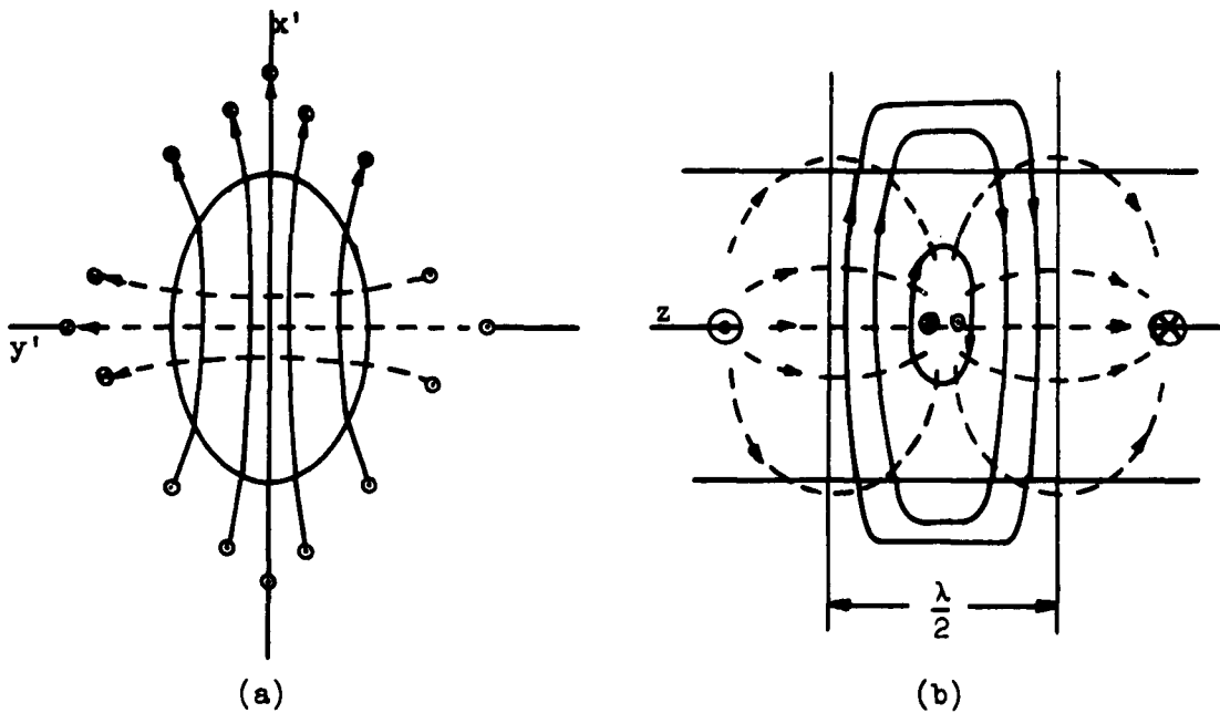
Fig. III-12. Field configuration of the {}^o\text{HE}_{11}^{(1)} mode (a) cross section (b) longitudinal section
