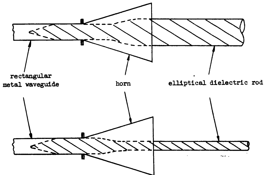
Figure VI-3. The Launching Device.
