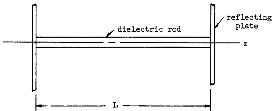
Figure V-1. The Elliptical Dielectric Rod Resonator
