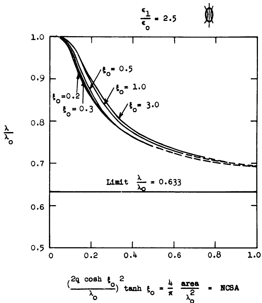
Fig. III-9. Normalized guide wavelength of the {}_{0\text{HE}}^{(1)}_{11} mode as a function of normalized cross-sectional area.
