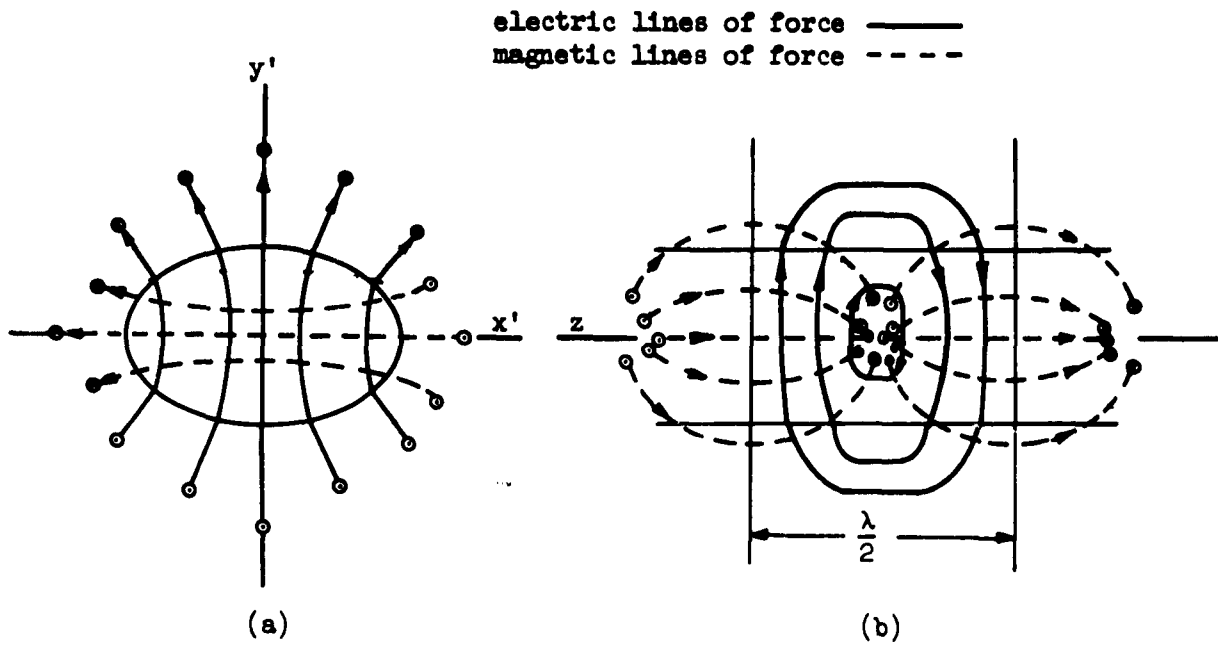
Fig. III-11. Field configuration of the {}^e\text{HE}_{11}^{(1)} mode. (a) cross section (b) longitudinal section
