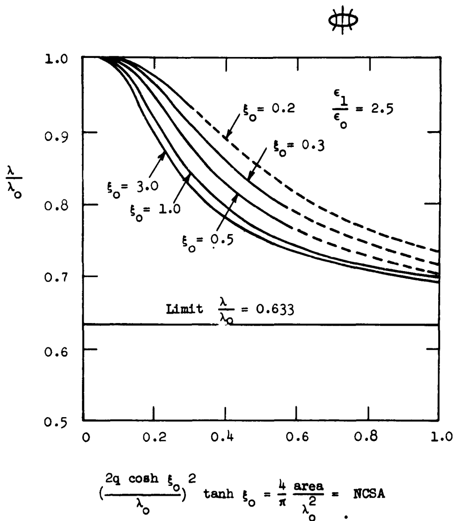
Fig. III-4. Normalized guide wavelength of the e_{HE_{11}}^{(1)} mode as a function of normalized cross-sectional area.
