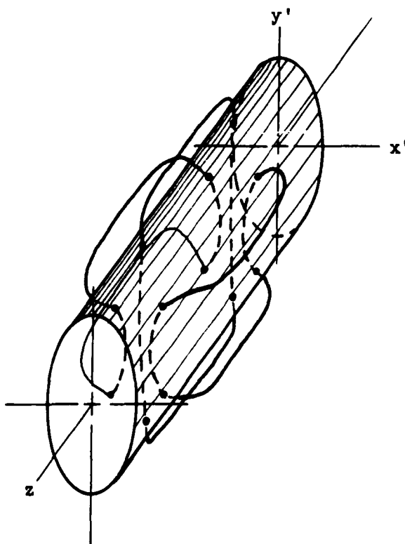
Fig. III-14. A sketch of the electric lines of force for the oHE_{11}^{(1)} mode
