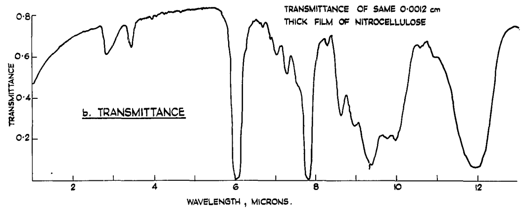
EMISSION AND TRANSMITTANCE OF NITROCELLULOSE FILM.
