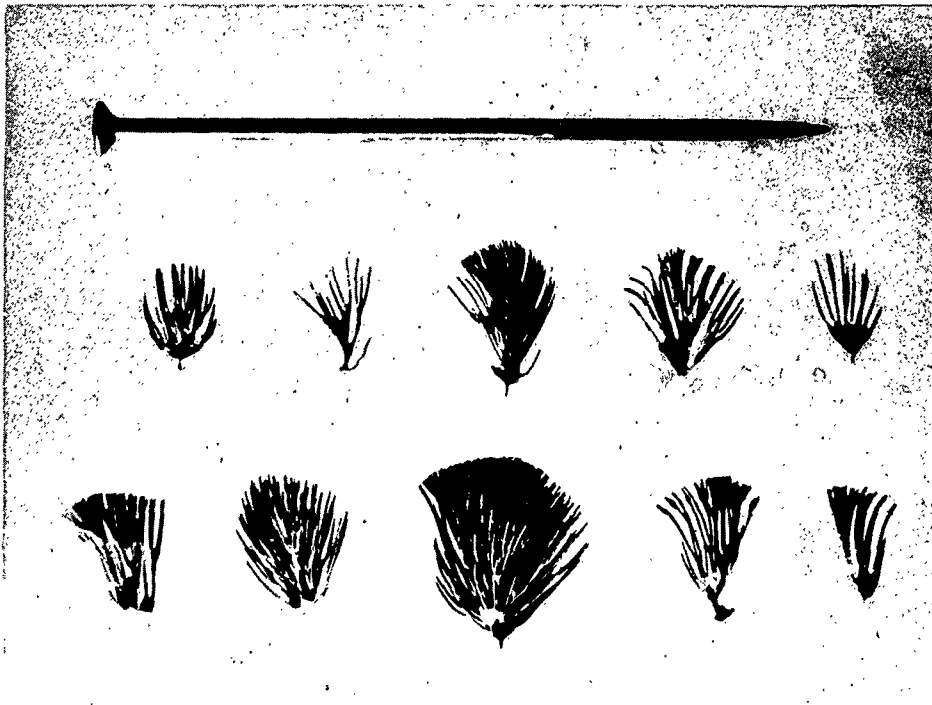
Figure 7 "BUSH" FORM OF SILICON METAL FOUND TO DEPOSIT IN AREA A OF REACTION TUBE -3.5 X MAG.
