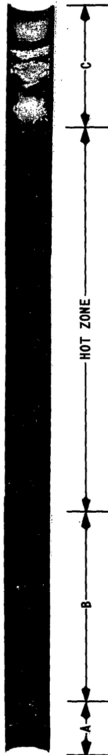
Figure 5 GRAPHITE REACTION TUBE ILLUSTRATING TYPICAL AREAS OF FORMATION AND GROWTH OF REACTION PRODUCTS.
