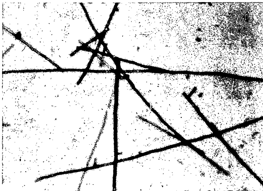
Figure 8 SHORT, STUBBY NEEDLE-LIKE GROWTH OF SiC TYPICAL OF FORMATION IN AREA B
