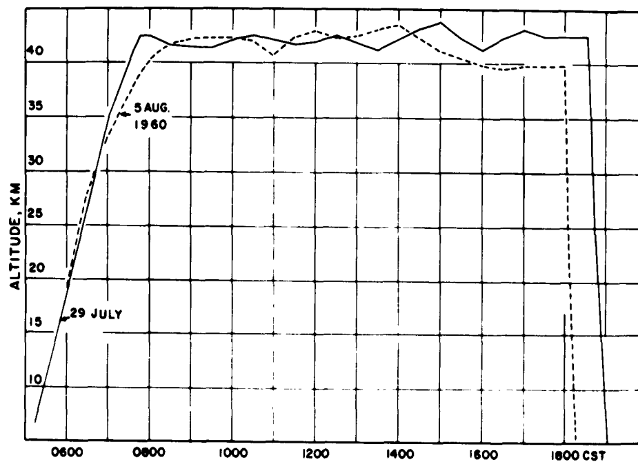
Figure 2. Flight trajectories of the 9 million cu ft balloons
