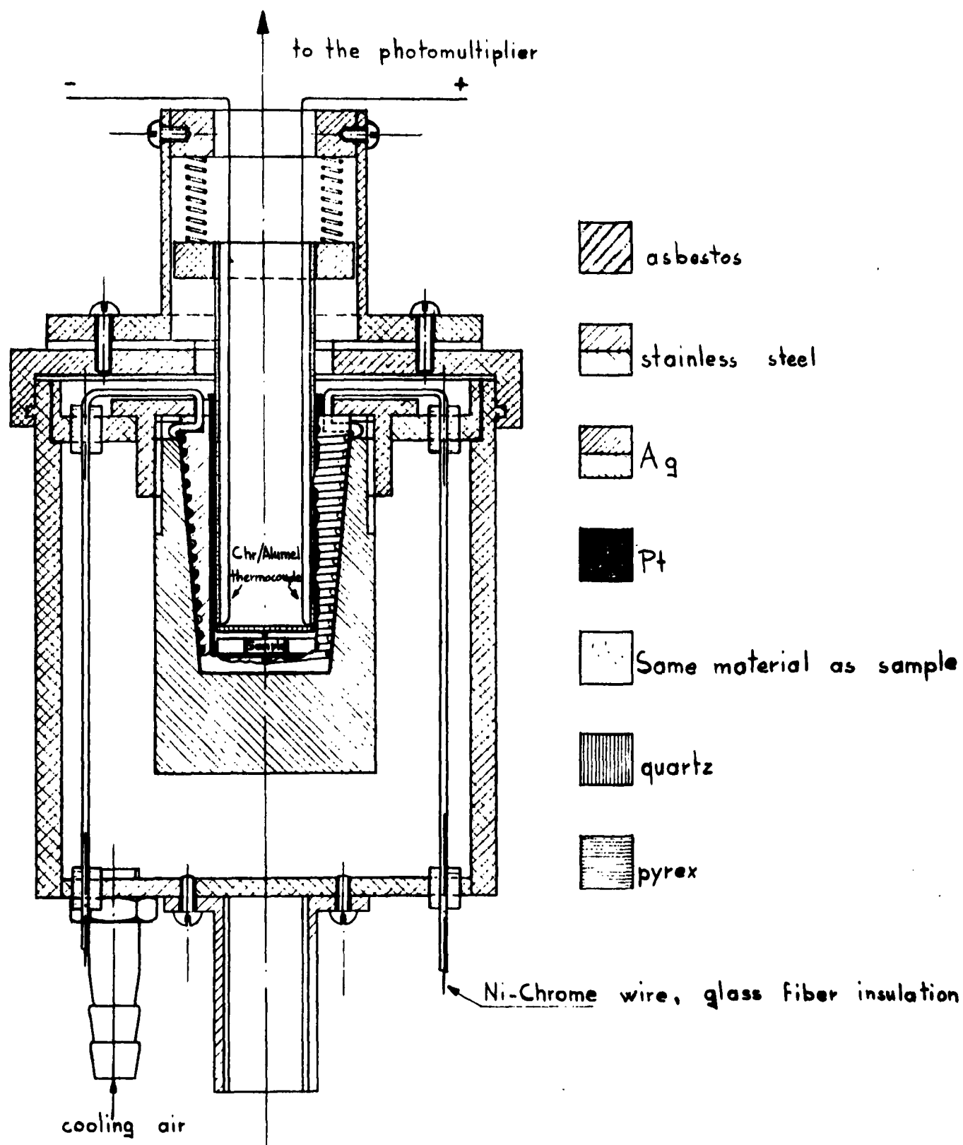
Thermoluminescence Furnace
