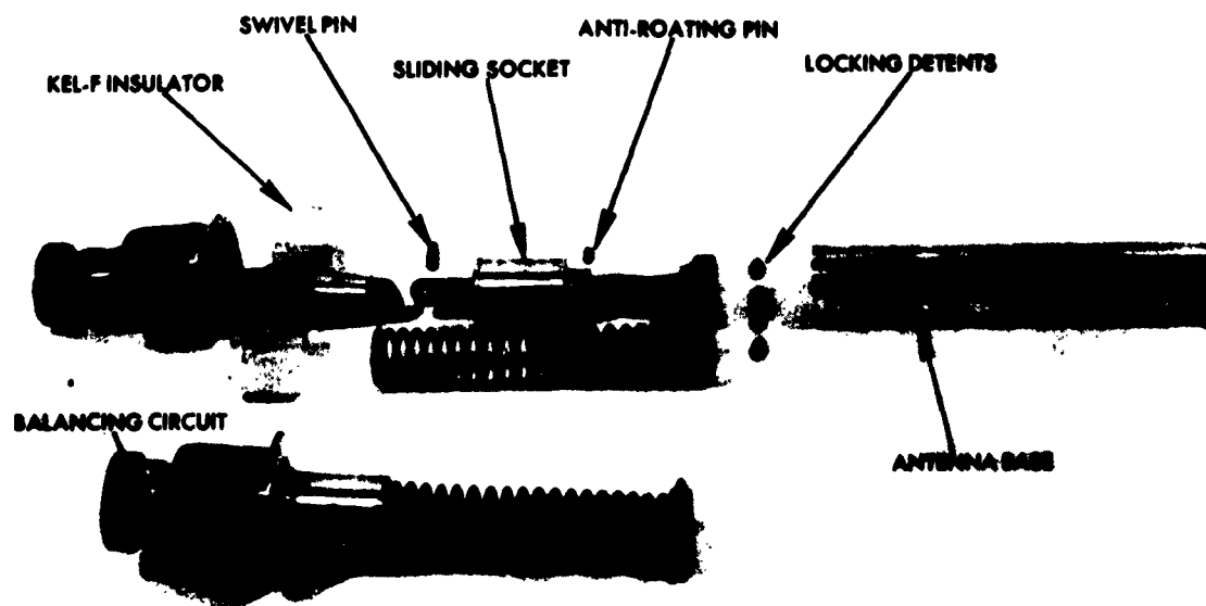
Figure 7 — Antenna folding and locking device
