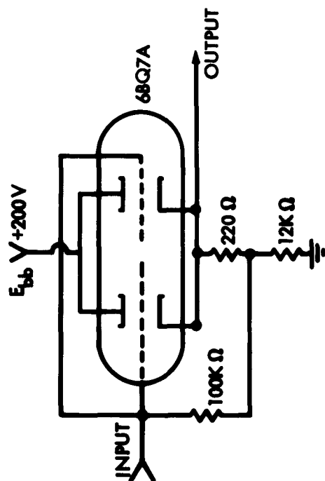
b. CATHODE FOLLOWER
