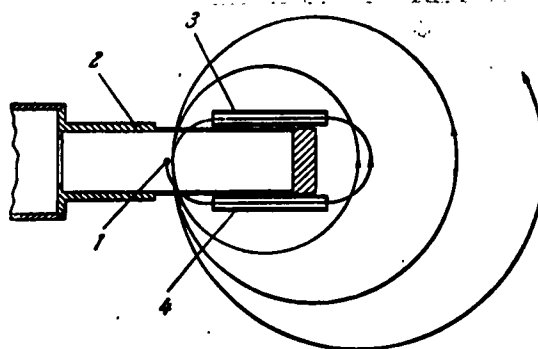
Fig. 15. Diagram of the placement of magnetic shields making it possible to increase the upper limit of the strength of the master magnetic field. 1--cathode; 2--cylindrical resonant cavity; 3,4--magnetic shields.
