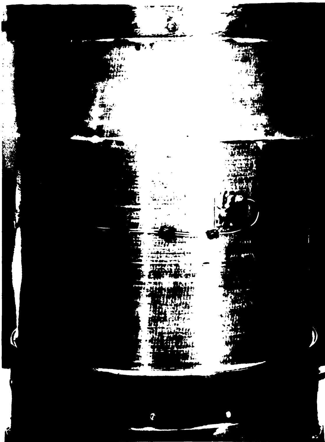
Figure 9. Subscale Case 2 after Failure
