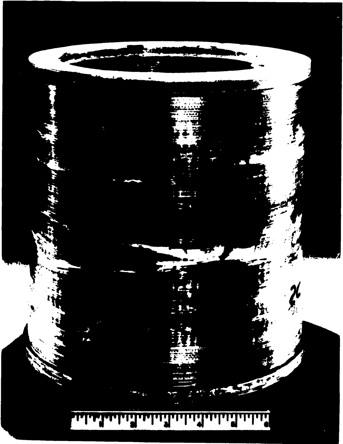
Figure B-3. Sandwich-Wall Cylinder 7 After Test
