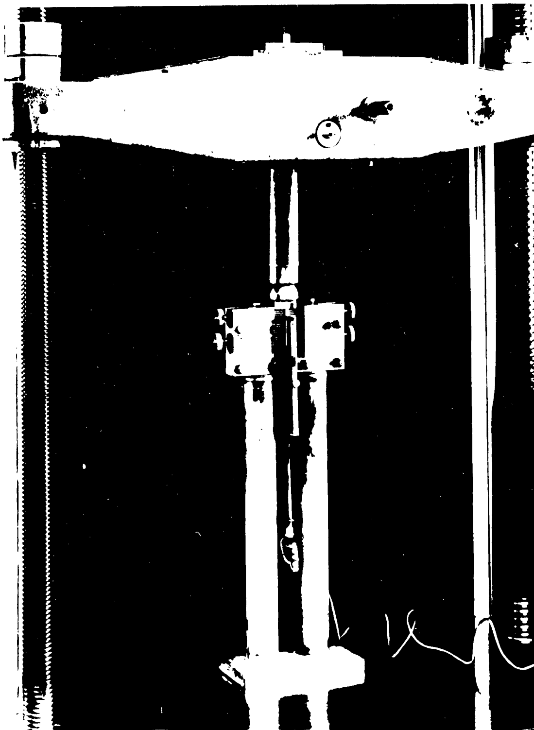
Figure 2. Typical Edgewise Compression Test Fixture
