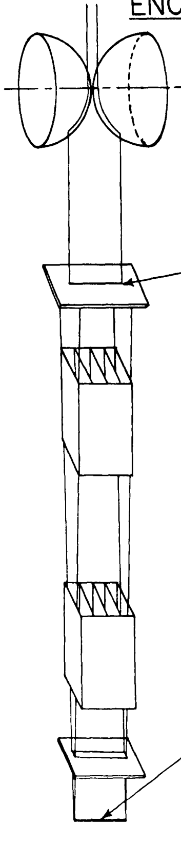
FIG A - VERTICAL SOURCE - PARALLEL PLATES LIMIT VERTICAL DIVERGENCE
