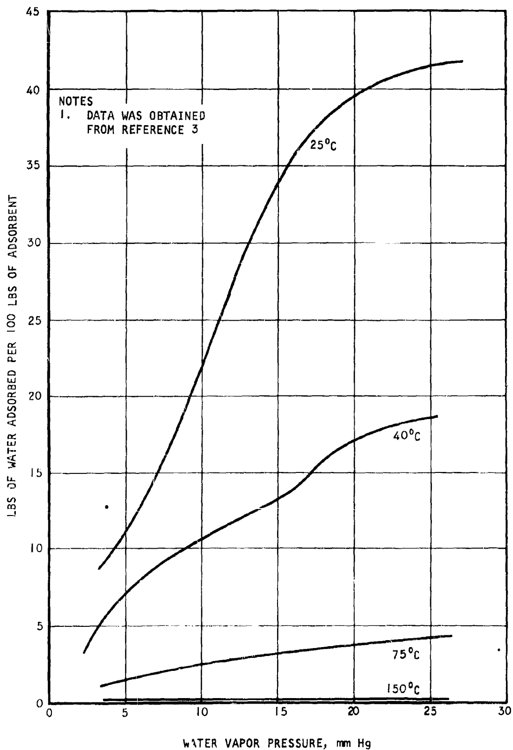
Figure 5. Water Vapor Adsorption Isotherms for Silica Gel
