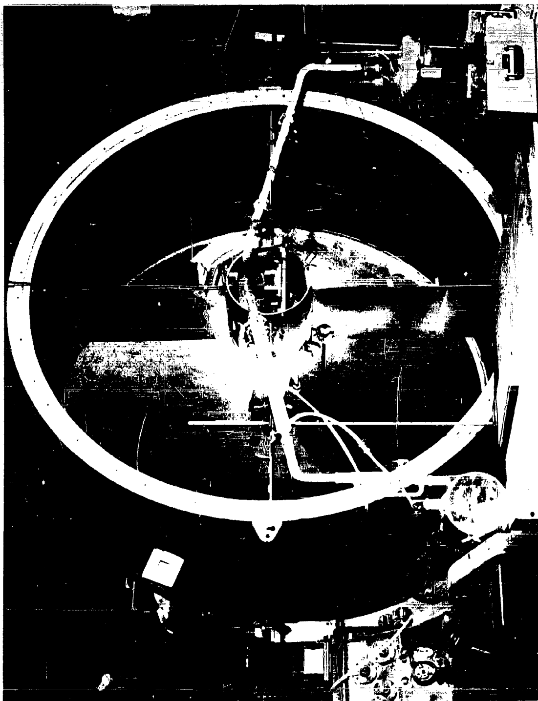
FIG. 11. SOLAR FURNACE IN OPERATION
