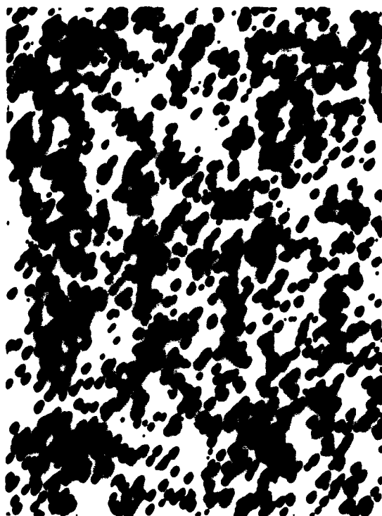
Fig. 22 Etch pits near neutral axis on the (112) surface of crystal bent about [112] axis--500X. Note the glide polygonization evident perpendicular to the glide bands marked S.
