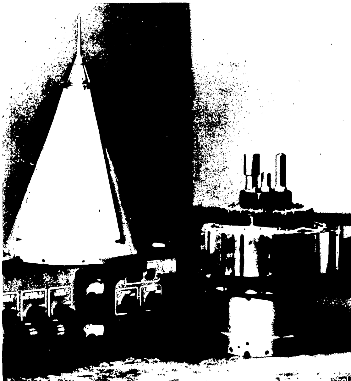
Figure 2 - The two Geiger-Müller Counters are located in the two outside vertical cylinders on the top of the Pioneer IV payload
