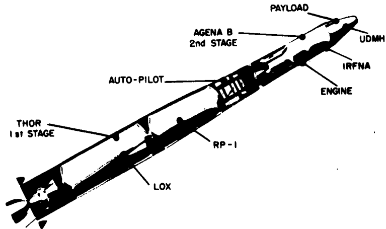
Figure 9 - The Thor-Agena B launch vehicle
