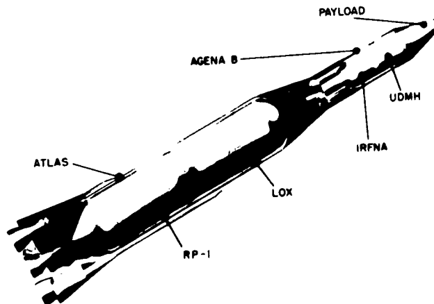
Figure 10 - The Atlas-Agena B launch vehicle
