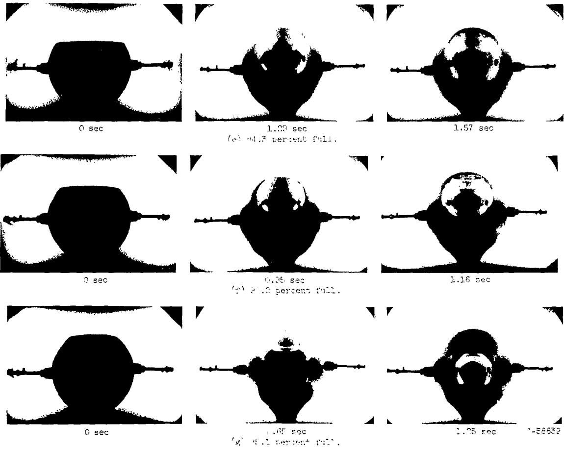
Figure 26. - Included. High speed in 1.0-millisecond glass sphere over range of liquid-to-tank-volume ratios.
