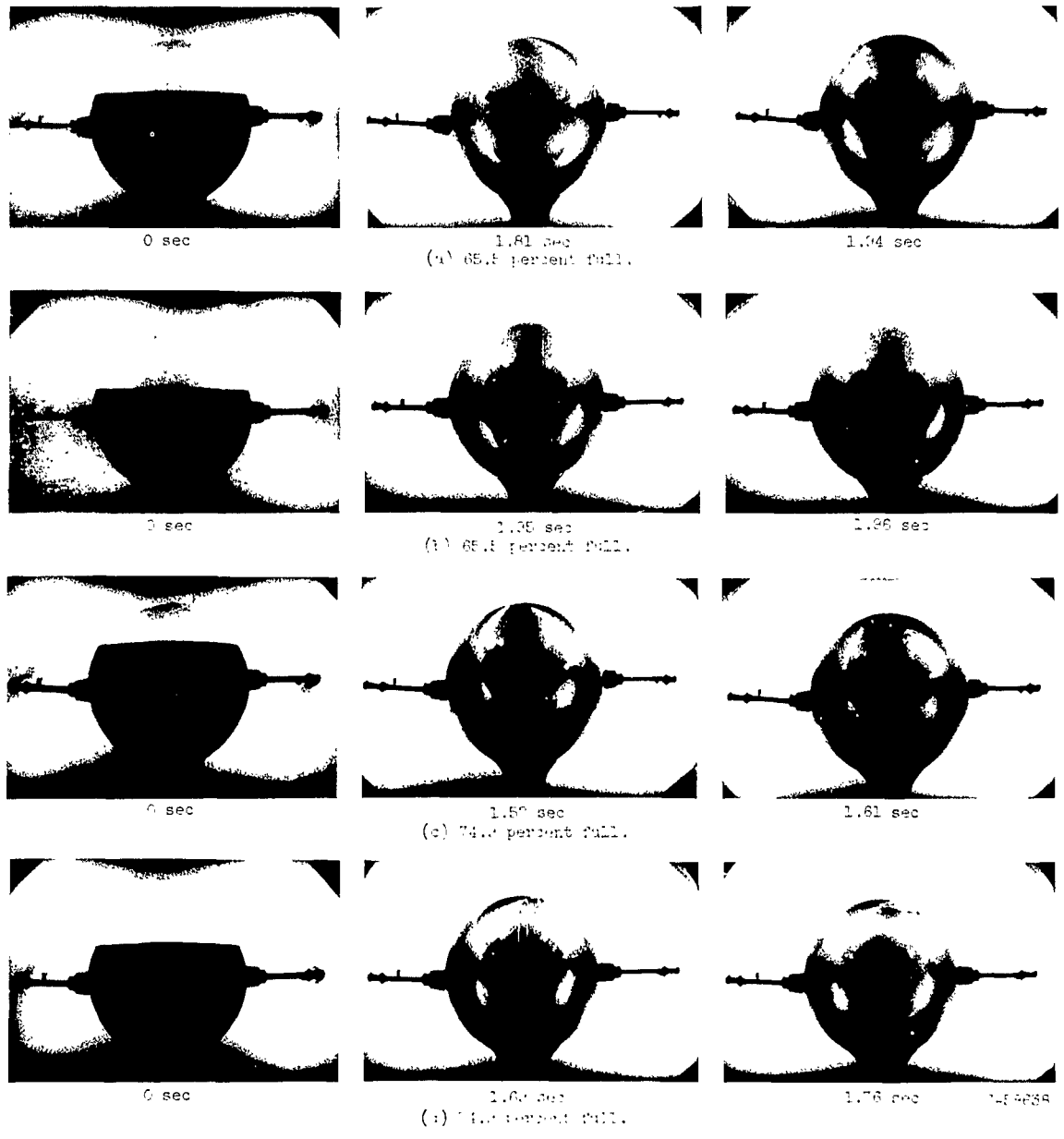
Figure 20. - High speed, 10,000-frames-per-second glass spheres over various liquid-to-tank-volume ratios.
