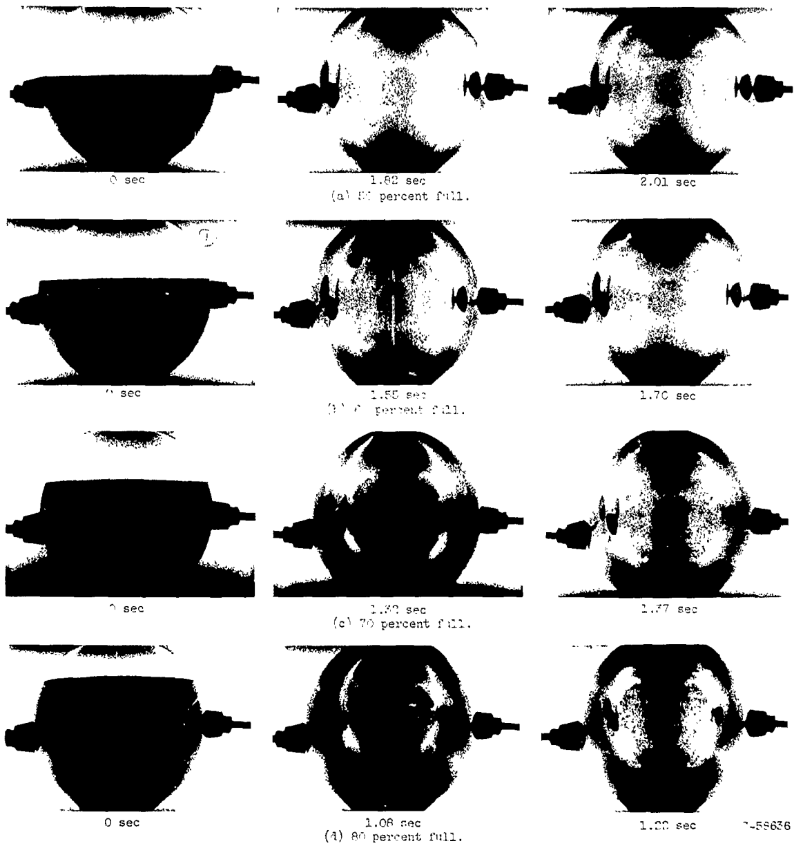
Figure 25. - Methyl alcohol in 100-milliliter glass spheres over range of liquid-to-tank-volume ratios.
