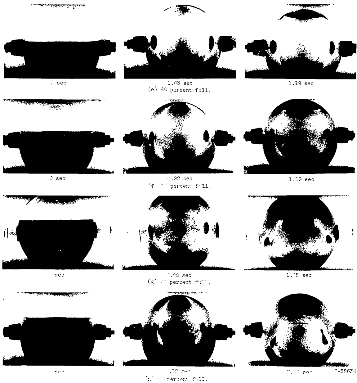
Figure 21. - (Continued). High speed 16 mm. millimeter glass spheres over range of liquid-to-tank-volume ratios.
