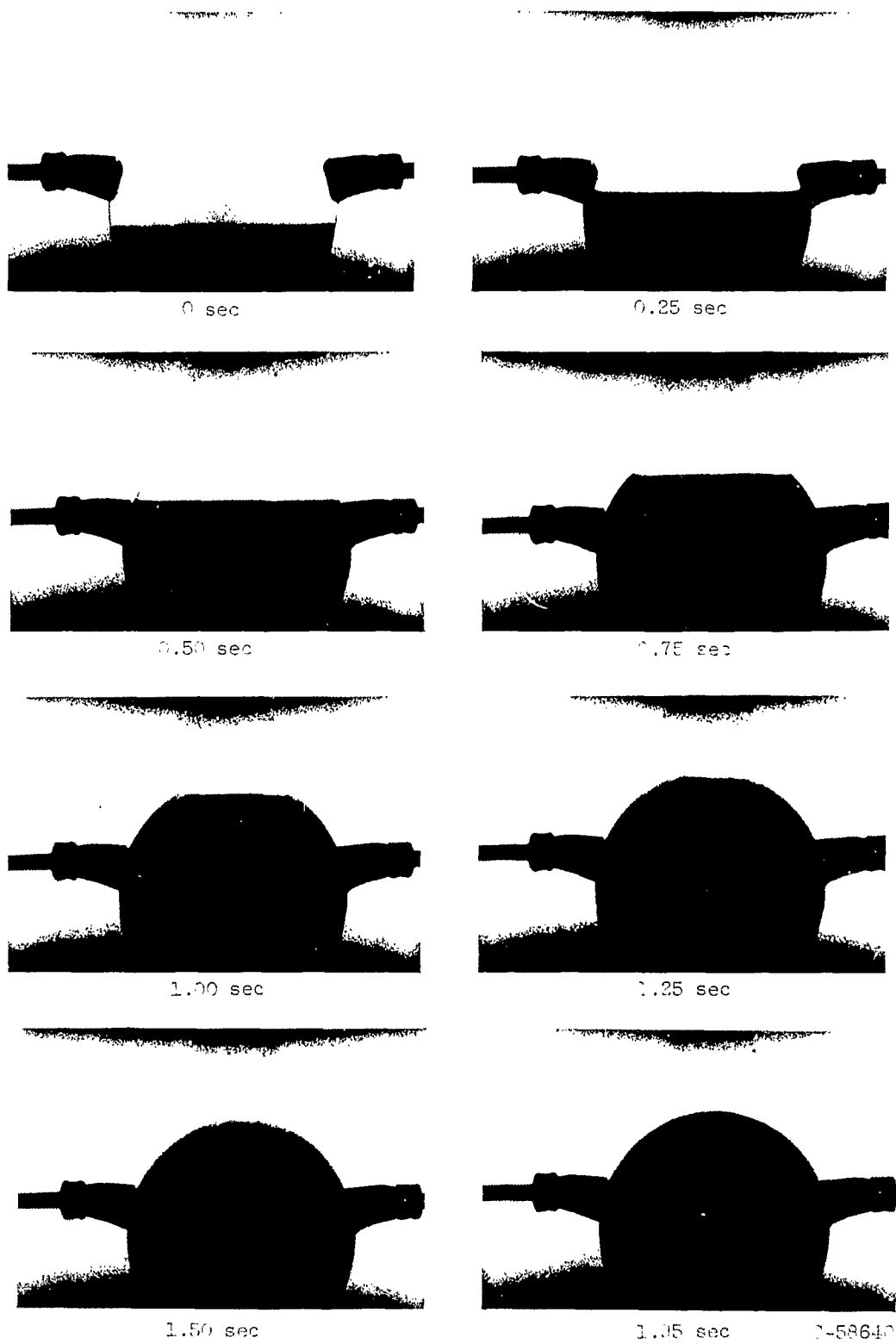
Figure 27. - 40% alcohol in 100-milliliter glass sphere during 1.75 seconds of zero gravity at liquid-to-tank-volume ratio of 35 percent.
