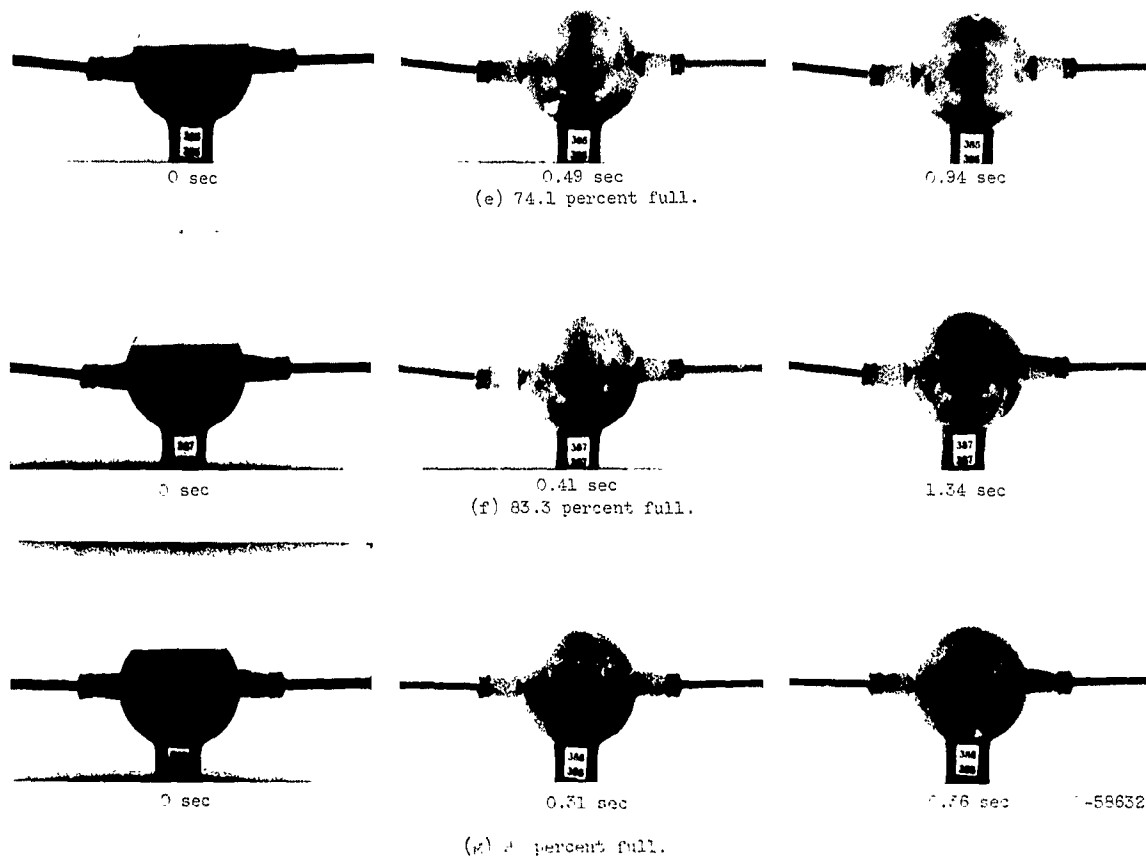
Figure 27. - Concluded. Ethyl alcohol in 64-milliliter glass spheres over range of liquid- to tank-volume ratios.
