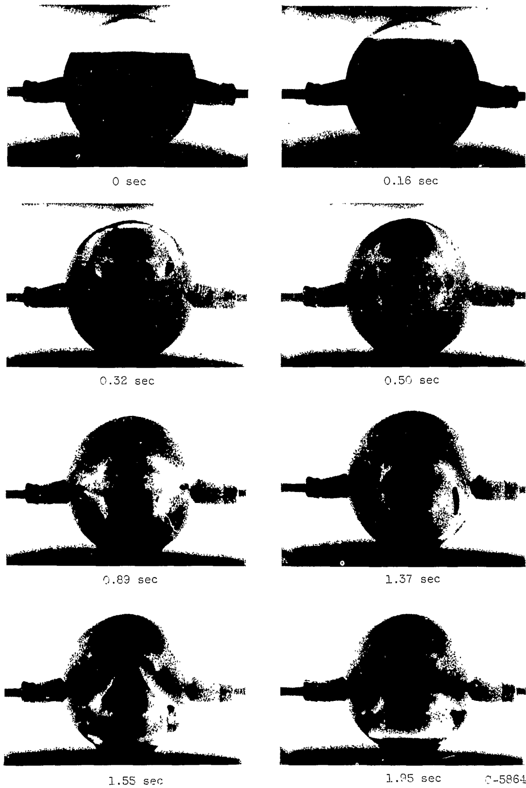
Figure 32. - Ethyl alcohol in 300-milliliter glass sphere during 1.95 seconds of zero gravity at liquid- to tank-volume ratio of 80 percent.
