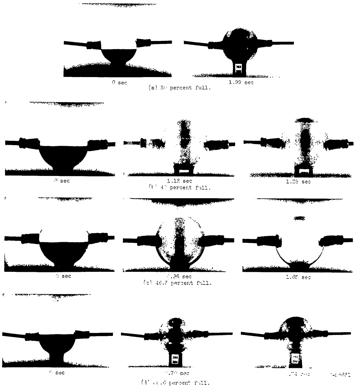
Figure 23. - Ethyl alcohol in 11-millimeter glass spheres over range of liquid-to-vacuum ratio.
