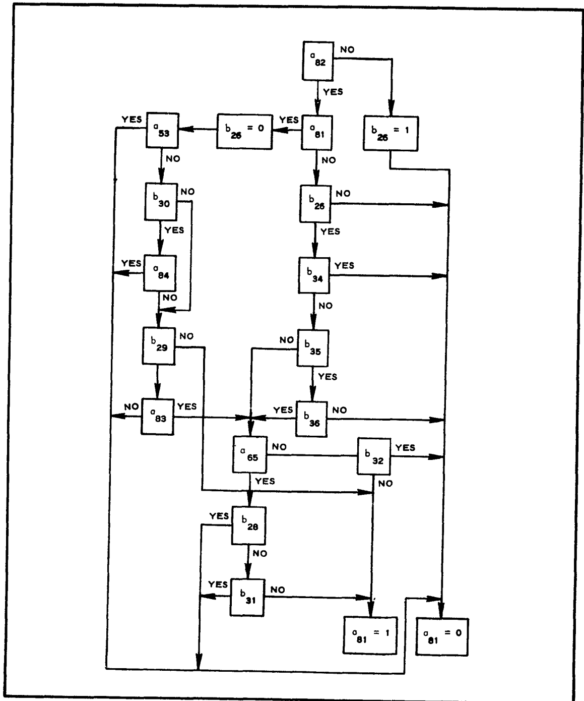
Figure D-26 - Afterburner Light-Off and Blowout Routine
