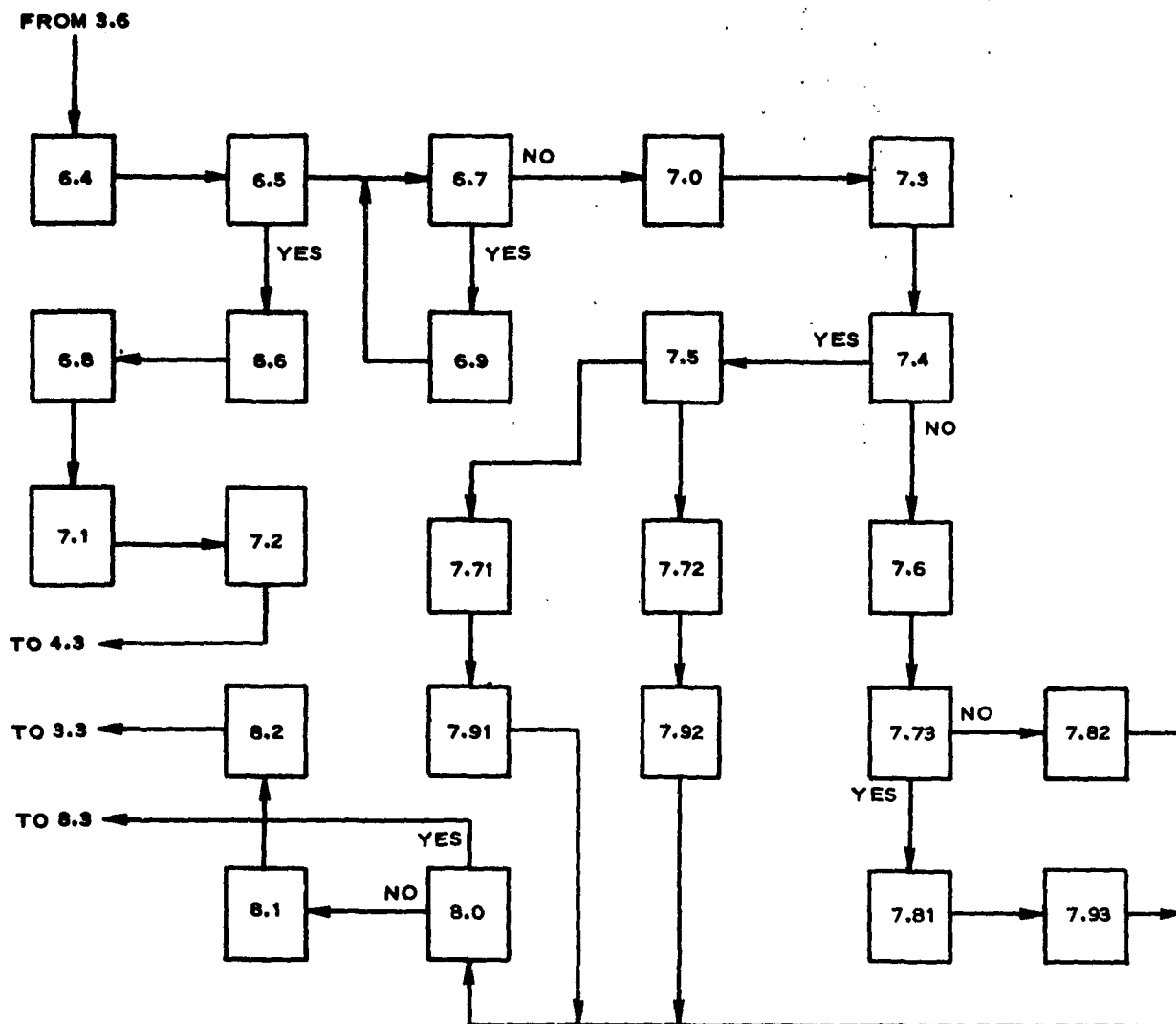
Figure E-10 - Subroutine VI Tank Volume, Input Rate Logic
