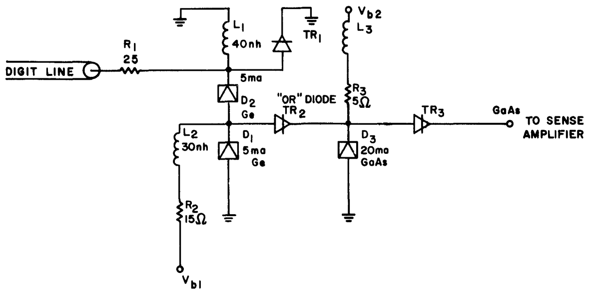
Figure 5-25. Sense Amplifier Circuit
