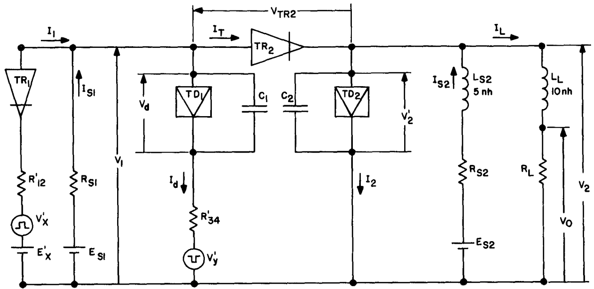
Figure 5-12. Equivalent Circuit of Two-Stage Driver
