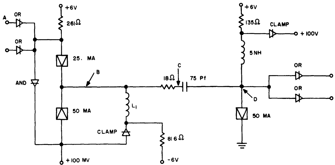
Figure 2-51. Delay Circuit
