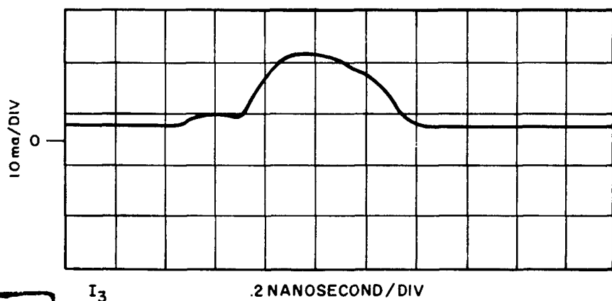
Figure 2-30. Waveforms of Computer Run 32
