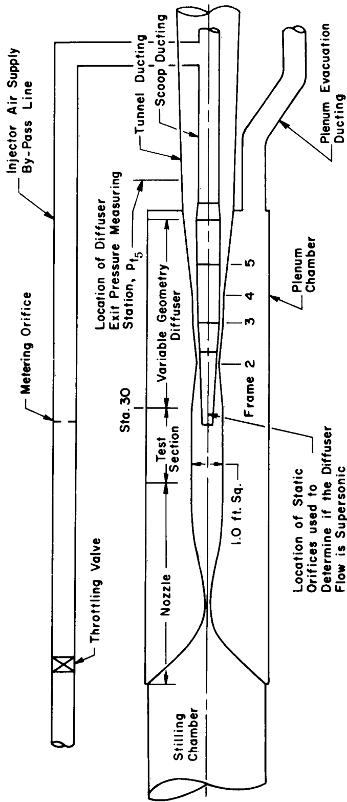
Fig. 1 Schematic of the Supersonic Model Tunnel
