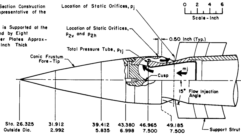
Fig. 5 Injector C Geometry, A_i^* = 9.48 \text{ in.}^2 and M_i \approx 2.6
