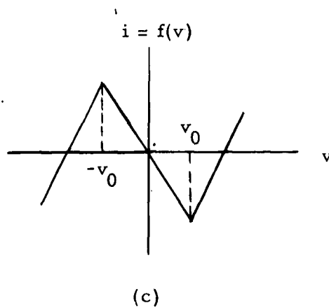
Figure 3 Tunnel Diode Oscillator
