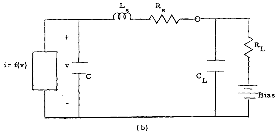
Figure 2 Tunnel Diode with Load and Bias
