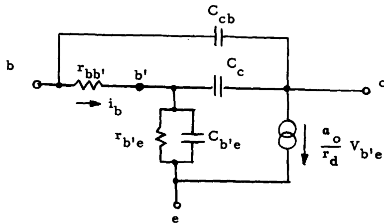
Figure 13. Equivalent Circuit of the Transistor Assumed in Determination of r_{bb'}
