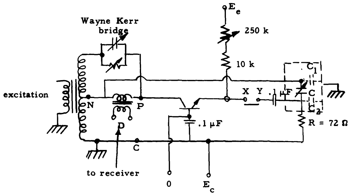
Figure 12. Circuit Arrangement of Figure Used for Measurement of r_{bb'} , C_c and C_o
