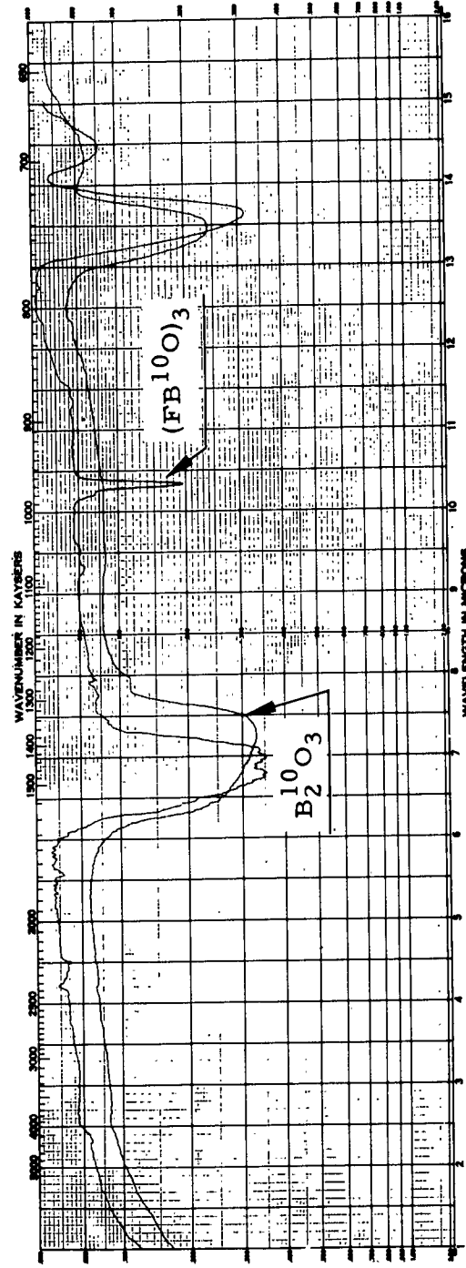
Figure 2. Infrared Spectra of Labeled Trifluoroboroxines and Labeled Boric Oxides
