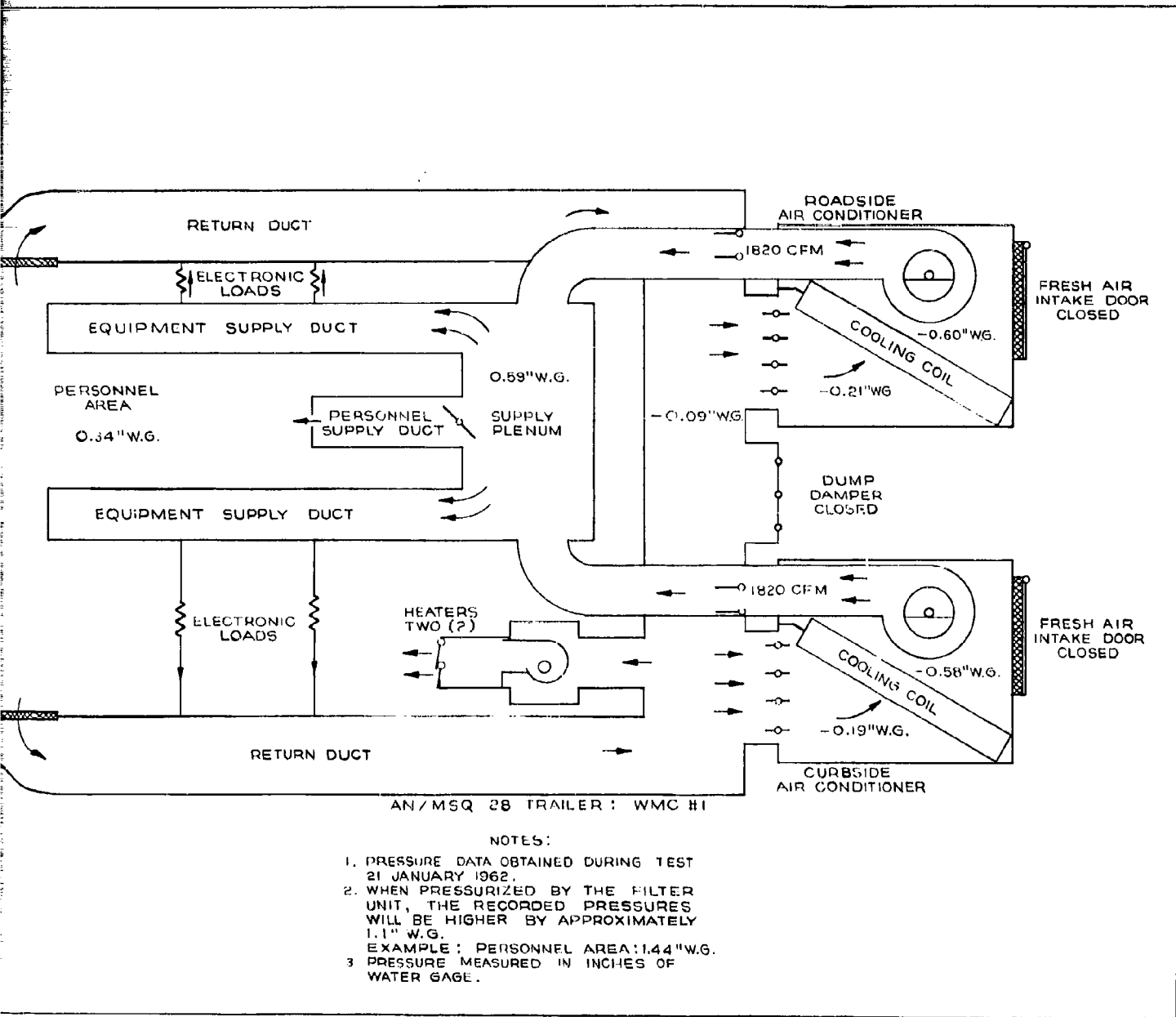
Figure 11 Actual Operating Pressure of AN/MSQ-28 WMC
