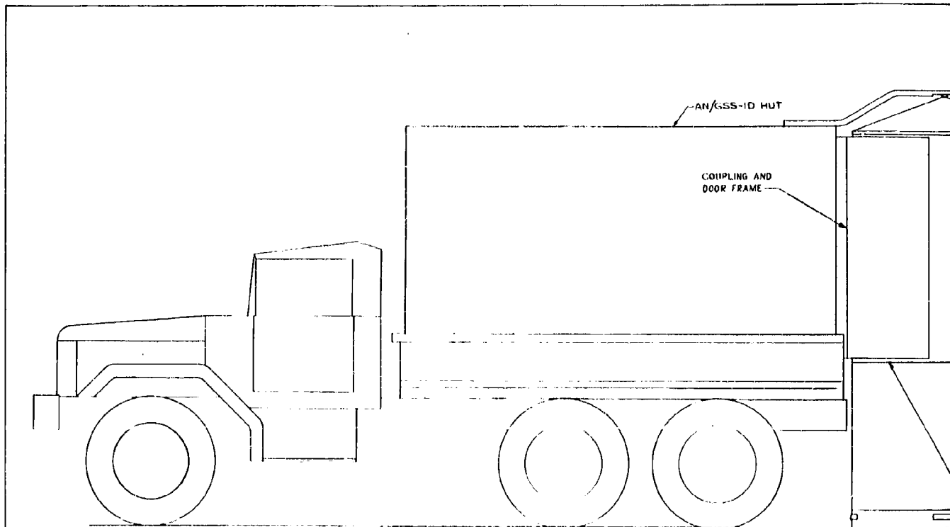
TRUCK MOUNTED PROTECTIVE ENTRANCE SCALE 1/40
