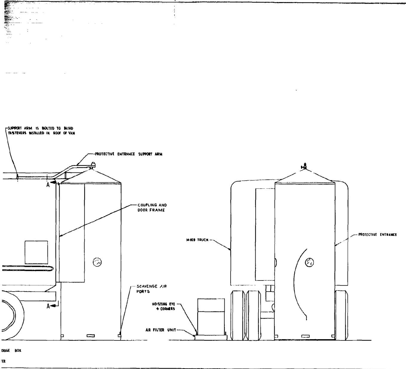
Figure 18 Category A Collective Protection Equipment for OC & CDG Vehicles (AN/MSQ-18)
