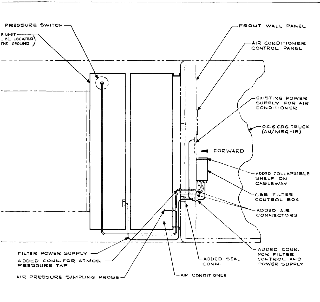
Figure 19 AN/MSQ-18 Vehicle Modifications Required for Filter Unit Control System
