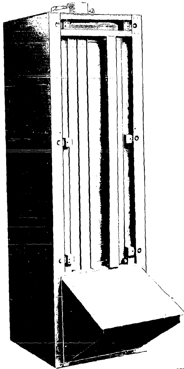
Figure 4 400 CFM Filler Unit with Aerogel Filter Partially Removed
