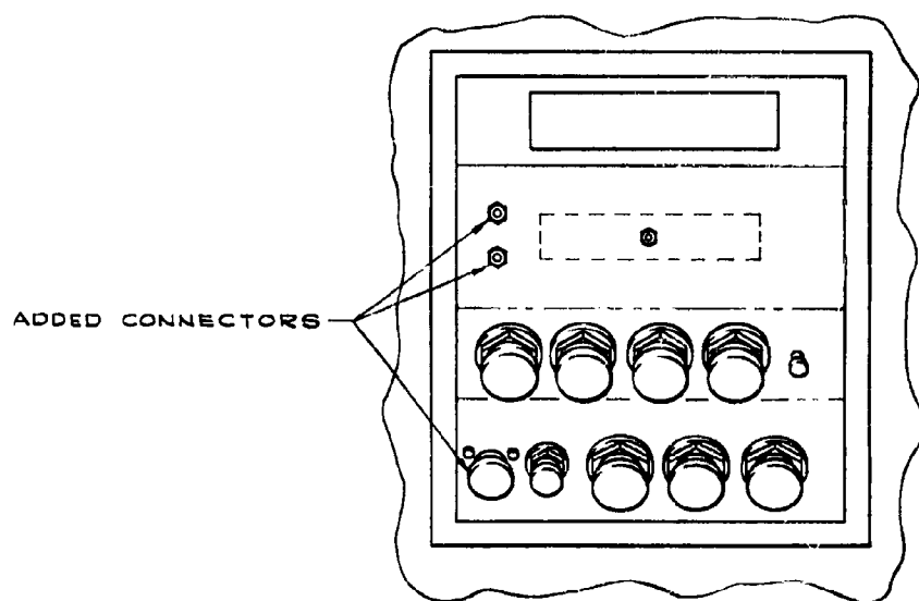
VIEW 13-13 ROTATED 180° SHOWING RIGHT SIDE POWER PANEL
