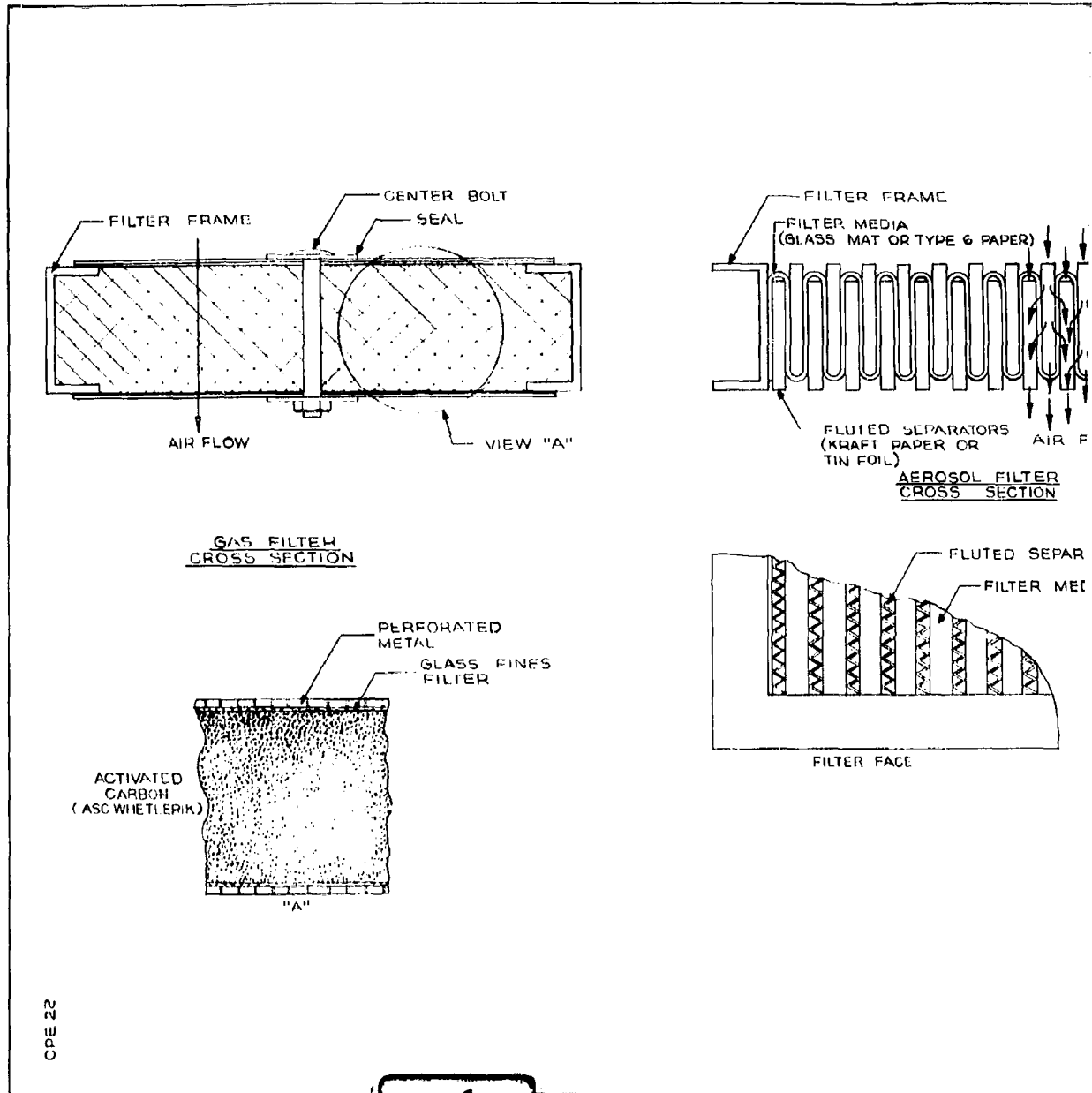
Figure 12 Typical Construction of Aero
