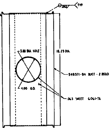
VIEW A SCALE 1/2
