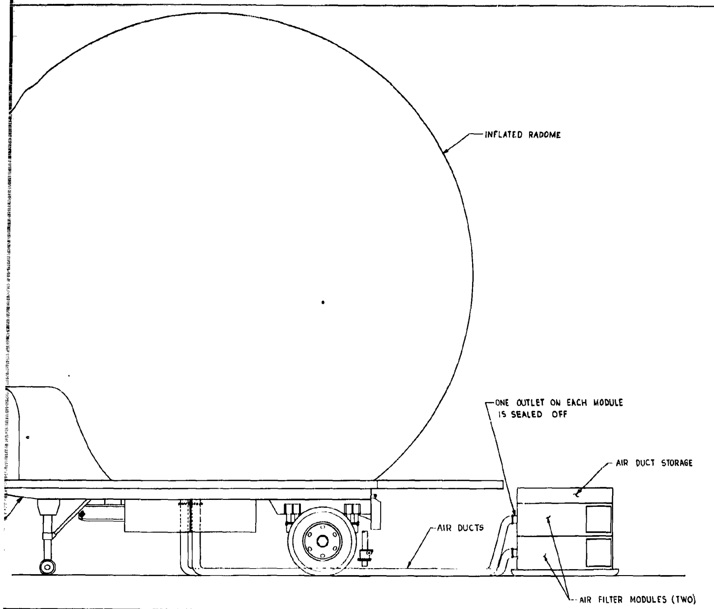
Figure 17 Category B Collective Protection Equipment for AN/MP8-23 Radar Antenna Trailer
