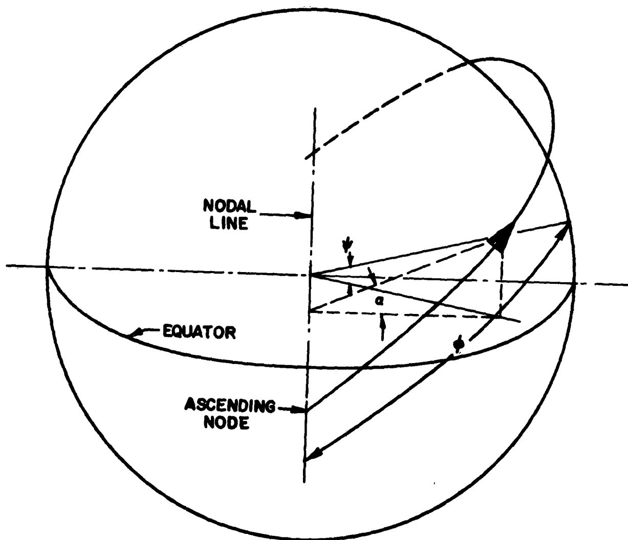
Fig. 2 - Geometric Parameters for an Inclined Orbit
