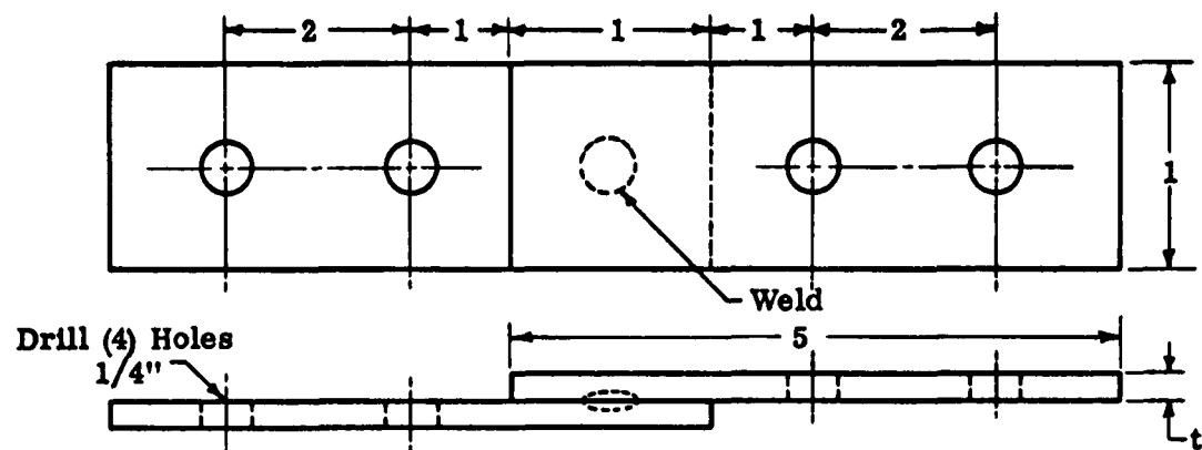
Tensile Shear Fatigue Specimen
