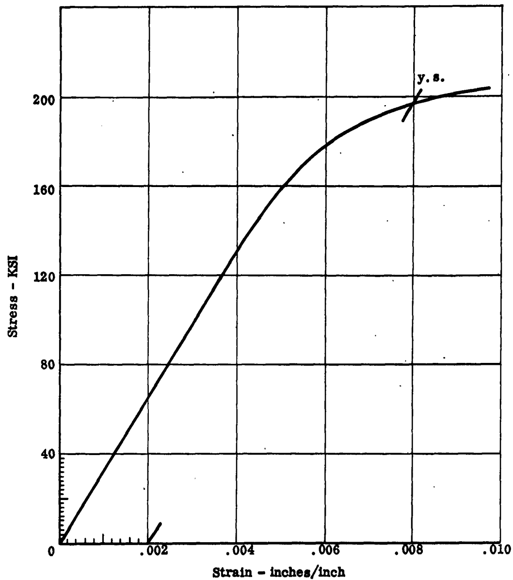
Stress vs Strain Specimen 7A Room Temperature - No Exposure
