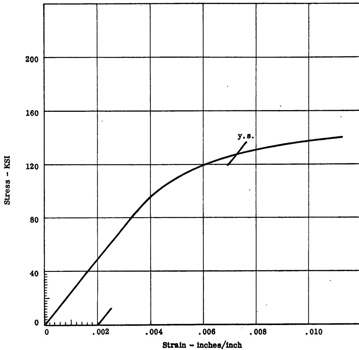
Stress vs Strain Specimen 6B At 1000°F - Half Hour Soak
