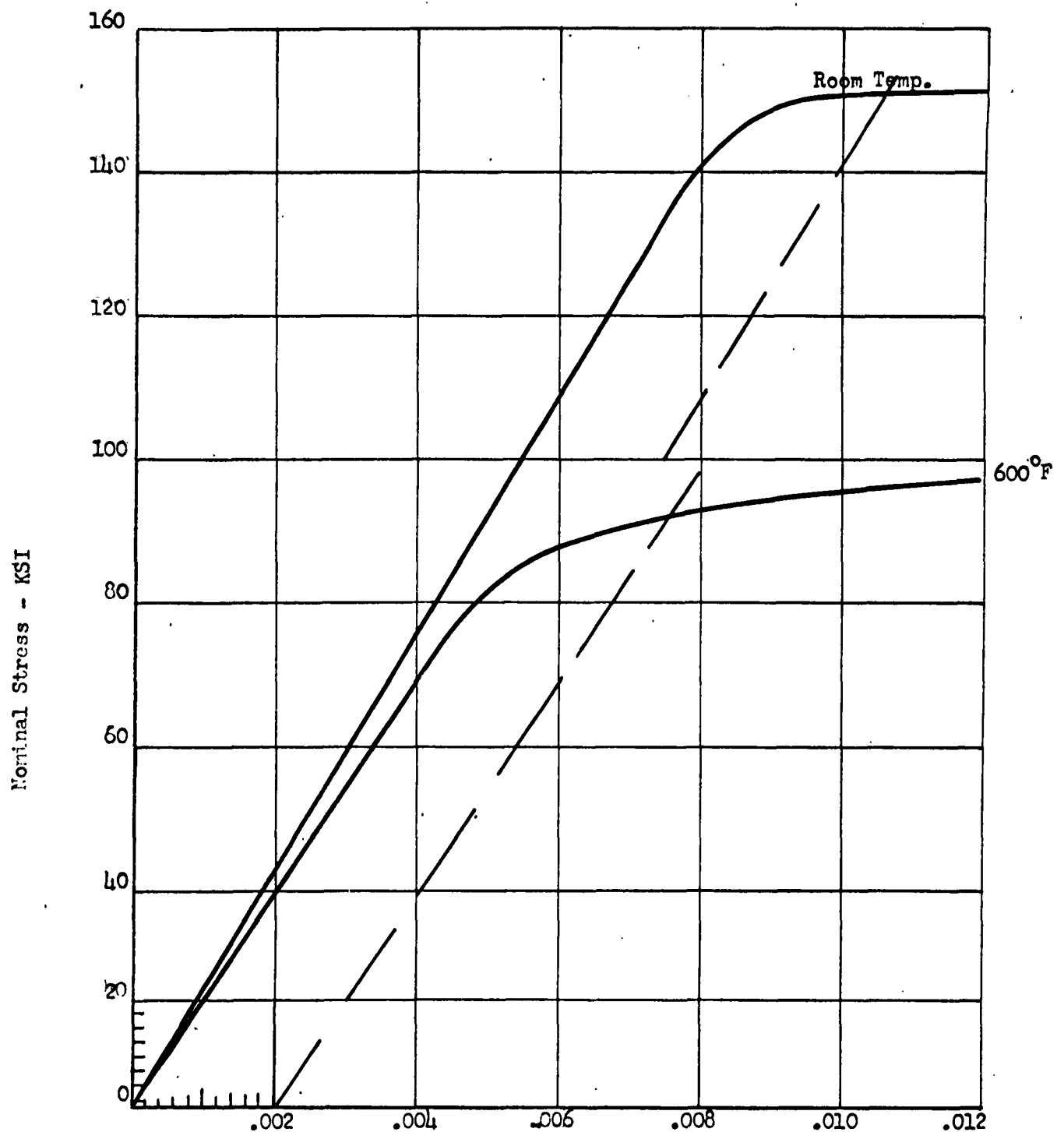
Nominal Strain - In./In. Typical Stress-Strain Curves for Short Transverse Specimens at Room Temperature and 600°F Billet 51009
