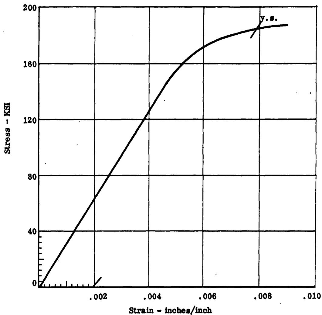
Stress vs Strain Specimen 5B Room Temperature - After 100 Hours at 1000°F
