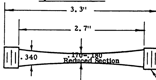
Specimen - "B"
