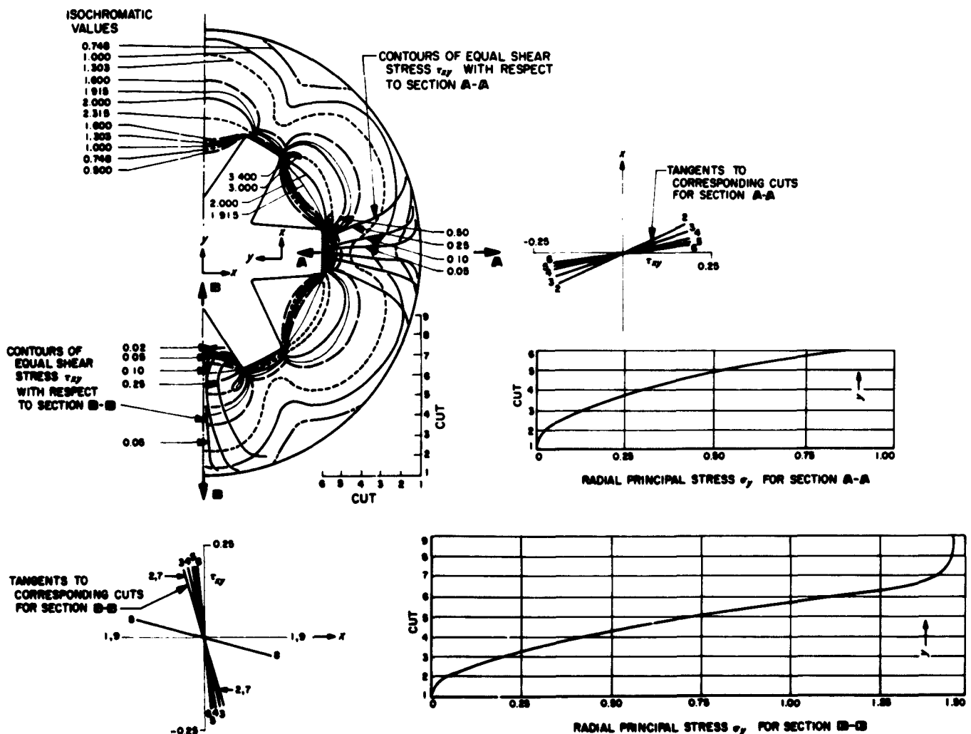
Fig. 4. Typical graphical data reduction to separate principal stresses in coating for free star grain, 60 psi
