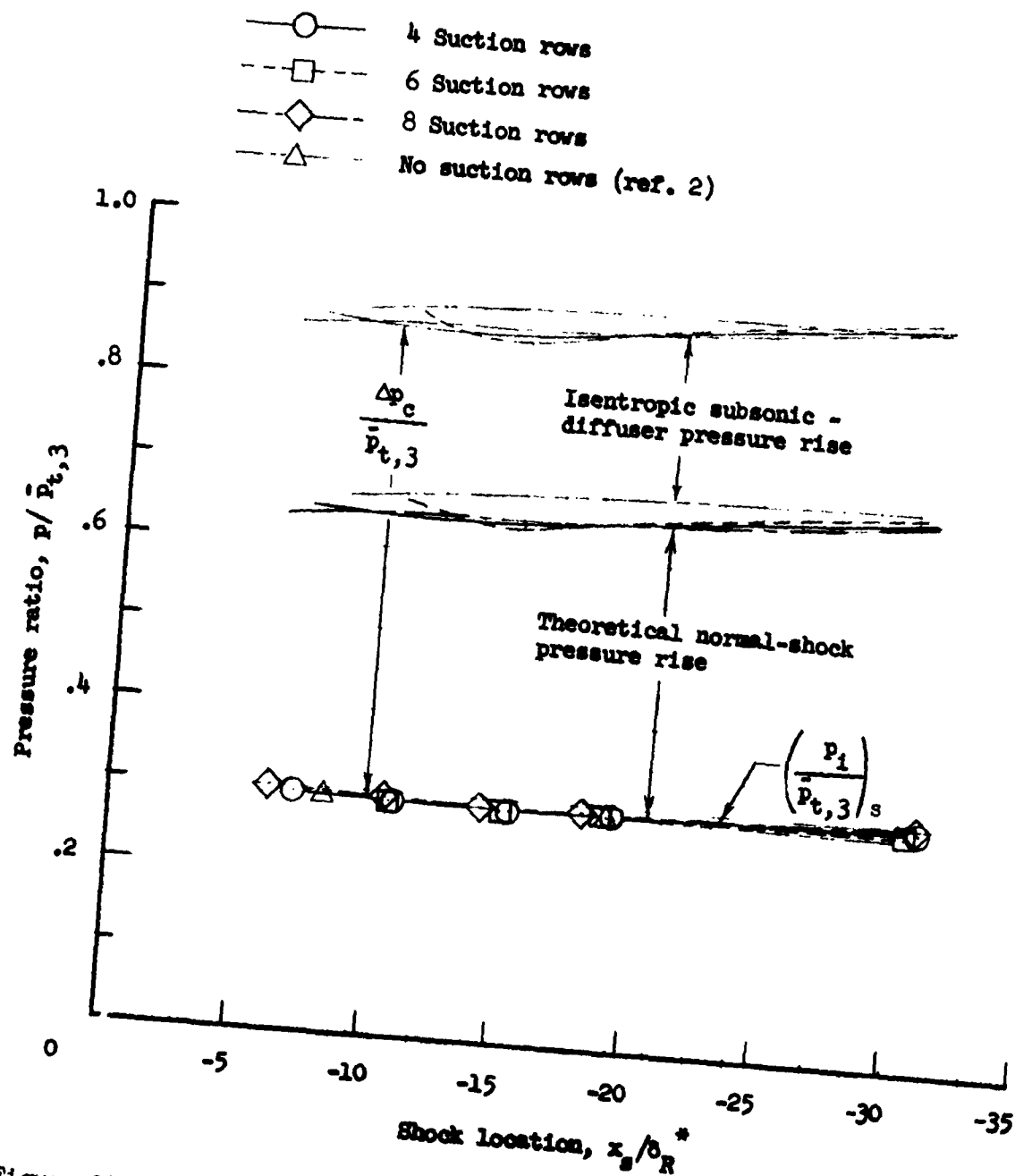
Figure 15.- Theoretical diffuser static-pressure rise due to normal shock and isentropic diffusion; total suction flow of approximately 7 percent.
