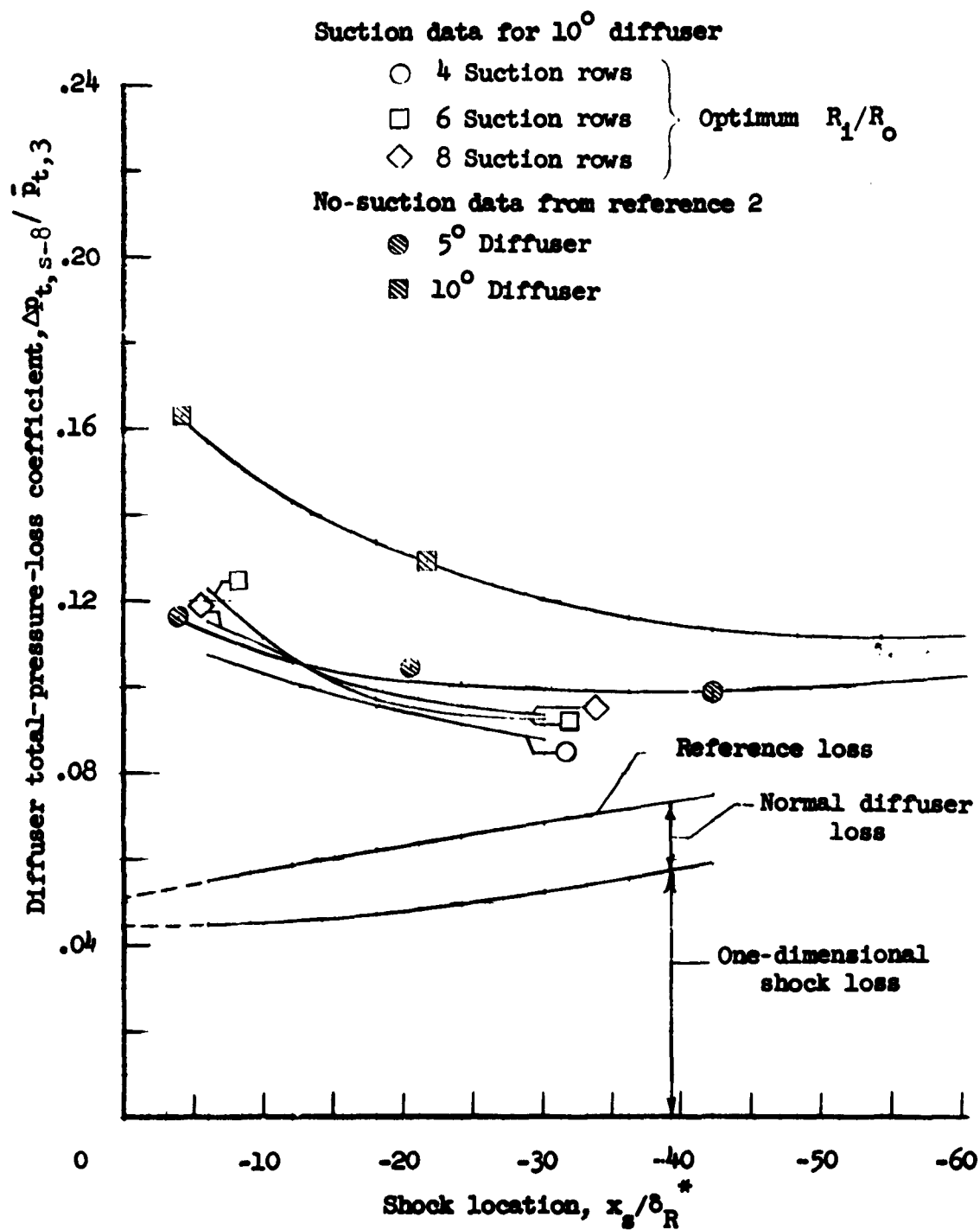
Figure 13.- Minimum diffuser total-pressure loss at various shock locations.
