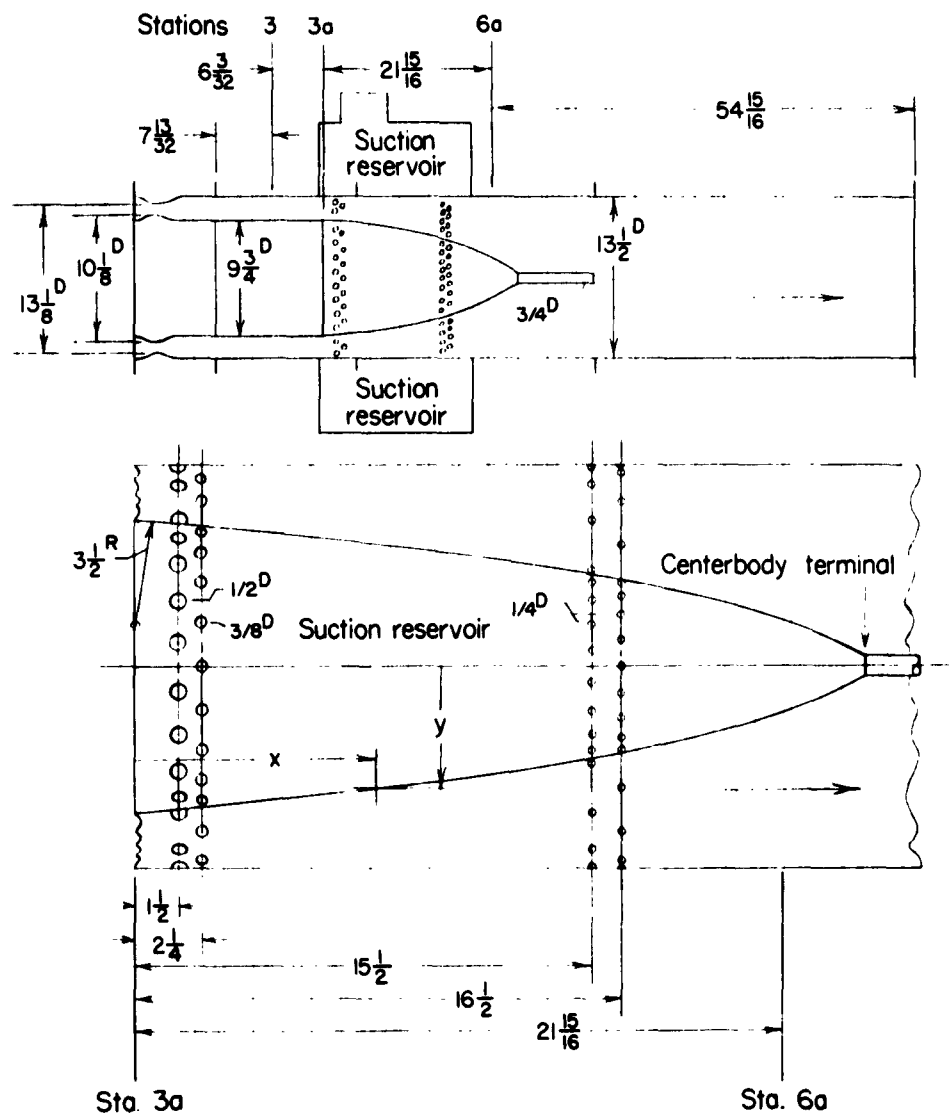
Coordinates for 10° diffuser
