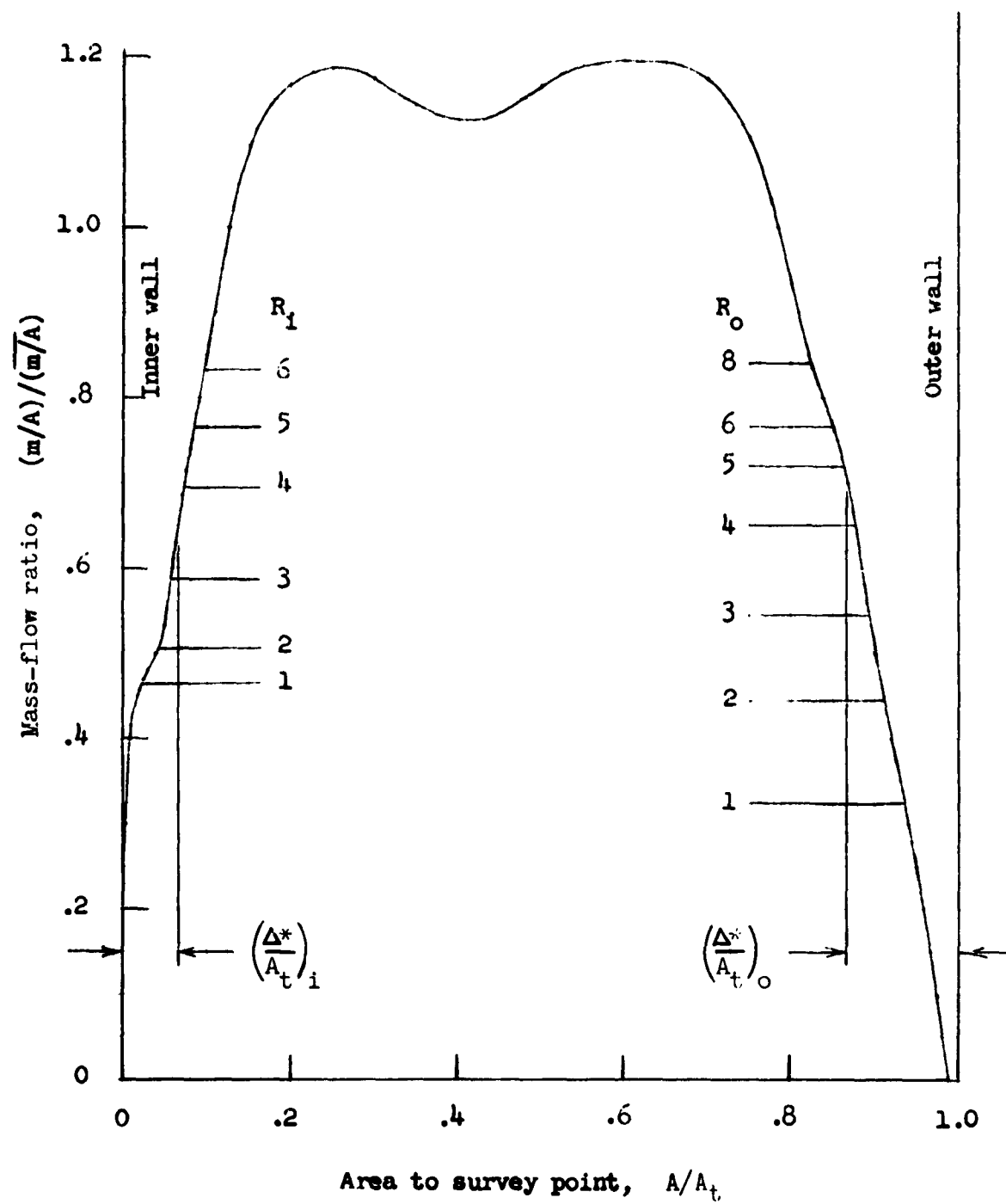
(b) Mass-flow distribution for a shock location x_s/D_0 of -0.185.
