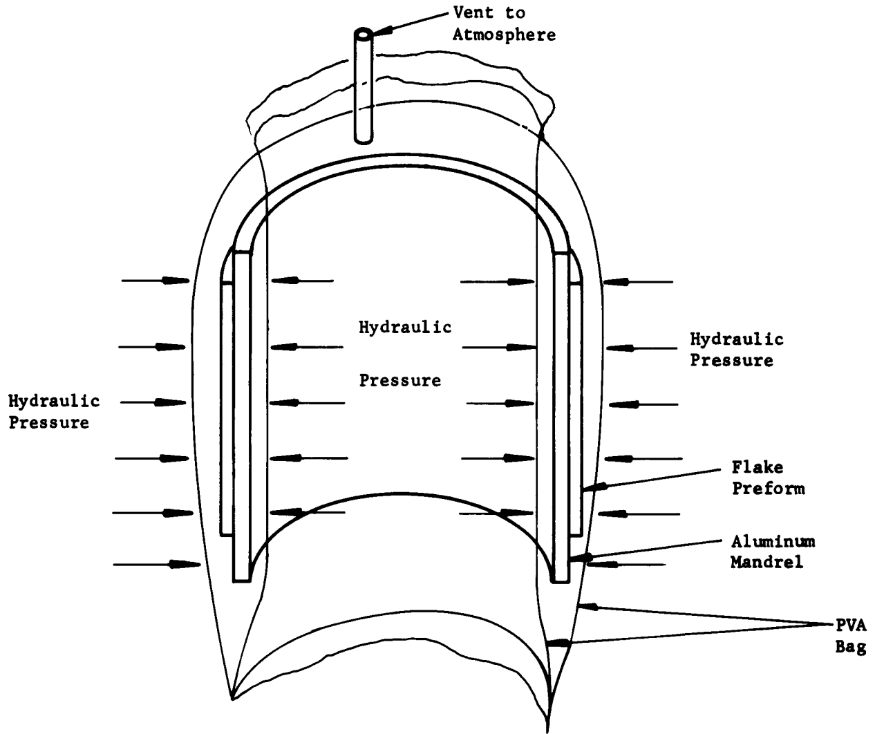
Figure 14. Hydroclave Assembly
