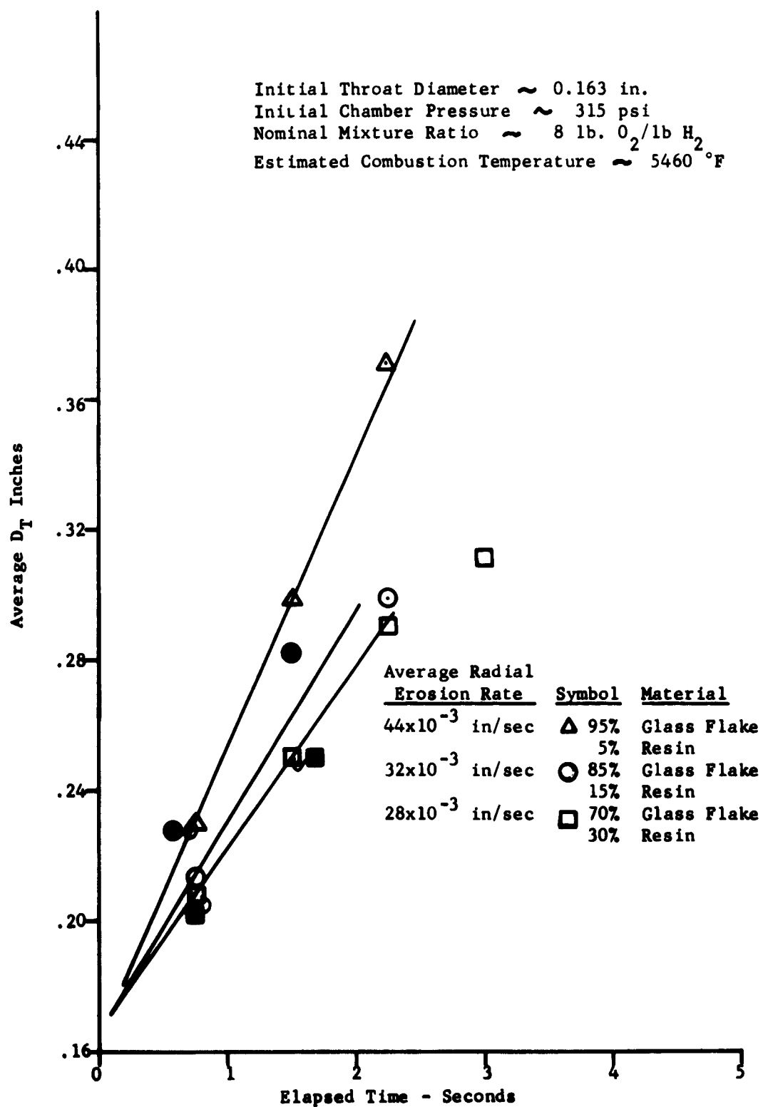
Figure 23. H_2 - O_2 Rocket Nozzle Tests, Throat Diameter Erosion
