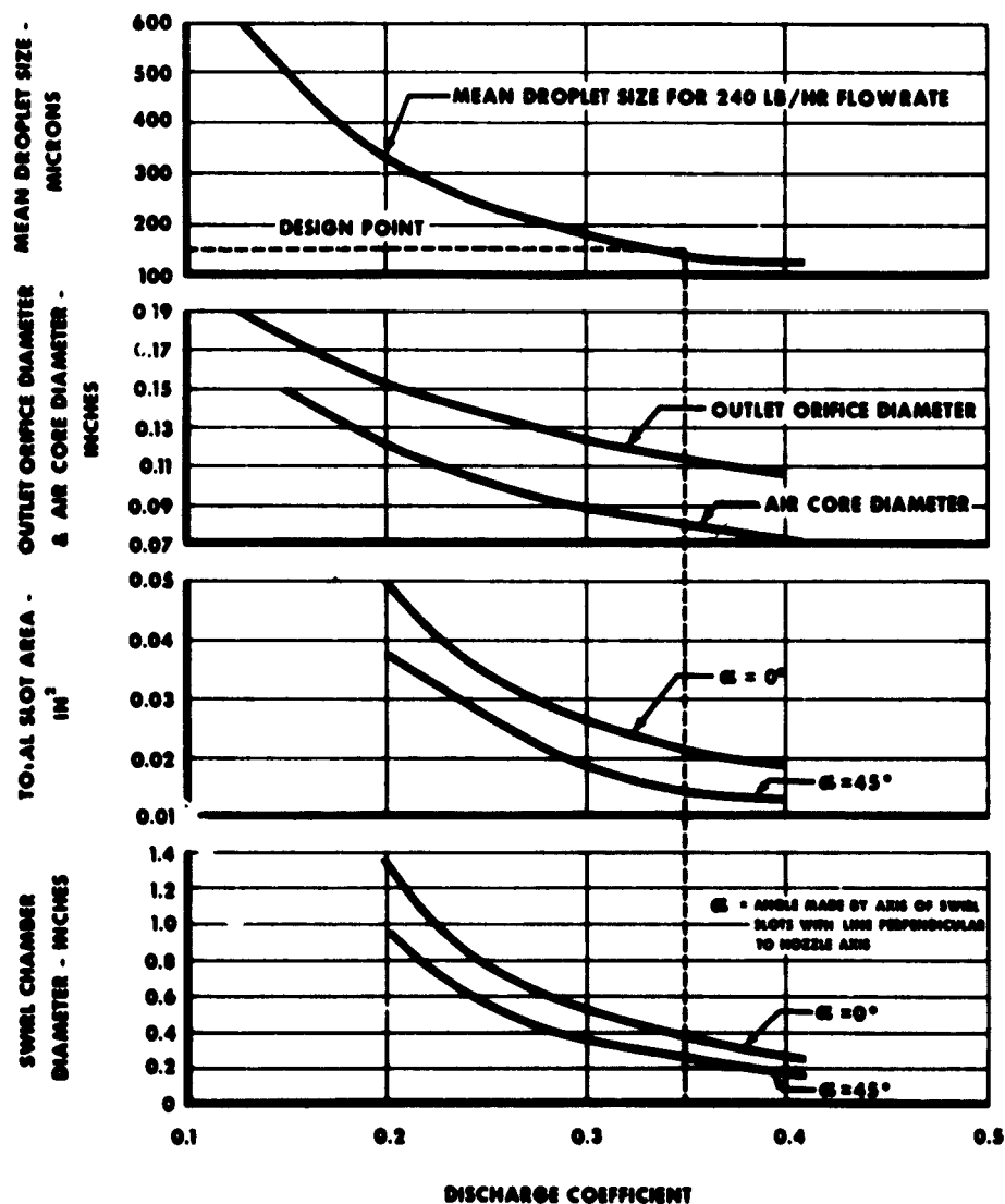
Figure 89 Design Curves for Secondary Orifice of the Dual Orifice Nozzle FD 3522
