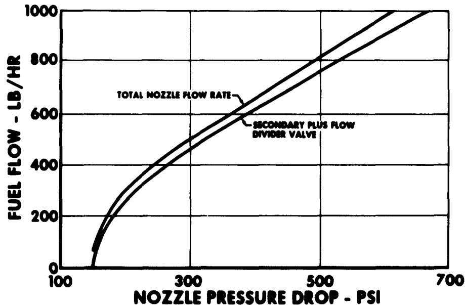
Figure 91 Flow Schedule, Dual Orifice Nozzle
