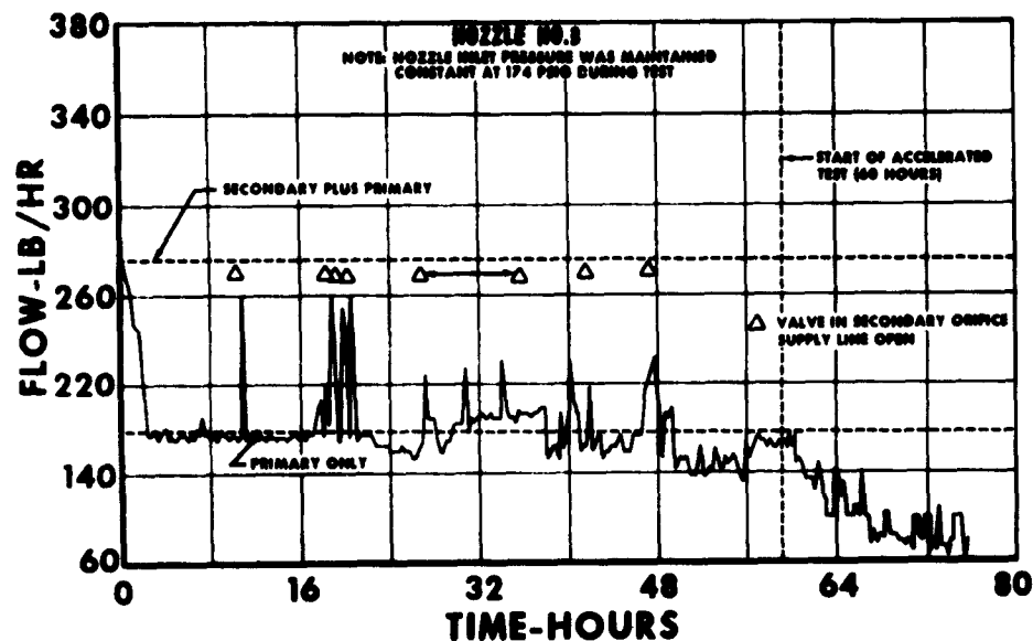
Figure 30 Fuel Flow Variation, Dual Orifice Nozzle (Nozzle No. 3)
