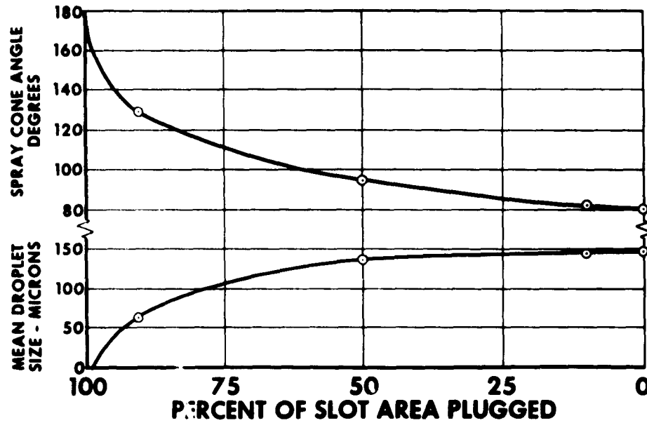
Figure 3 Effect of Plugged Swirl Slots on Spray Angle and Droplet Size FD 3499
