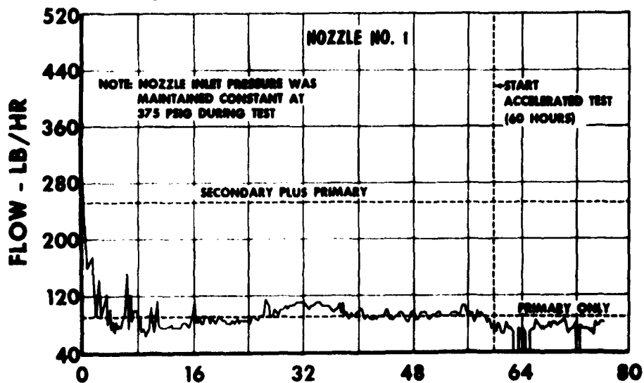
Figure 22 Fuel Flow Variation, Dual Orifice Nozzle with Integral Flow Divider (Nozzle No. 1) FD 3537
