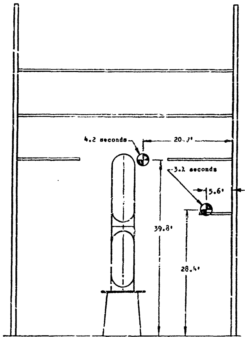
Approximate Center Locations of Vapor Explosions At 3.1 and 4.2 Seconds After Destruct Initiation (Measurements are in one plane only)
