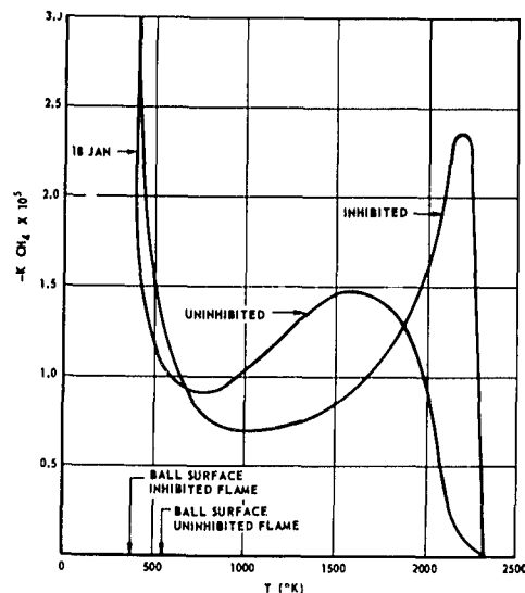
Figure III-3 THE EFFECT OF \text{HBr} ON THE RATE OF METHANE DISAPPEARANCE IN A STOICHIOMETRIC FLAME ( \text{CH}_4 - 0.09 \text{O}_2 0.179 \text{Ar} - 0.727 ; P = 0.05 atm.). K_{\text{CH}_4} (MOLES PER CUBIC cm. per sec \times 10^5 ) VERSUS TEMPERATURE ( ^\circ\text{K} ).
