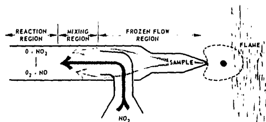
Figure III-5a SCHEMATIC DIAGRAM OF SCAVENGER PROBE USED IN MEASURING OXYGEN-ATOM CONCENTRATIONS
