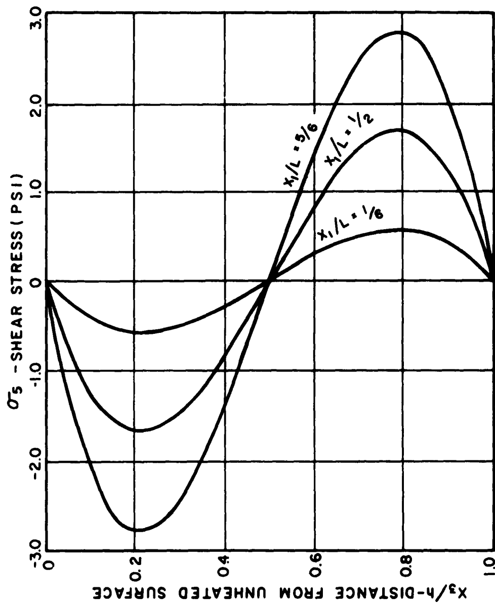
FIG.21 DISTRIBUTION OF \sigma_s THROUGH 1/4 INCH THICK PLATE AFTER 40 SECONDS OF HEATING
