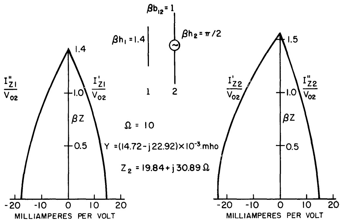
FIG. 10-2 ELEMENT CURRENTS FOR PARASITIC COUPLET WITH \beta h_1 = 1.4 , \beta h_2 = \pi/Z , \beta b = 1 , V_{01} = 0
