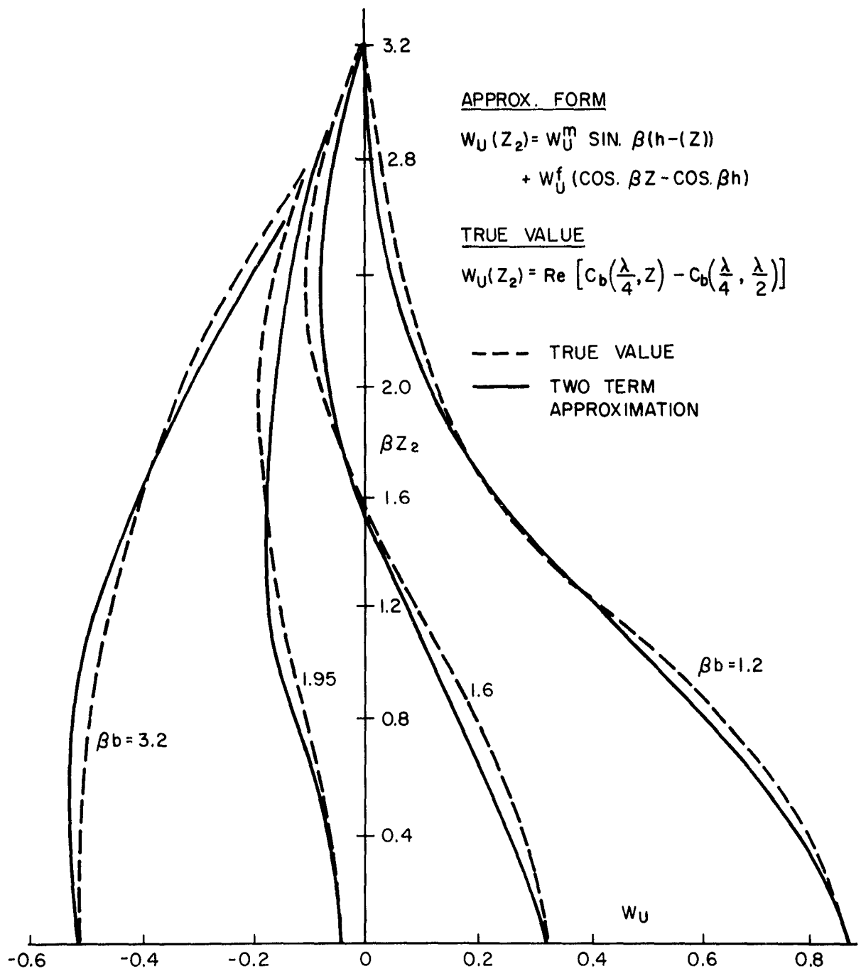
FIG. 8-6 COMPARISON OF TWO TERM APPROXIMATION FOR VECTOR POTENTIAL SHOWN IN FIG. 8-5 WITH TRUE VALUE
