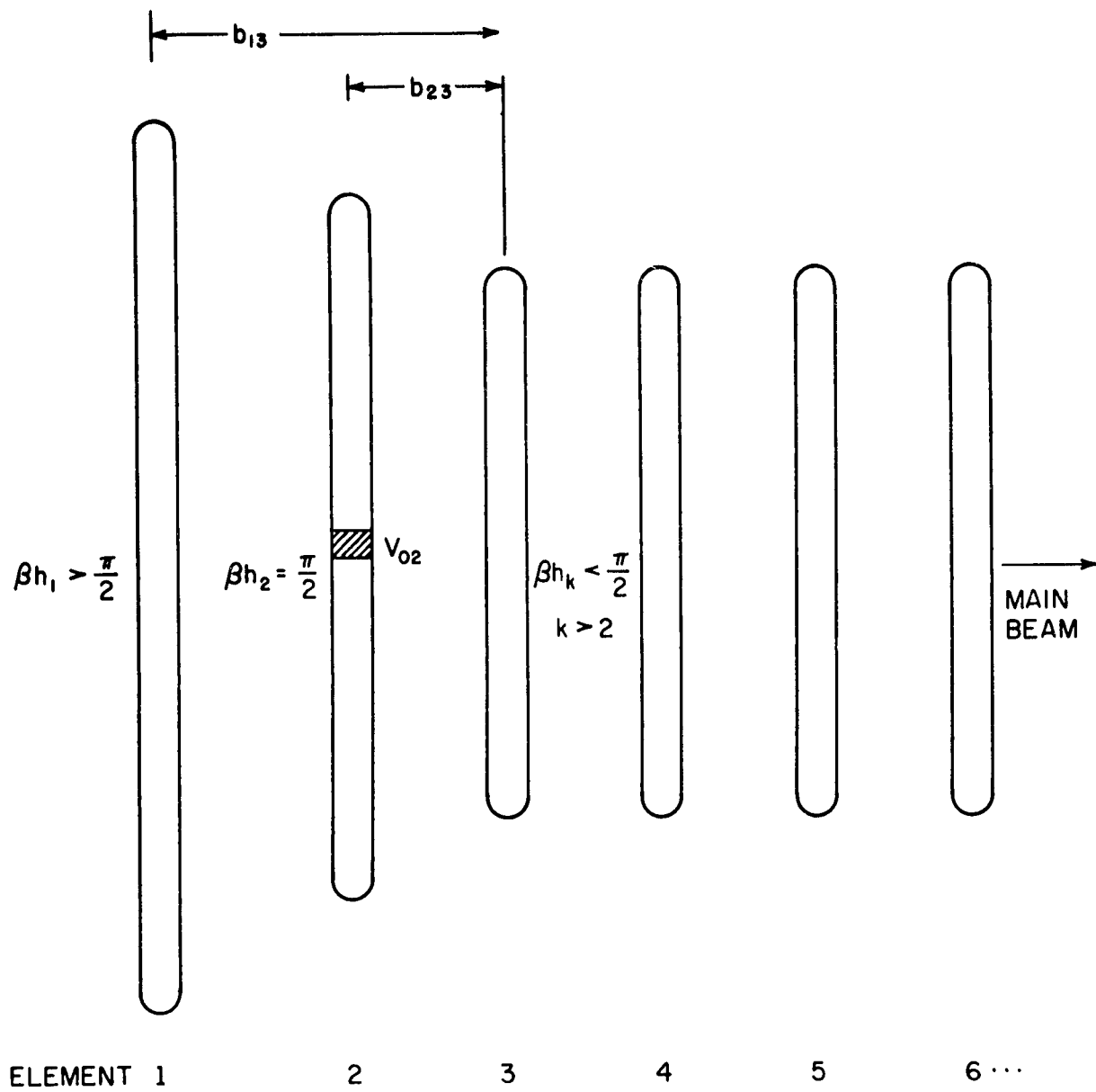
FIG. 11-1 A SIX ELEMENT YAGI ARRAY
