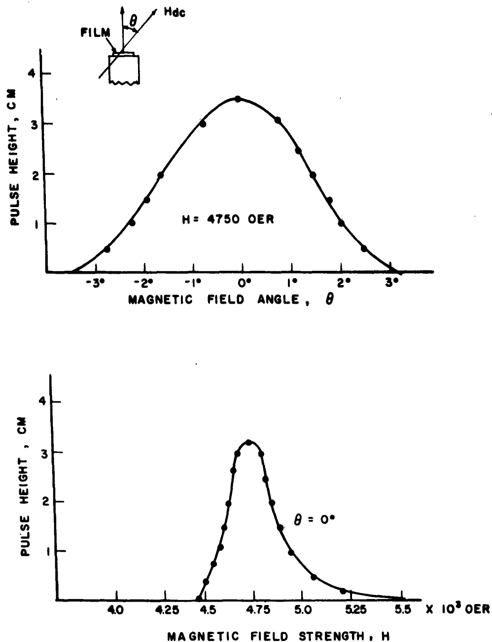
Figure 15. Characteristics of Magnetostrictive Excitation of Transverse Phonons in \langle 111 \rangle Silicon Frequency. 3.15 kMc/s Liquid Helium Temperature. Velocity is 5.08 \times 10^5 cm/sec.
