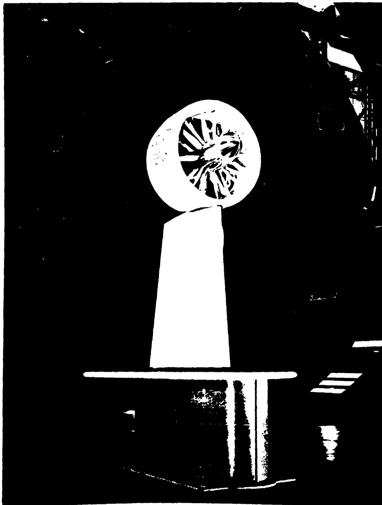
Figure 1.- Ducted fan model mounted in the Ames 40- by 80-Foot Wind Tunnel.
