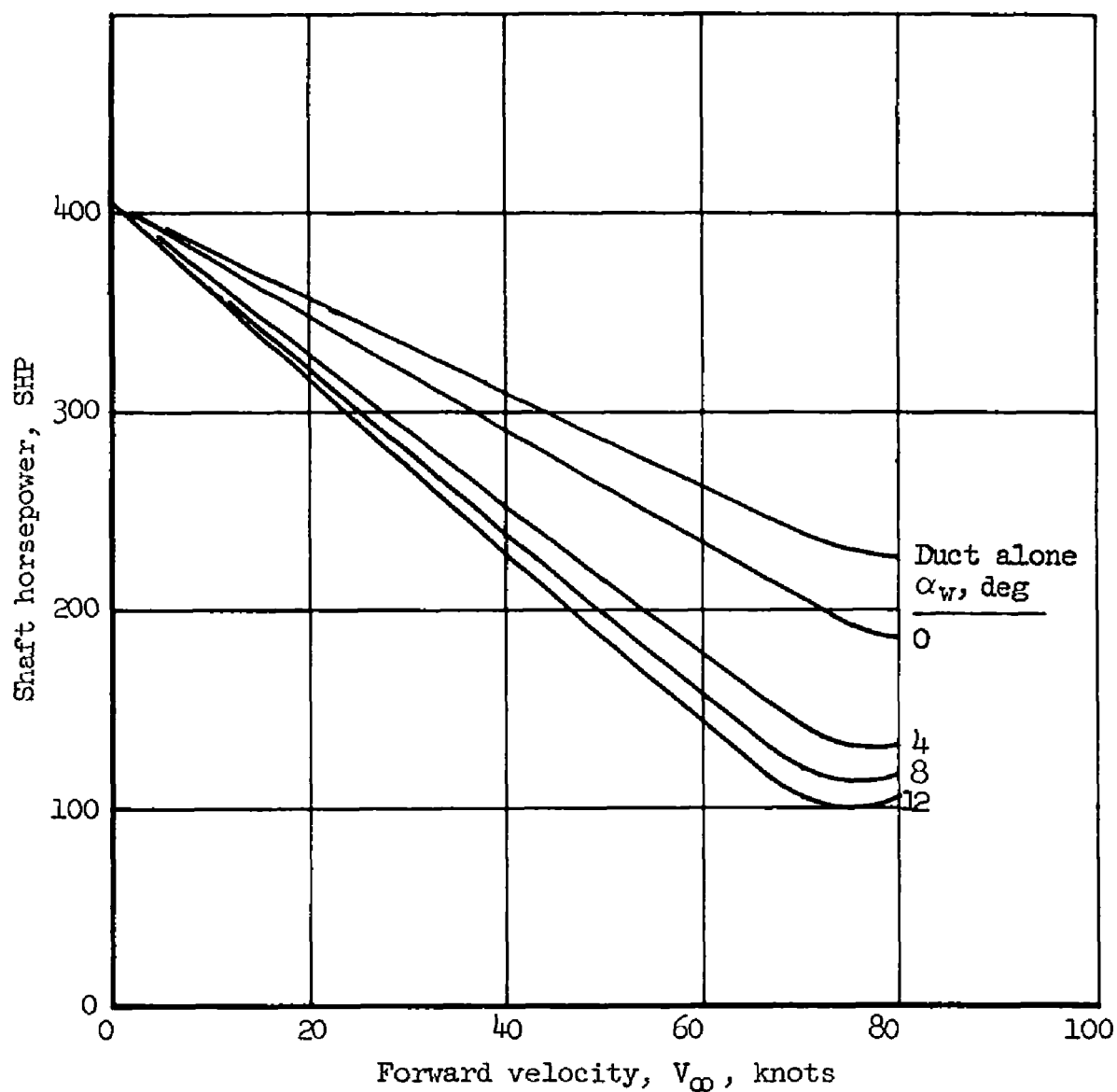
Figure 12.- Effectiveness of the wing in reducing the power required for transition.
