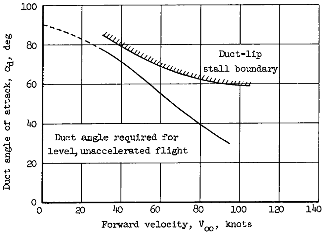
(b) Duct angle of attack as a function of forward velocity.
