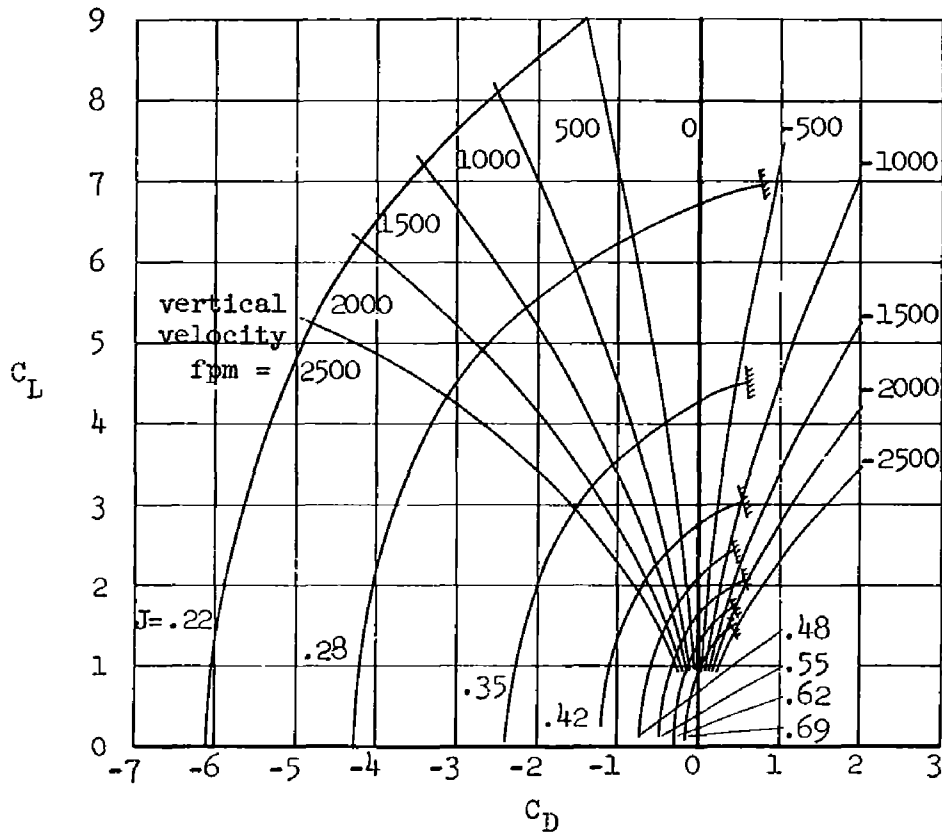
(a) Curves of constant vertical velocity superimposed upon the wing-duct aerodynamic characteristics at \alpha_w = 0^\circ .
