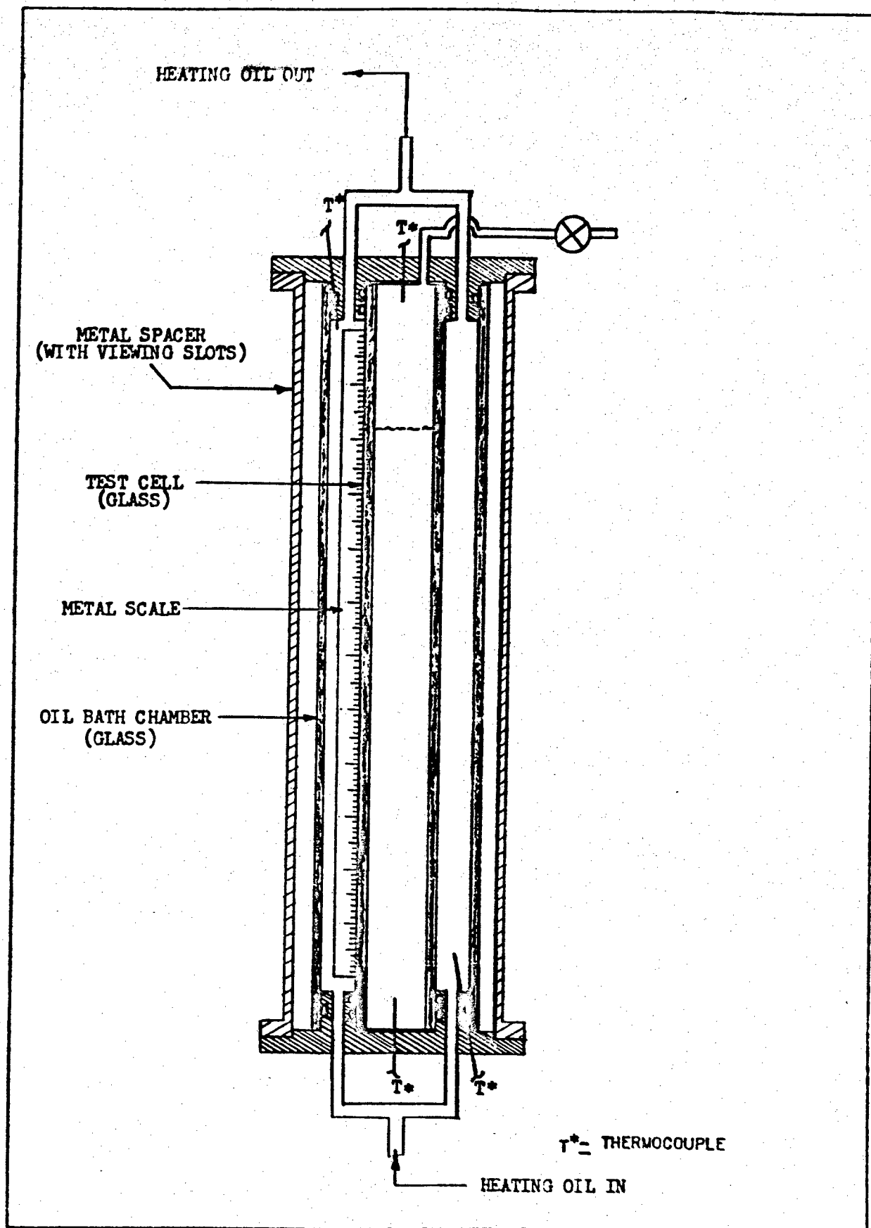
Figure 65 - Specific Volume Apparatus
