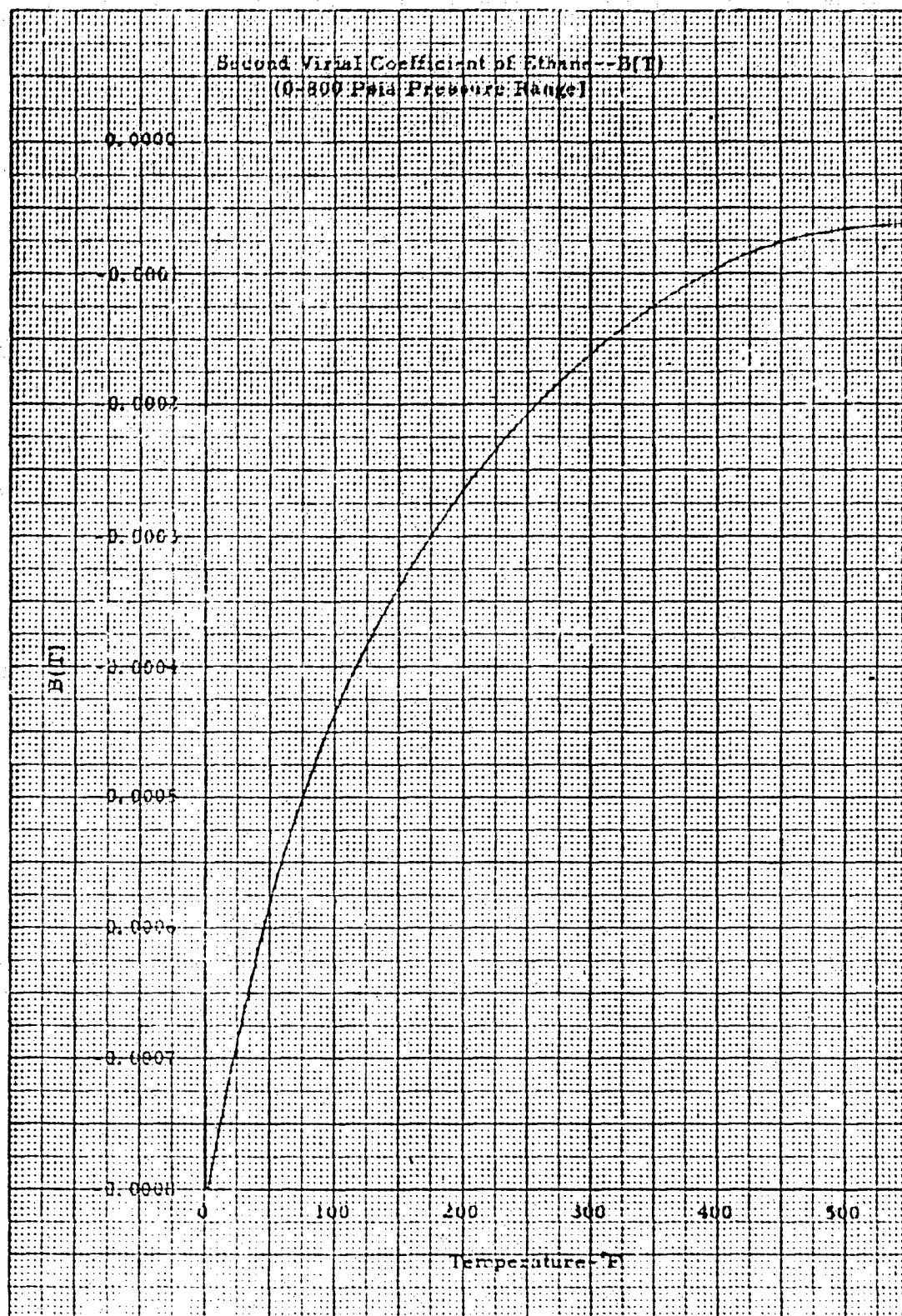
Figure No. 7 - Second Virial Coefficient of Ethane
