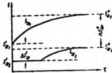
Fig. 88. Variation in temperature t_{w1} and t_{w2} of plane wall with time
