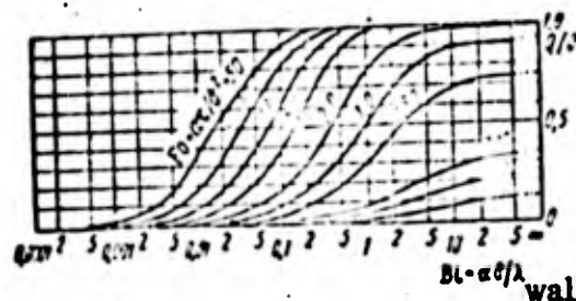
Fig. 96. \frac{Q}{Q_0 - Q_f} = f(Bi, Fo) as function of plane infinite wall
