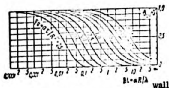
Fig. 97. \frac{\theta_w}{\theta'} = f(Bi, Fo) as function of infinitely long cylinder
