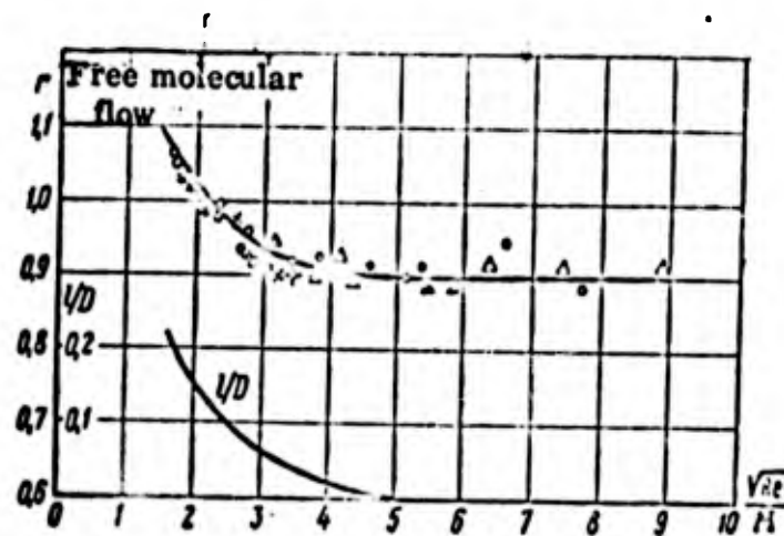
Fig. 213. Temperature recovery coefficient on sphere
