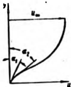
Fig. 150. Shape of velocity profile in sweat cooling
