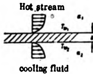
Fig. 144. Convective Cooling
