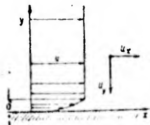
Fig. 38. Concept of boundary layer
