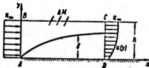
Fig. 115. Derivation of integral relationship of momentum on plate
