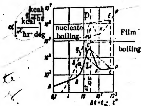
Fig. 46. Nature of variations in heat flux and heat-transfer coefficient for boiling water as function of temperature head ( p=1 \text{ atm} )
