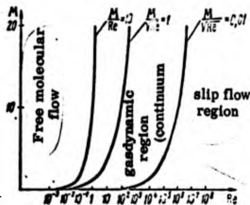
Fig. 212. Flow regions
