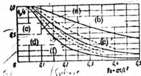
Fig. 103. Curves showing \frac{Q}{Q_\infty} = f(Fo) for bodies of different shapes at Bi = \text{const.}
