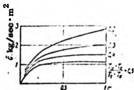
Fig. 195. Variation in specific coolant consumption in barrier cooling
