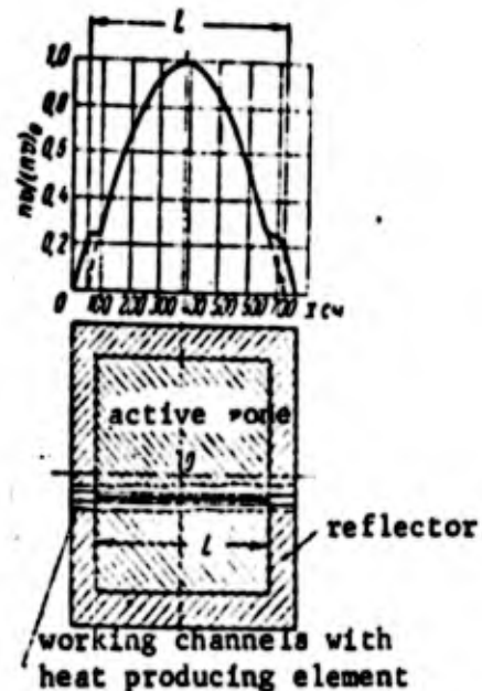
Fig. 249. Distribution of thermal neutron flux along length of uranium graphite power reactor with reflector
