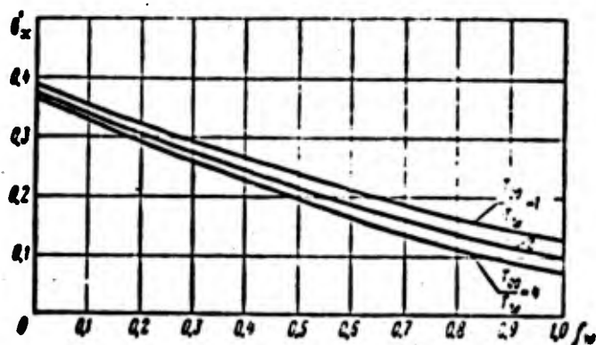
Fig. 161. Variation in \Theta'_x in sweat cooling in neighborhood of leading critical point on axially-symmetric body
