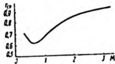
Fig. 119. Variation in mean temperature recovery coefficient of cylinder as function of M
