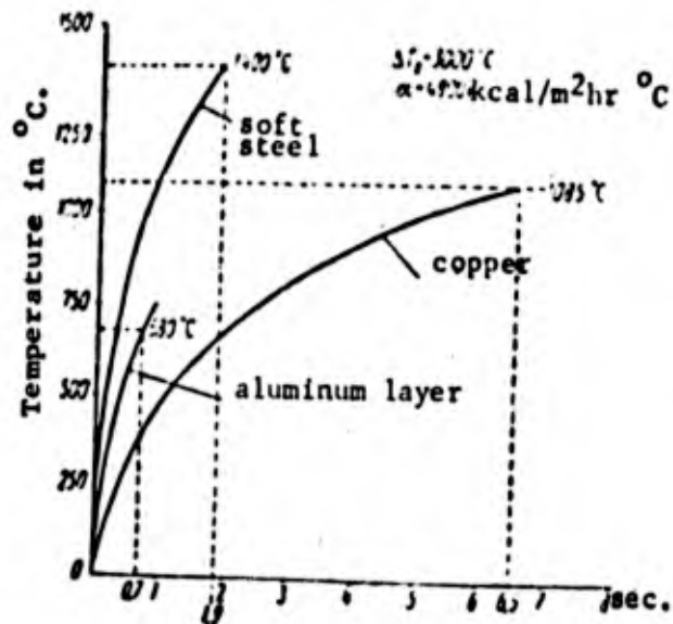
Fig. 227. Variation in thick wall temperature with time for different materials
