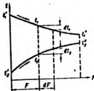
Fig. 81. Distribution of temperature in co-flowing heat exchanger
