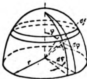
Fig. 72. Determining spatial angle in spherical coordinates
