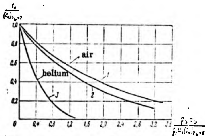
Fig. 177. Variation in heat-exchange coefficients in sweat cooling on plates with turbulent boundary layer
