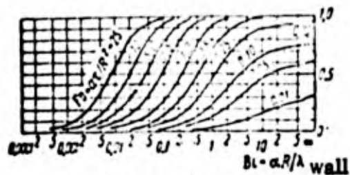
Fig. 102. \frac{Q}{Q_\infty} = f(Fo, Bi) as function of sphere
