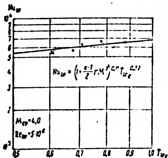
Fig. 134. Effect of temperature factor \bar{T}_w = T_w/T_c on heat exchange
