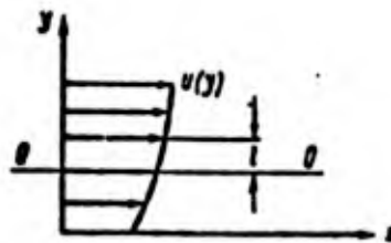
Fig. 211. Concept of free path length of molecule
