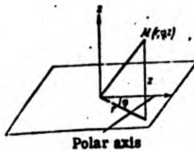
Fig. 18. Diagram of cylindrical coordinates of points
