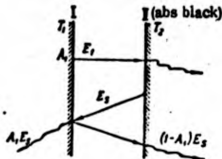
Fig. 69. Derivation of Kirchhoff's law
