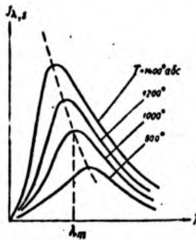
Fig. 67. Energy distribution of black radiation over spectrum
