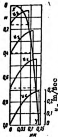
Fig. 57. Variation in film thickness and velocity distribution in film of condensate
