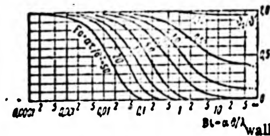
Fig. 95. \frac{\theta_0}{t_0 - t_f} = f(Bi, Fo) as function of plane infinite wall
