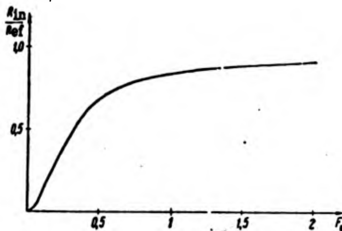
Fig. 224. Dependence \frac{R_{in}}{(R_{in})_{ef}} from Fo = \frac{q_{in} \tau}{\lambda_{in}} .
