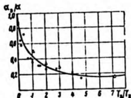
Fig. 60. Relative variation in heat-transfer coefficient during condensation as function of air content in vapor
