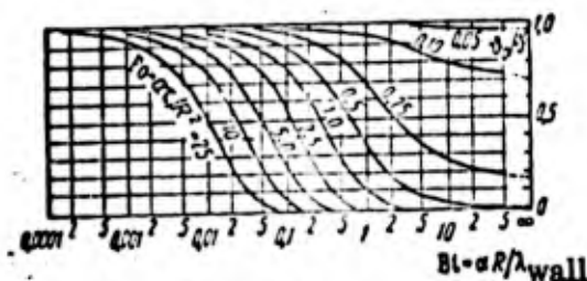
Fig. 101. \frac{Q}{Q'} = f(Bi, Fo) as function of sphere
