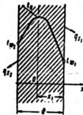
Fig. 253. Temperature distribution in plate during volume heat release q_{s1} + q_{s2} (showing derivation of equation).
