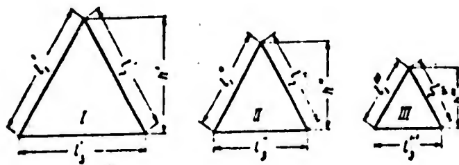
Fig. 36. Geometrically similar triangles
