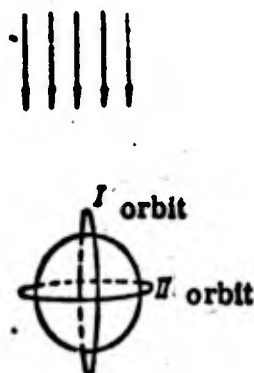
Fig. 245. Position of two extreme orbits
