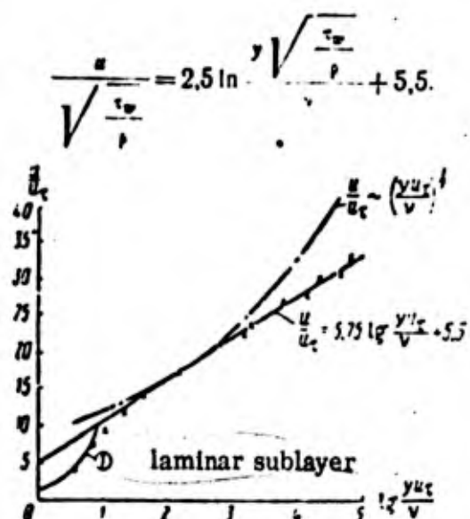
Fig. 131. Velocity distribution in dimensionless coordinates
