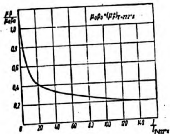
Fig. 142. Variation in \mu_0/\mu as function of enthalpy
