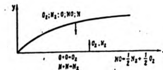
Fig.143. The case of chemical nonequilibrium in the boundary layer
