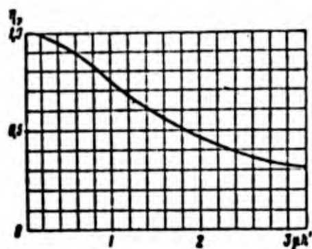
Fig. 35. Efficiency of fin \eta_f = f(J\beta h') .
