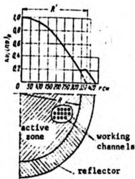
Fig. 248. Distribution of thermal neutron flux along radius of uranium graphite power reactor with reflector
