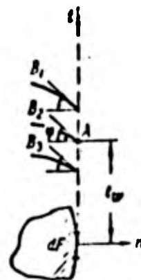
Fig. 91. Graphic representation of boundary condition of second kind
