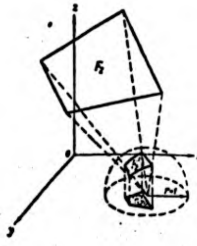
Fig. 77. Graphic determination of angular coefficient
