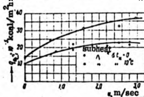
Fig. 53. Effect of fluid velocity on first critical thermal load (water p \approx 1 atm abs)
