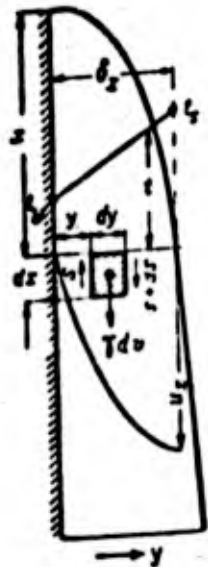
Fig. 56. Film condensation on vertical wall
