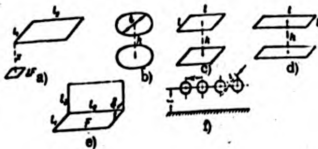
Fig. 78. Systems of radiant heat exchange
