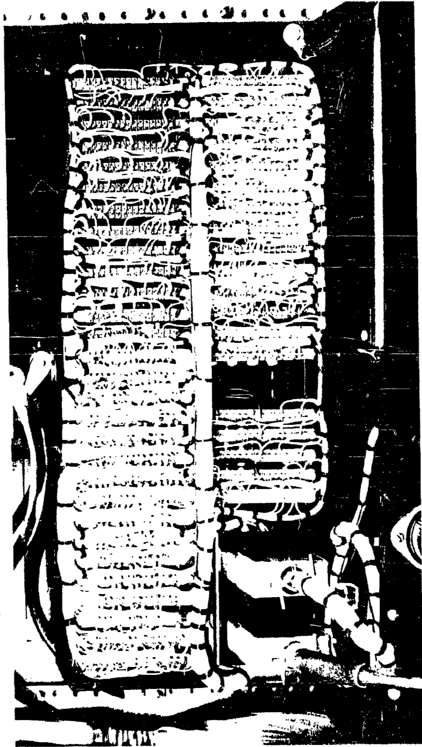
Fig. 7. Wind Data Acquisition System. Rear view, showing analog to digital converter
