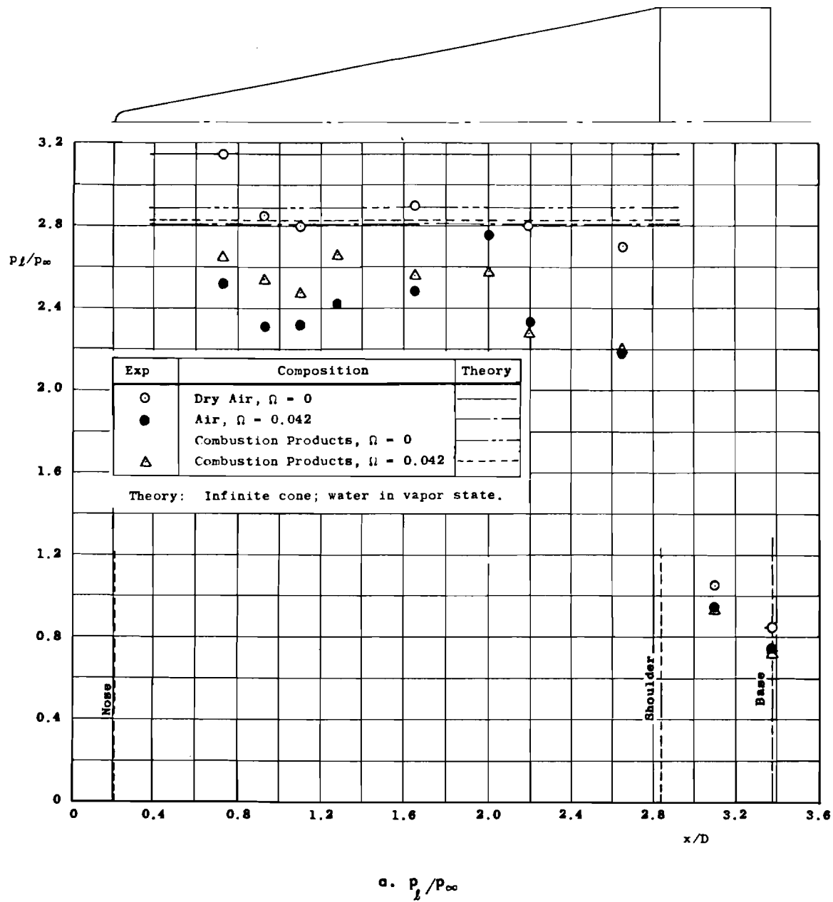
Fig. 6 Pressure Distribution on a 10-deg Half-Angle Blunted Cone, \alpha = 0 deg
